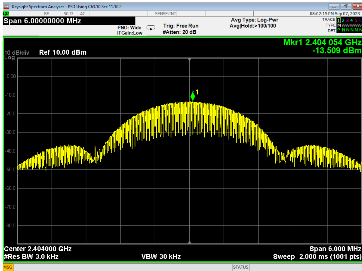
33 PSD, Low Channel, GMSK 2MB
