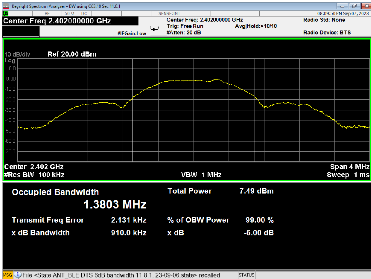
04 6dB Bandwidth, Low Channel, GFSK
