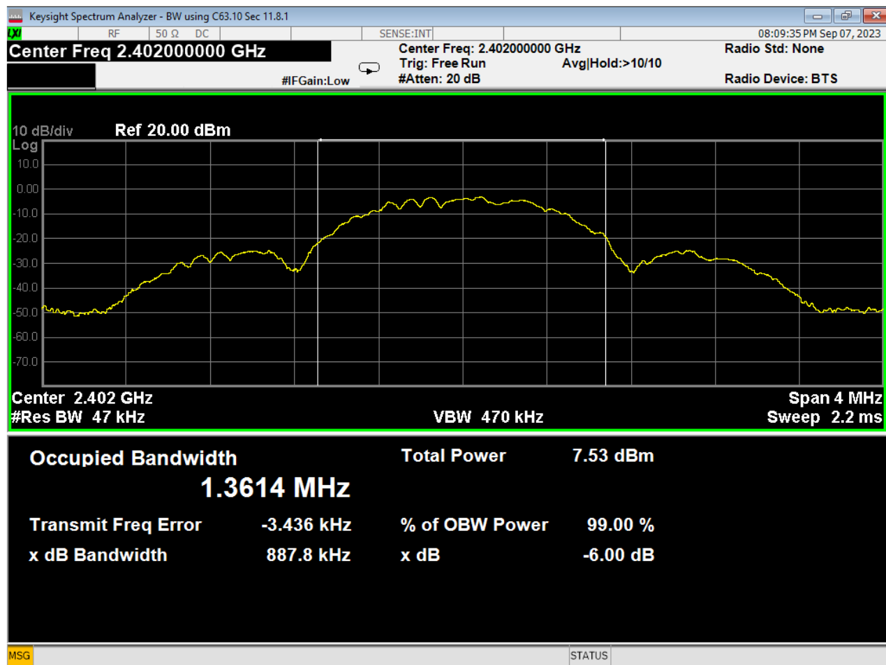
40 Occupied Bandwidth, Low Channel, GFSK
