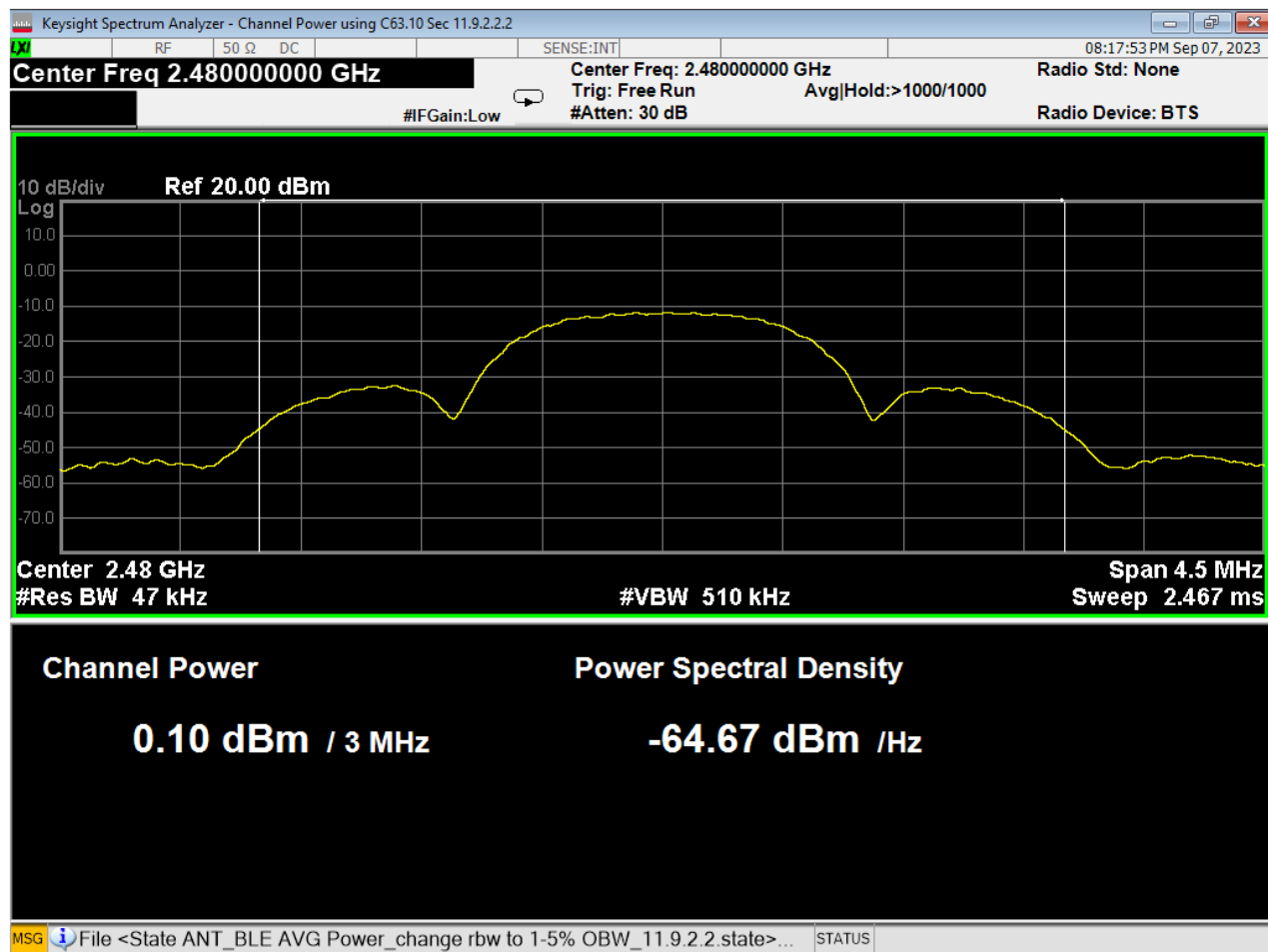
03 Average Power, High Channel, GFSK
