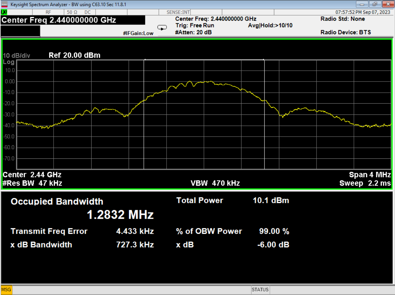
44 Occupied Bandwidth, Mid Channel, GMSK 1MB
