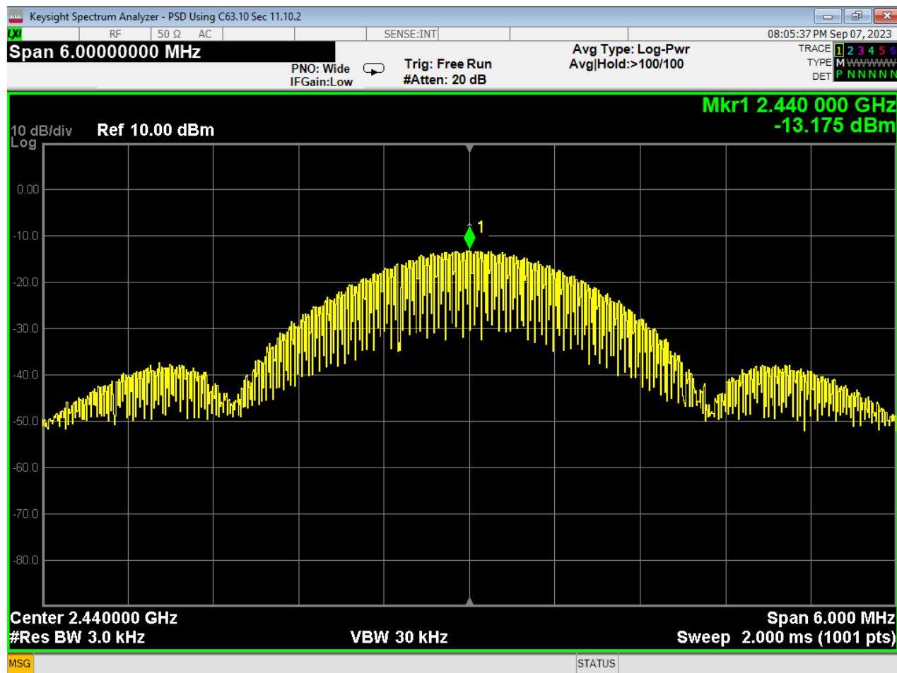
34 PSD, Mid Channel, GMSK 2MB
