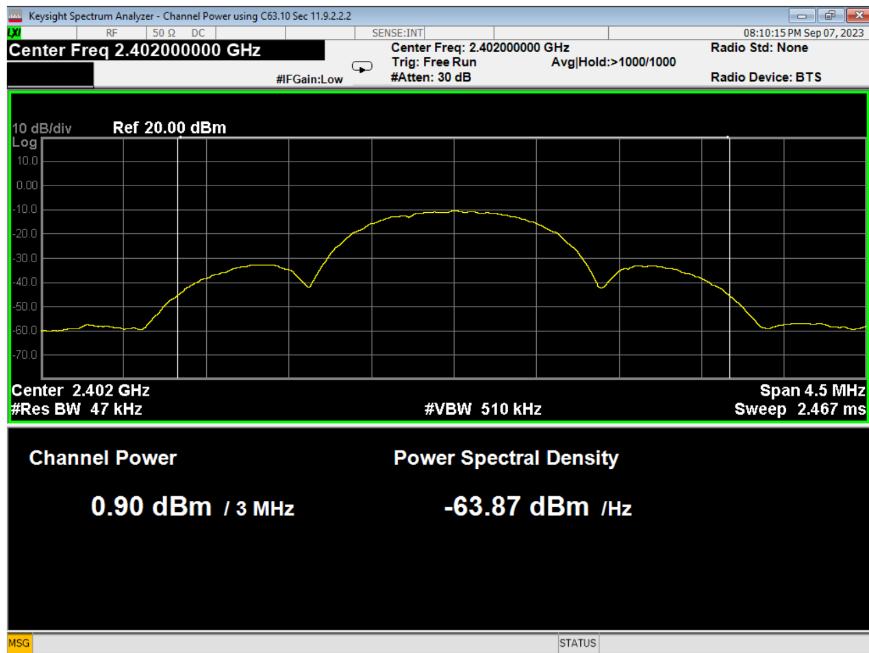
01 Average Power, Low Channel, GFSK
