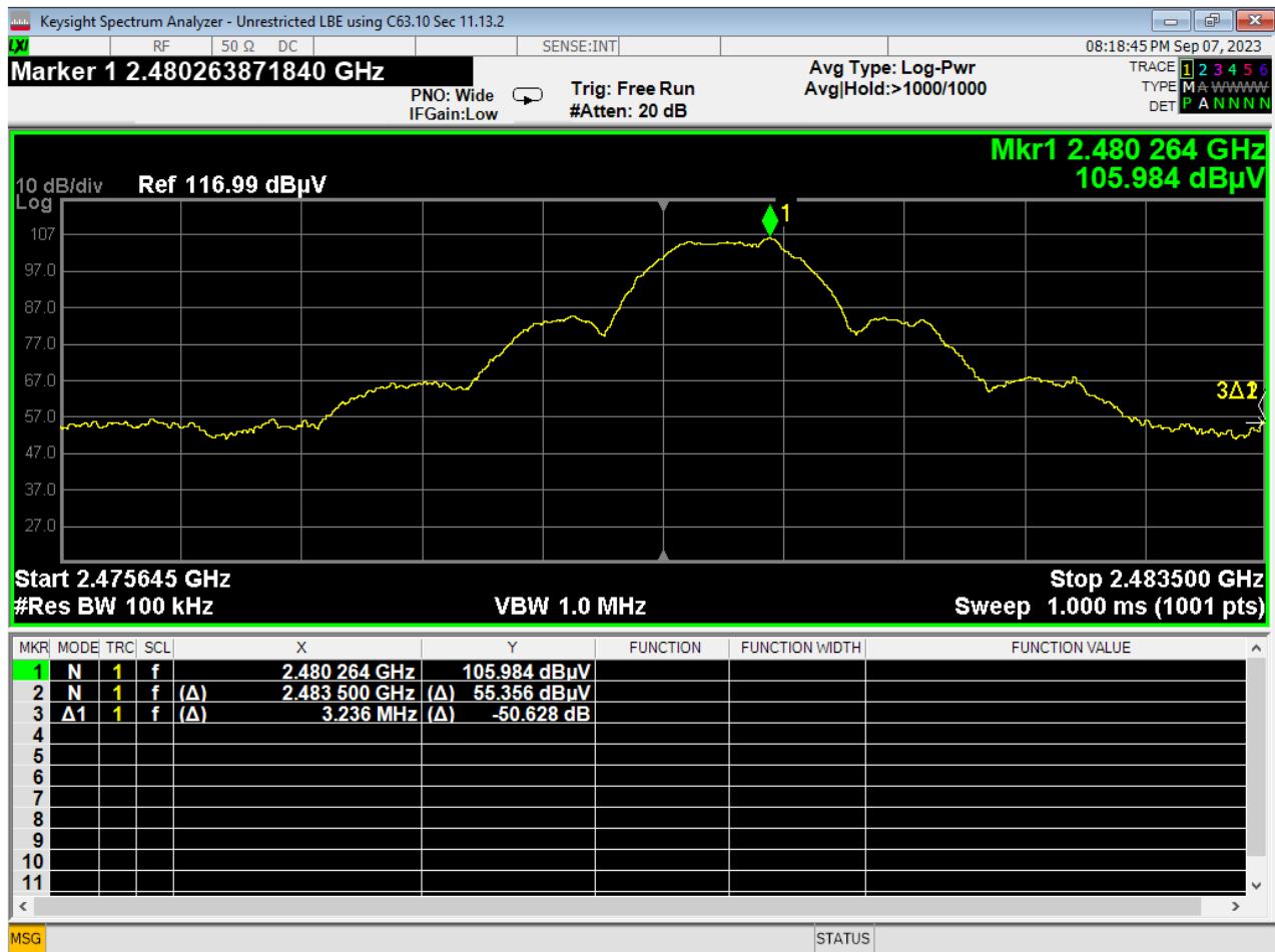
11 Higher Bandedge, Unrestricted, GFSK
