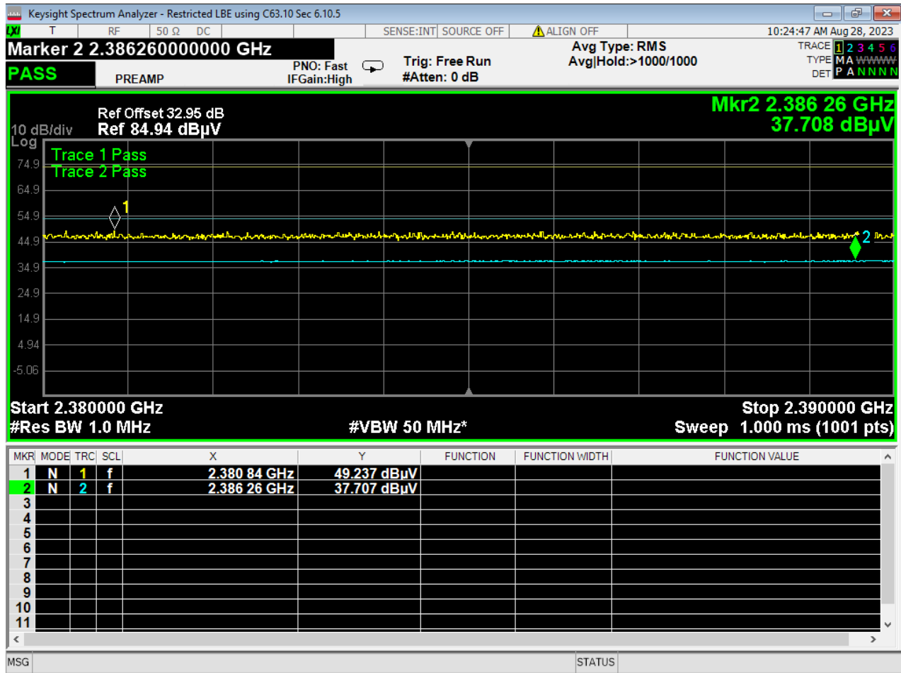
12 Lower Bandedge, Restricted, GFSK
