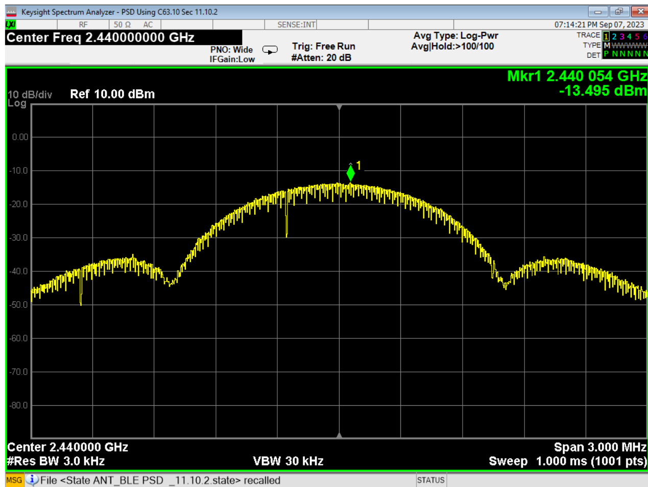
21 PSD, Mid Channel, GMSK 1MB
