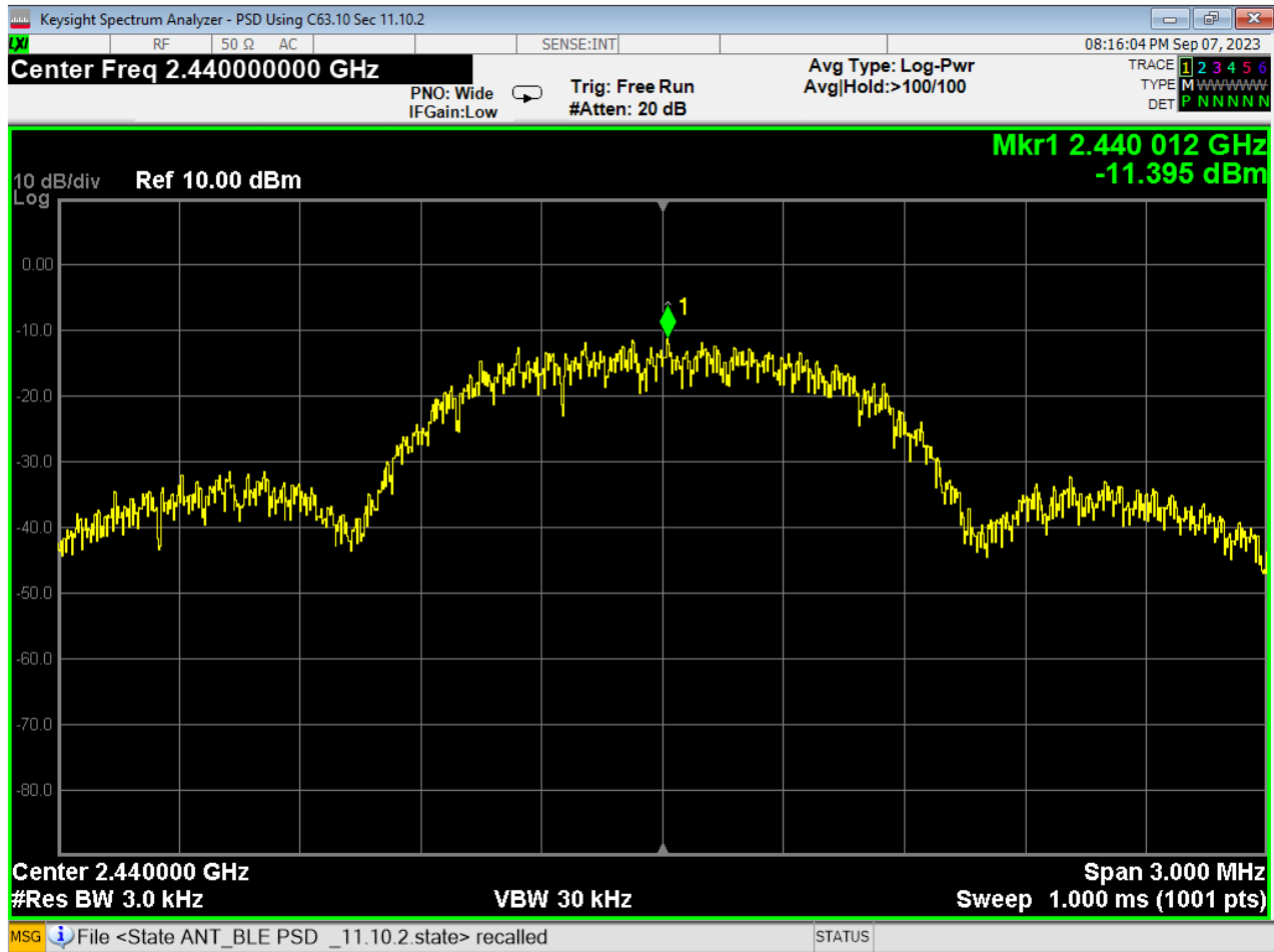
08 PSD, Mid Channel, GFSK
