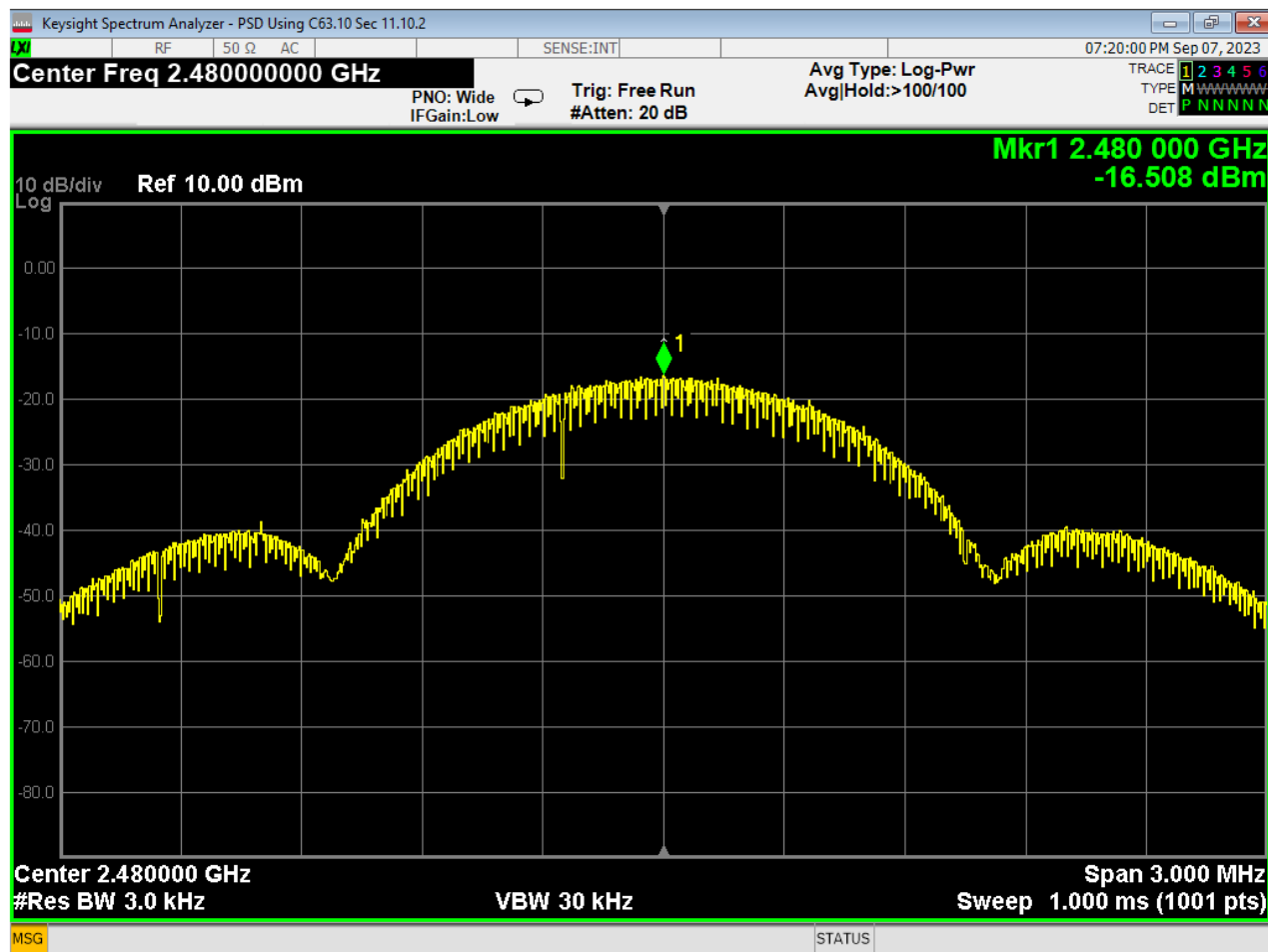
22 PSD, High Channel, GMSK 1MB
