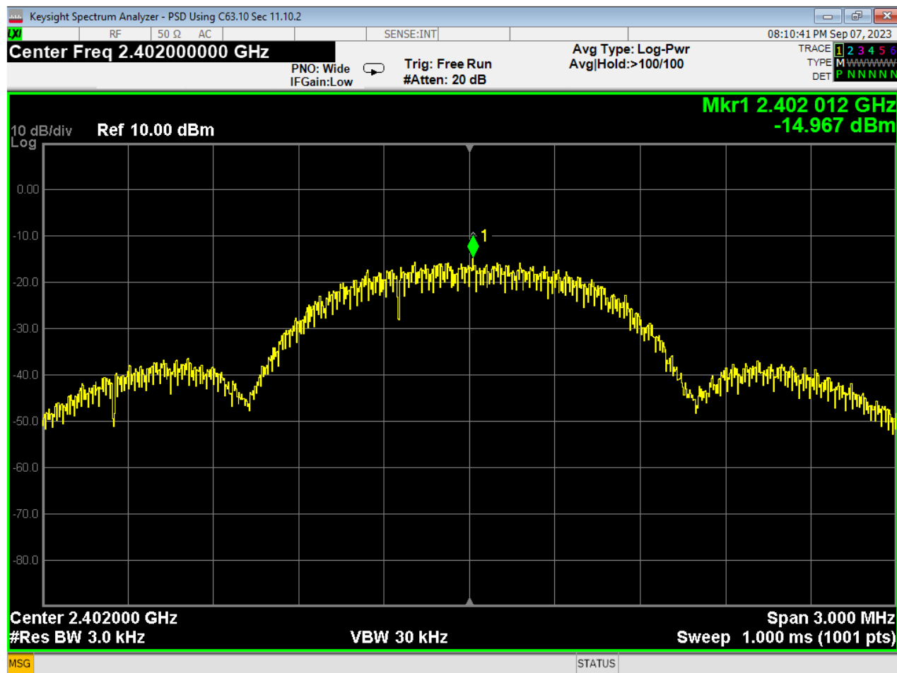
07 PSD, Low Channel, GFSK
