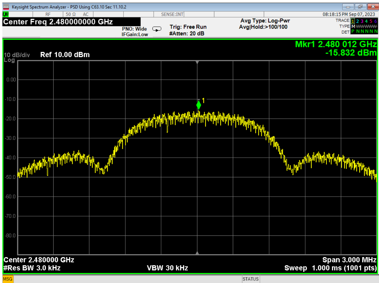
09 PSD, High Channel, GFSK
