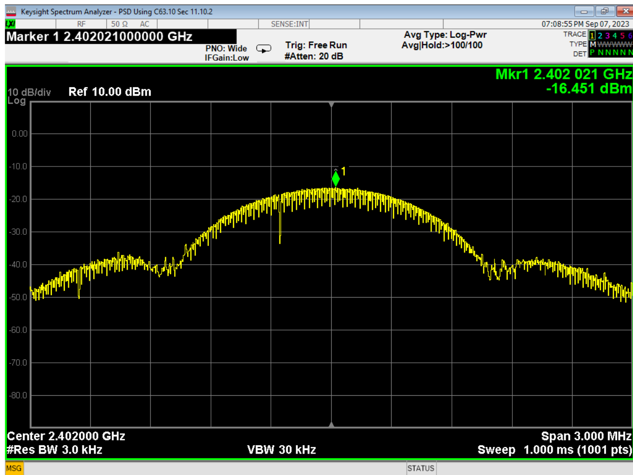
20 PSD, Low Channel, GMSK 1MB
