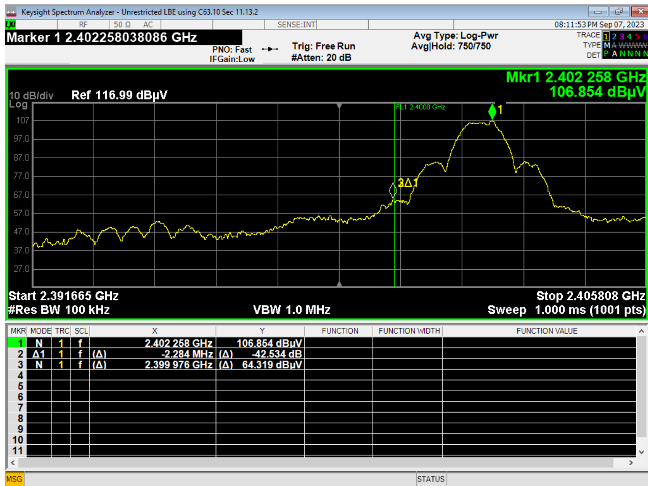
10 Lower Bandedge, Unrestricted, GFSK
