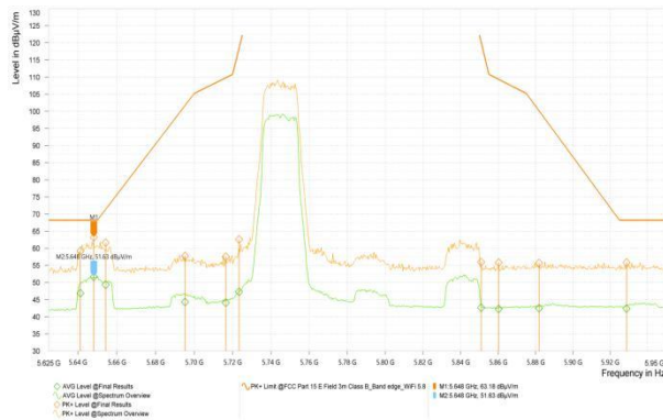
Wi-Fi 5G_11N40_5755
