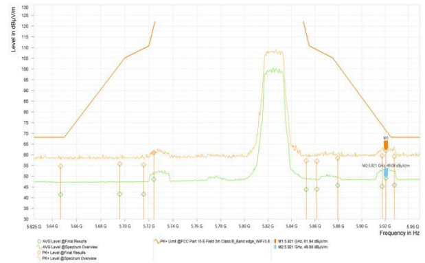
Wi-Fi 5G_11N20_5825
