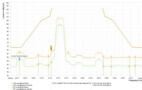
Wi-Fi 5G_11AC40_5755
