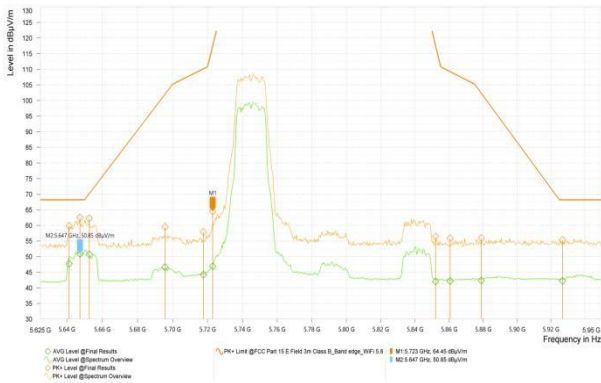
Wi-Fi 5G_11N20_5745
