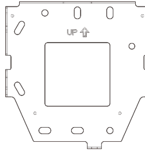
Wall-mount bracket
