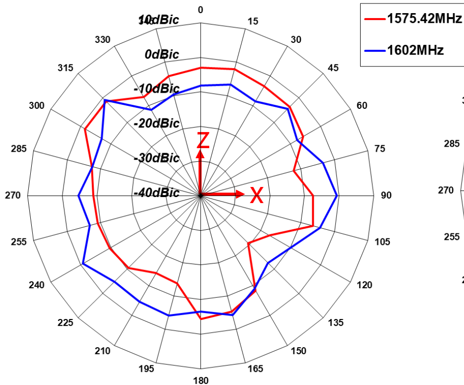
Circular Gain Radiation XZ Pattern
