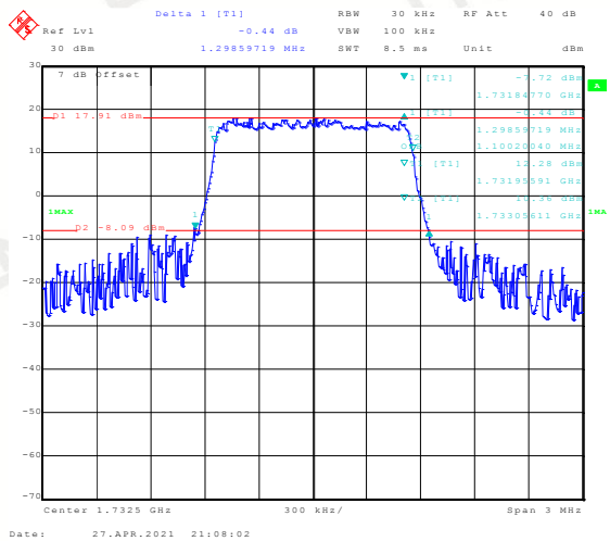
Band4-1.4MHz-16QAM-20175
