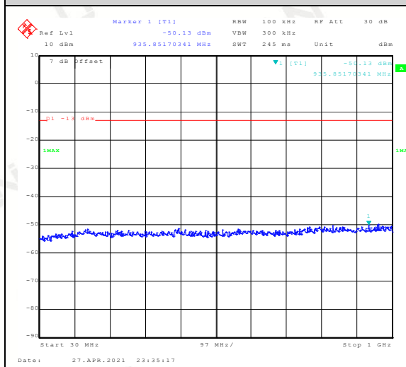
Band2-1.4MHz-QPSK-18900:30~1000MHz
