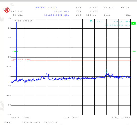
Band2-1.4MHz-QPSK-18900:1000~20000MHz
