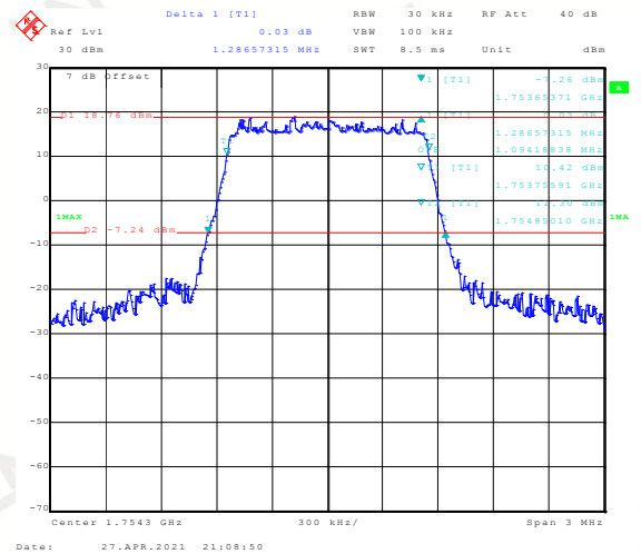
Band4-1.4MHz-16QAM-20393
