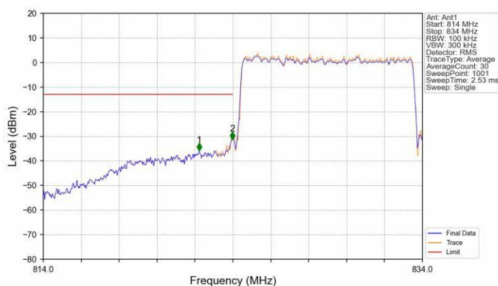
Band26b 10MHz 16QAM LCH 829MHz RB 50 0 NTNV
