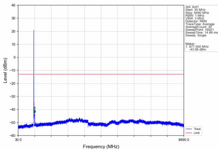
Band26b 15MHz 16QAM LCH 831.5MHz RB 75 0 NTNV
