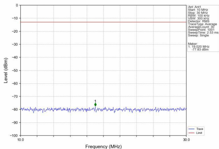
Band26b 10MHz 16QAM MCH 836.5MHz RB 1 0 NTNv
