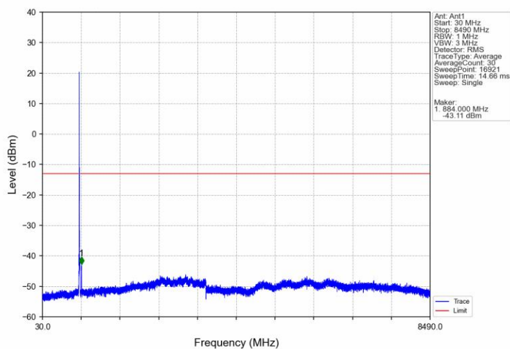
Band26b 10MHz 16QAM MCH 836.5MHz RB 1 0 NTNv
