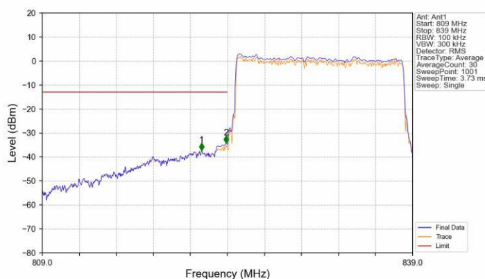
Band26b 15MHz 16QAM LCH 831.5MHz RB 75 0 NTNV
