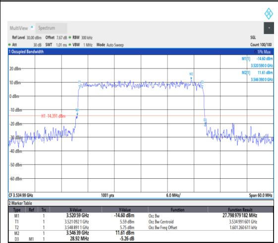
1-N78-3450-3550--30-30-H-7-CP-16QAM-Ou ter_Full-78@0-Ant1-27.799-28.920-≤30-
