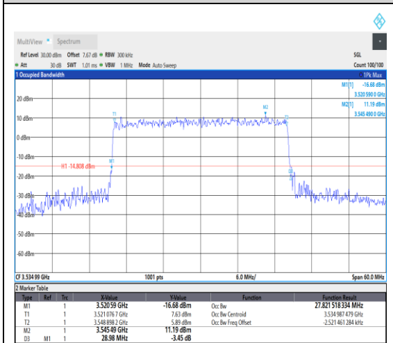
1-N78-3450-3550--30-30-H-8-CP-64QAM-Ou ter_Full-78@0-Ant1-27.822-28.980-≤30-
