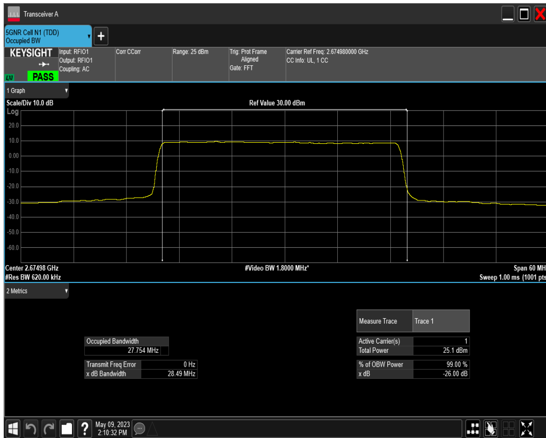
n41 SCS=30kHz DFT_QAM16 BW=30MHz Channel=534996 RB=75@0
