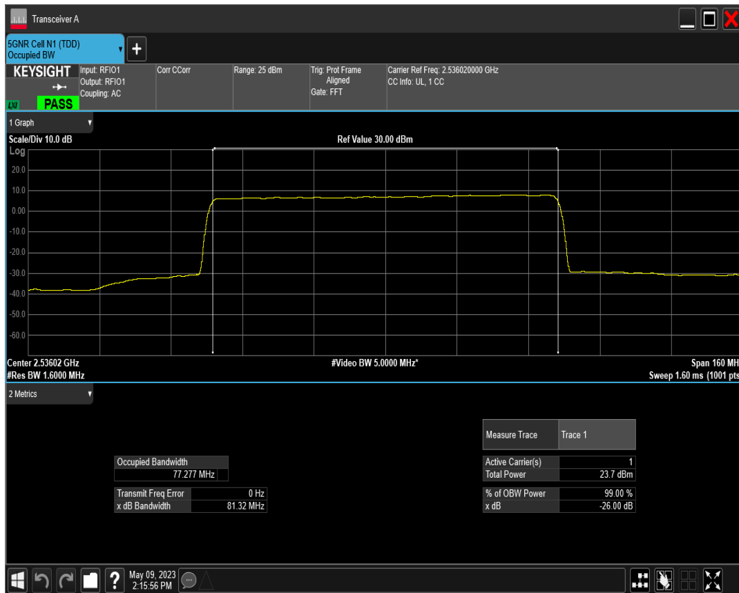
n41 SCS=30kHz DFT_QAM256 BW=80MHz Channel=507204 RB=216@0
