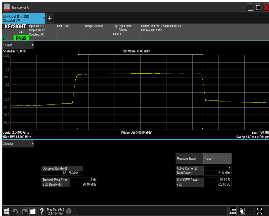
n41 SCS=30kHz CP_QPSK BW=90MHz Channel=508200 RB=245@0
