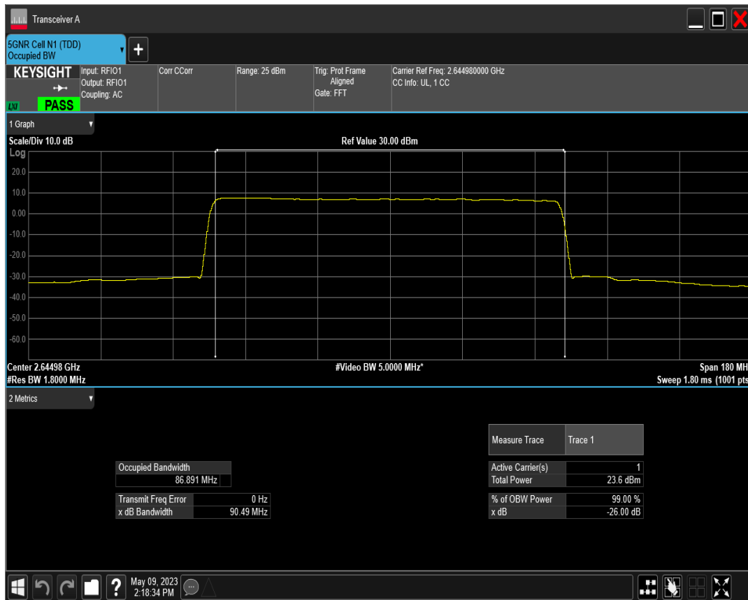
n41 SCS=30kHz DFT_QAM256 BW=90MHz Channel=528996 RB=240@0
