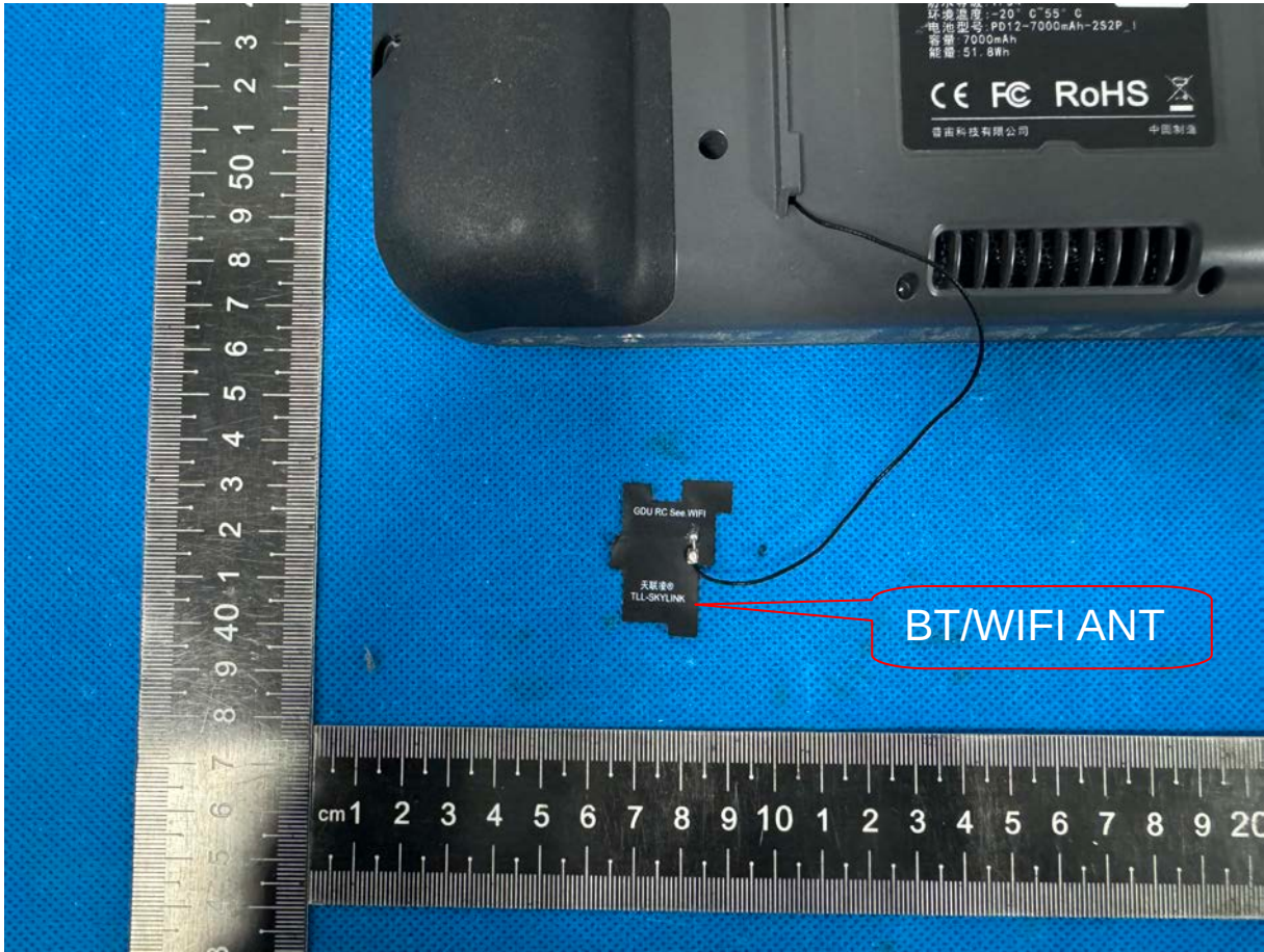
Photo 2 - WIFI / BT ANT location
