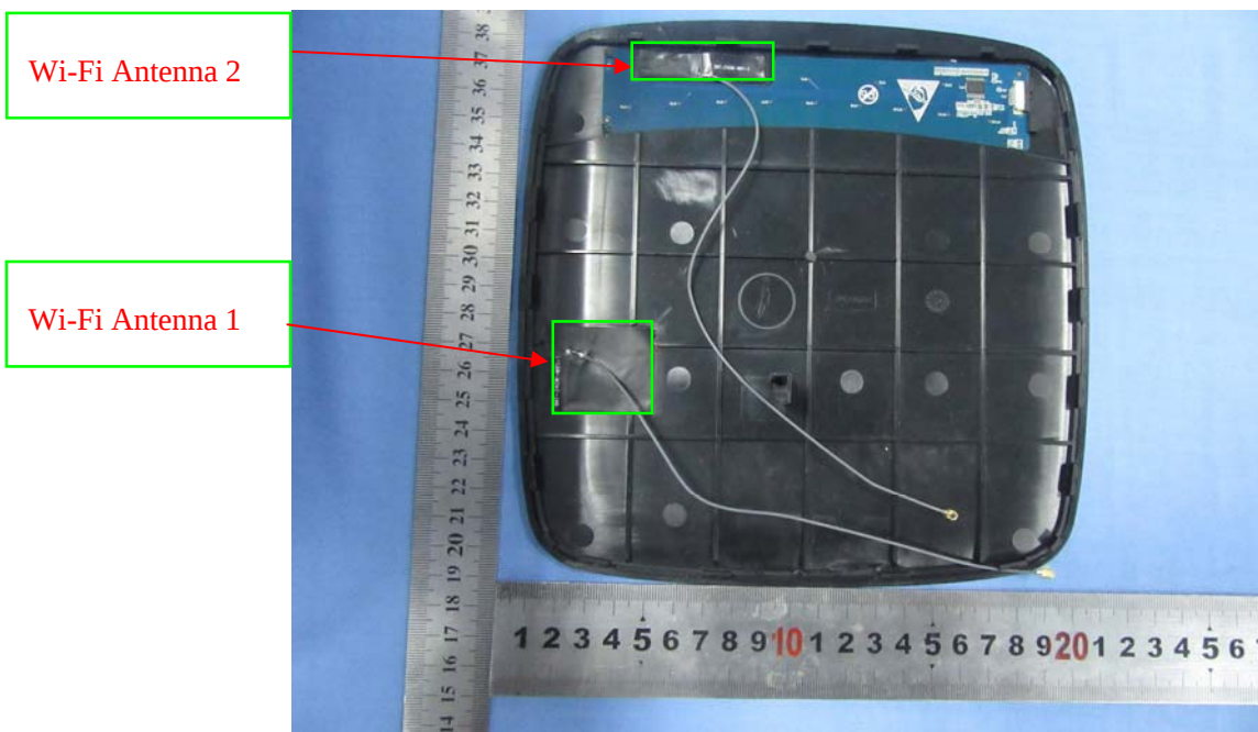
EUT – Wi-Fi Antenna View
