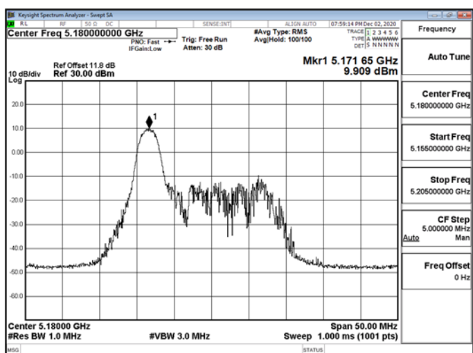
802.11ax_20MHz_RU_26_0_5180MHz-5180
