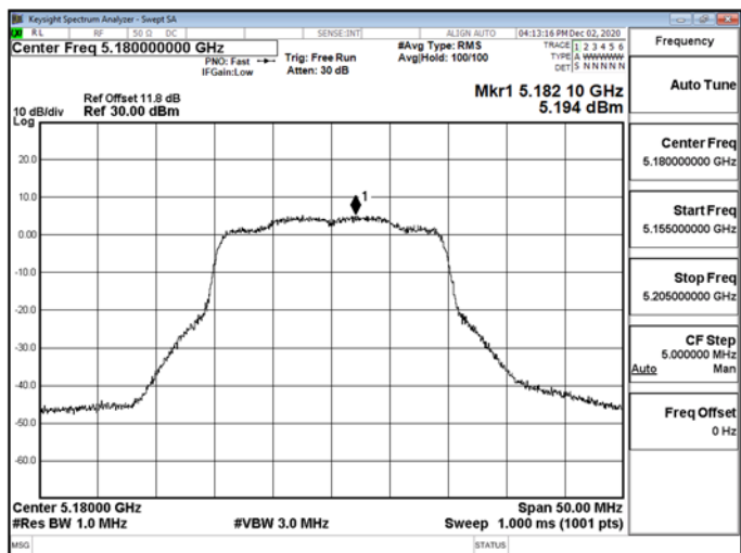
802.11ax_20MHz_RU_106_53_5180MHz-5180
