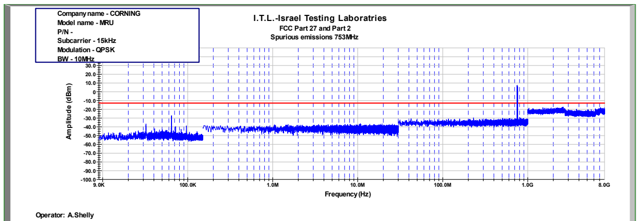
Figure 512: Spurious Emissions at Antenna Terminal QPSK 10MHz B.W.; 753.0MHz, 15kHz
