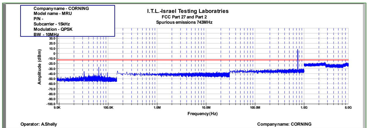
Figure 511: Spurious Emissions at Antenna Terminal QPSK 10MHz B.W.; 743.0MHz, 15kHz
