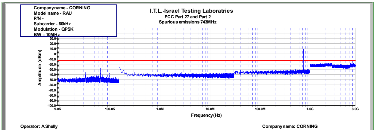
Figure 517: Spurious Emissions at Antenna Terminal QPSK 10MHz B.W.; 743.0MHz, 60kHz
