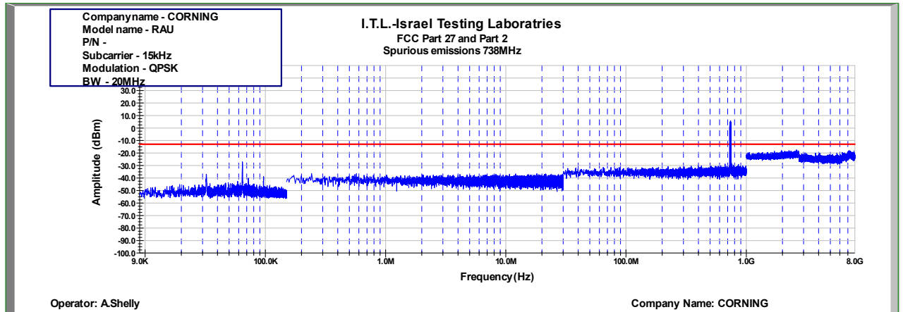
Figure 528: Spurious Emissions at Antenna Terminal QPSK 20MHz B.W.; 738.0MHz, 15kHz
