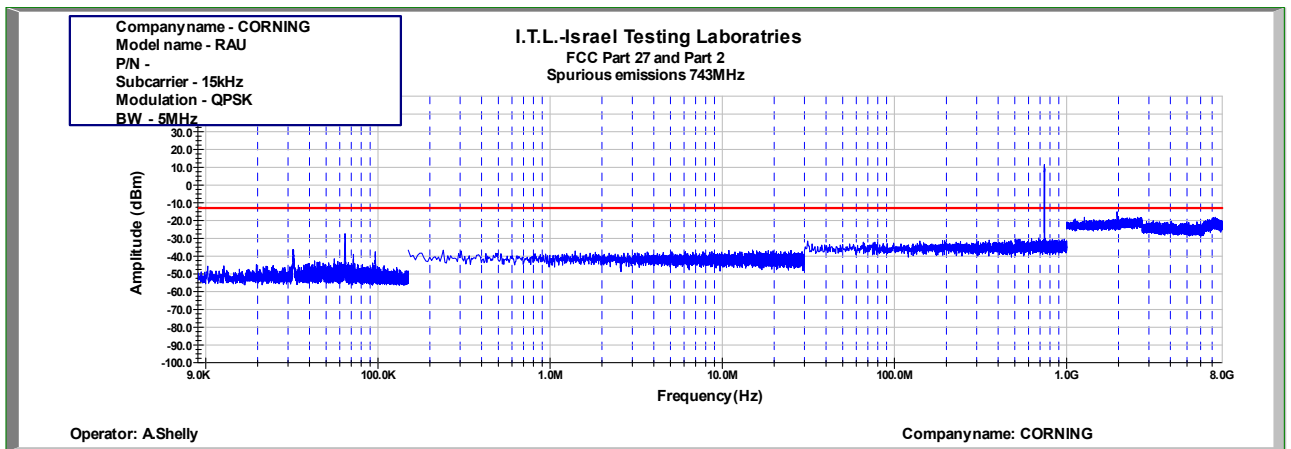
Figure 505: Spurious Emissions at Antenna Terminal QPSK 5MHz B.W.; 743.0MHz, 15kHz
