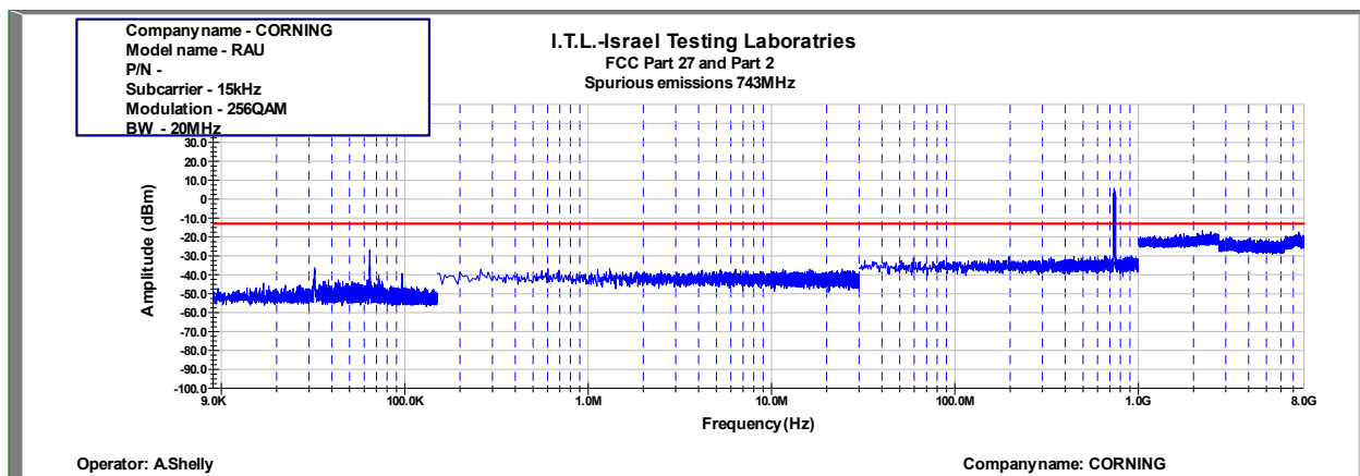
Figure 496: Spurious Emissions at Antenna Terminal 256QAM 20MHz B.W.; 743.0MHz, 15kHz
