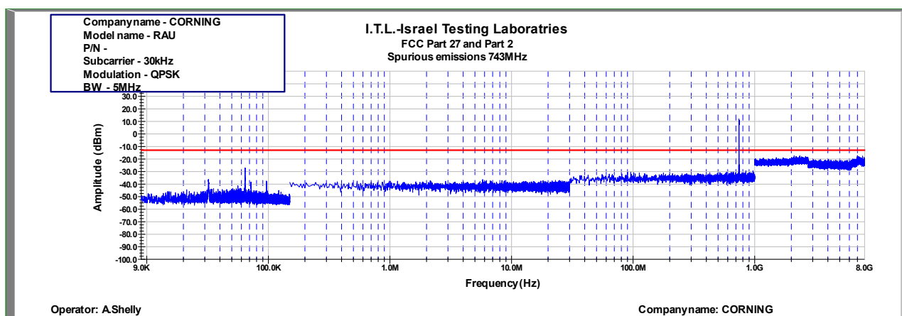
Figure 508: Spurious Emissions at Antenna Terminal QPSK 5MHz B.W.; 743.0MHz, 30kHz
