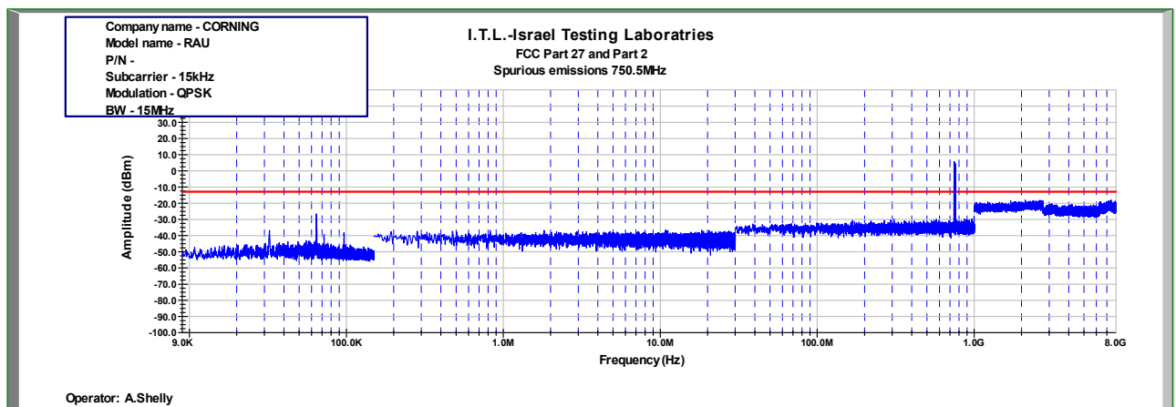
Figure 521: Spurious Emissions at Antenna Terminal QPSK 15MHz B.W.; 750.5MHz, 15kHz
