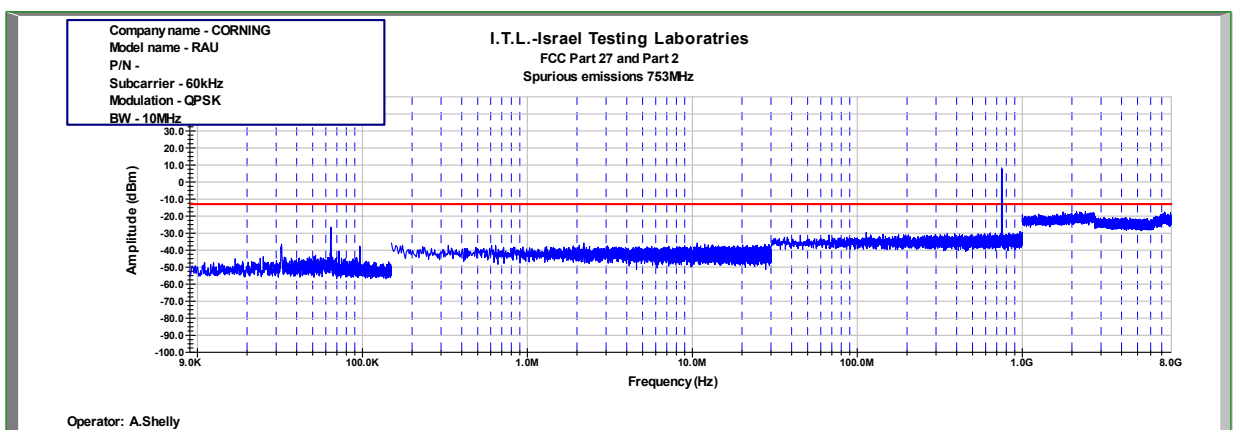
Figure 518: Spurious Emissions at Antenna Terminal QPSK 10MHz B.W.; 753.0MHz, 60kHz
