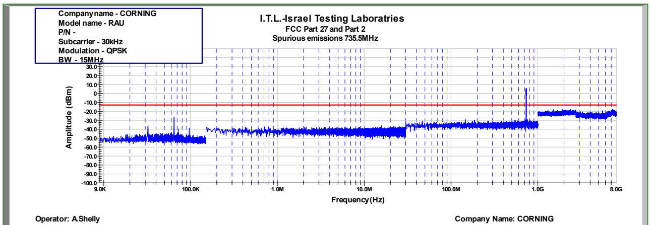
Figure 522: Spurious Emissions at Antenna Terminal QPSK 15MHz B.W.; 735.5MHz, 30kHz
