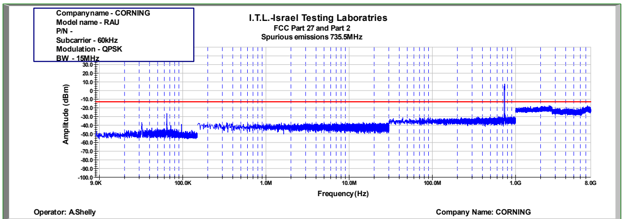
Figure 525: Spurious Emissions at Antenna Terminal QPSK 15MHz B.W.; 735.5MHz, 60kHz
