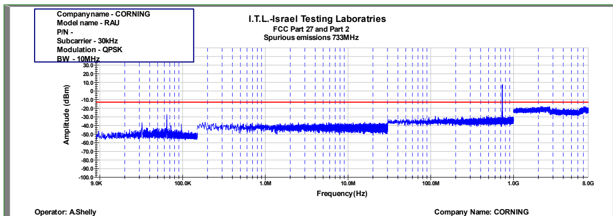
Figure 513: Spurious Emissions at Antenna Terminal QPSK 10MHz B.W.; 733.0MHz, 30kHz
