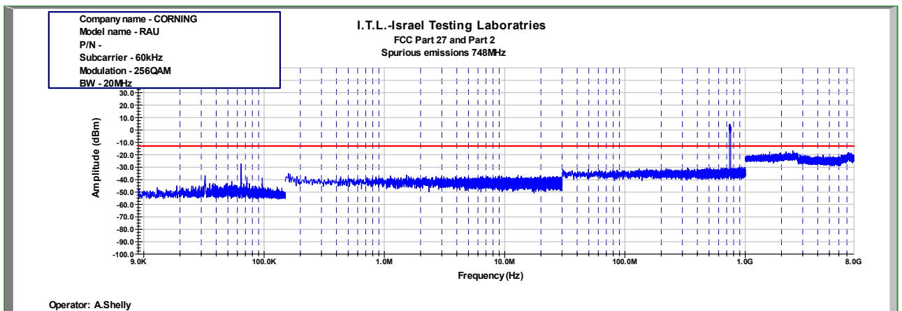
Figure 503: Spurious Emissions at Antenna Terminal 256QAM 20MHz B.W.; 748.0MHz, 60kHz
