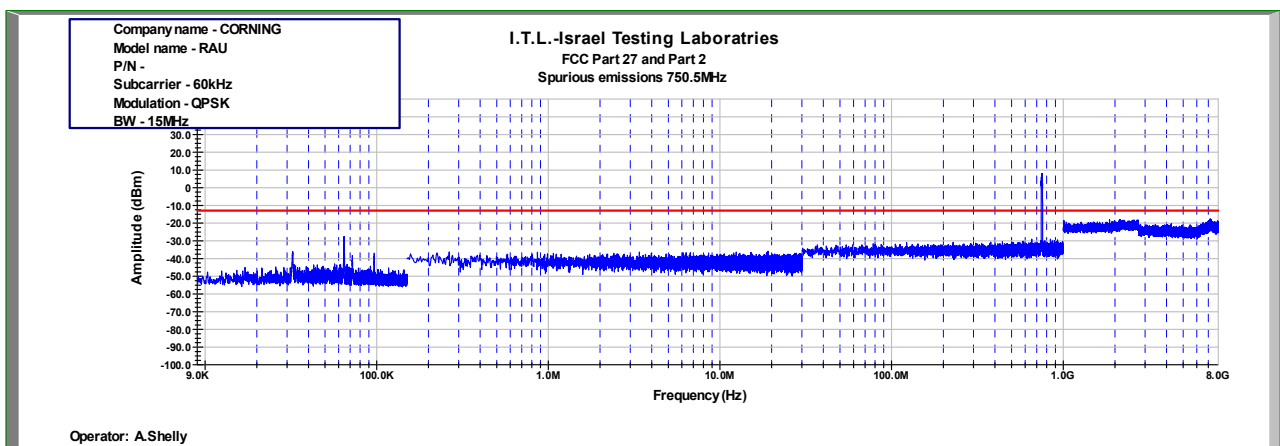
Figure 527: Spurious Emissions at Antenna Terminal QPSK 15MHz B.W.; 750.5MHz, 60kHz
