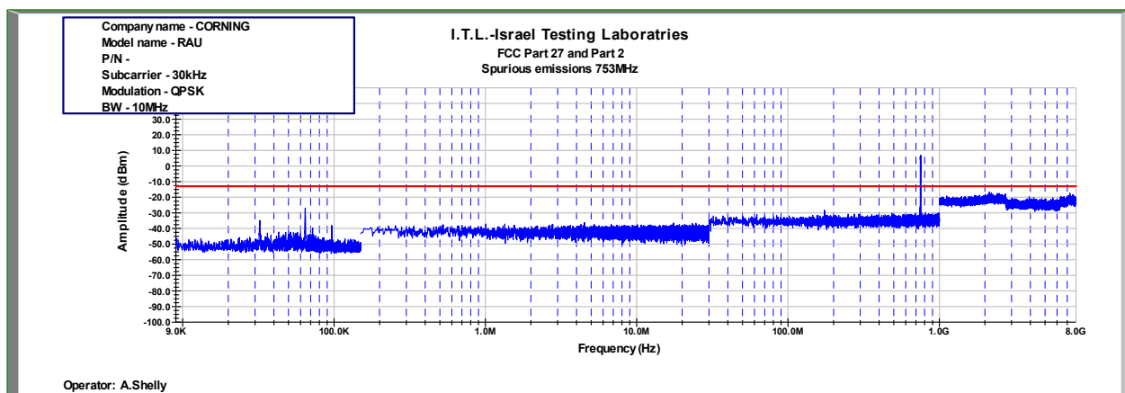
Figure 515: Spurious Emissions at Antenna Terminal QPSK 10MHz B.W.; 753.0MHz, 30kHz
