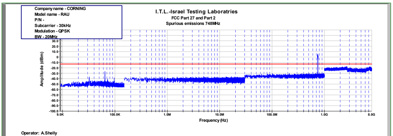
Figure 533: Spurious Emissions at Antenna Terminal QPSK 20MHz B.W.; 748.0MHz, 30kHz
