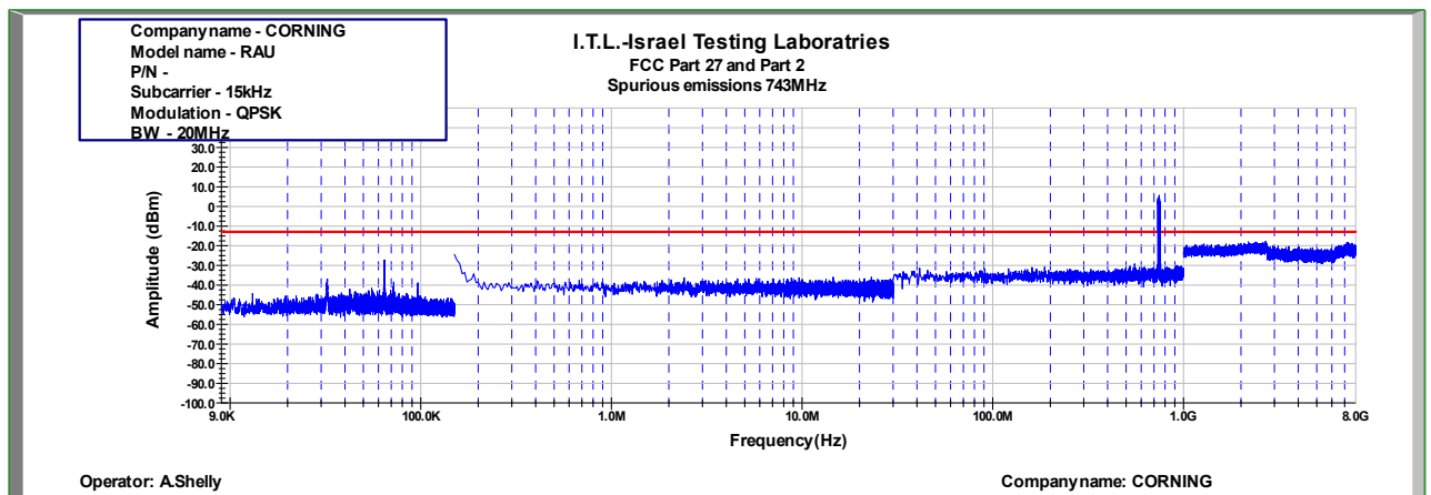
Figure 529: Spurious Emissions at Antenna Terminal QPSK 20MHz B.W.; 743.0MHz, 15kHz
