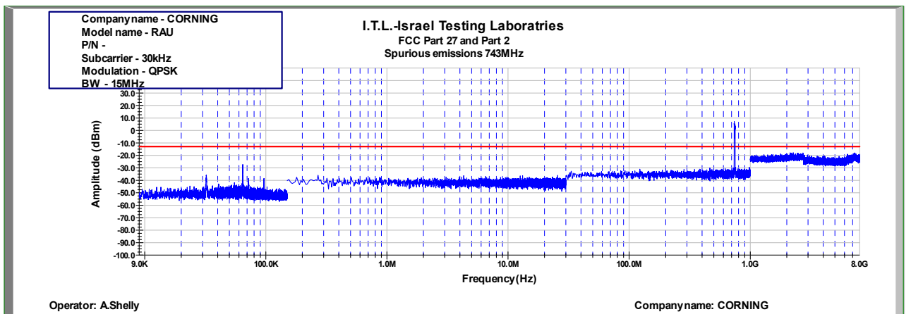
Figure 523: Spurious Emissions at Antenna Terminal QPSK 15MHz B.W.; 743.0MHz, 30kHz
