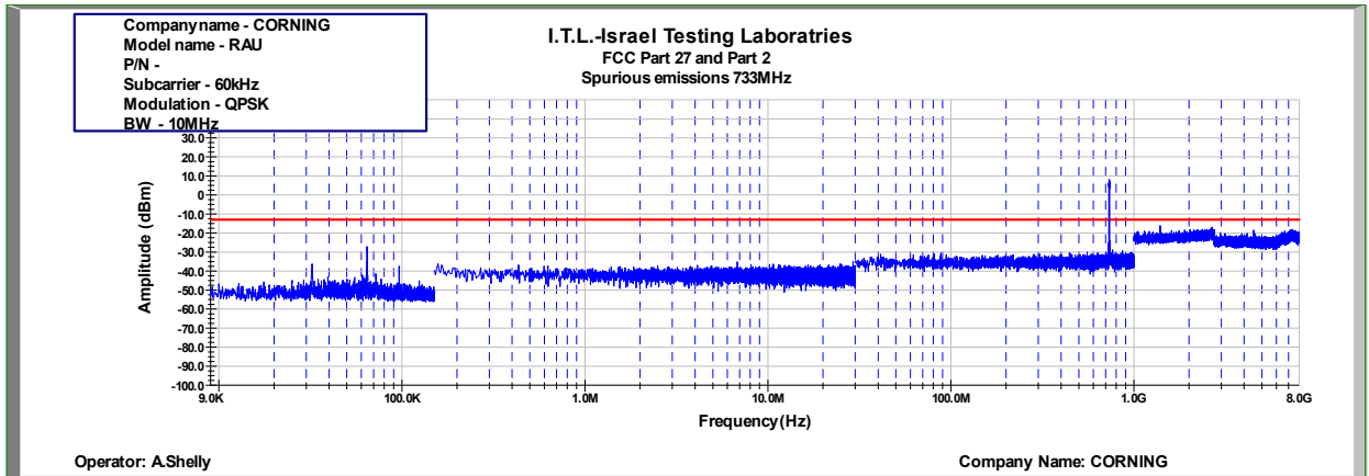
Figure 516: Spurious Emissions at Antenna Terminal QPSK 10MHz B.W.; 733.0MHz, 60kHz
