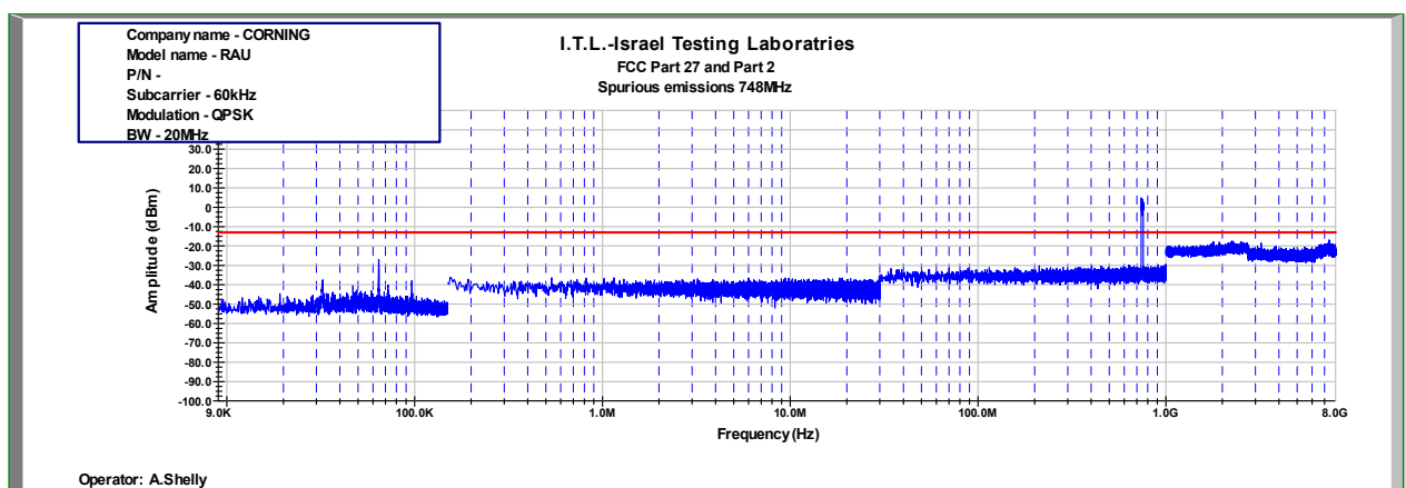
Figure 536: Spurious Emissions at Antenna Terminal QPSK 20MHz B.W.; 748.0MHz, 60kHz
