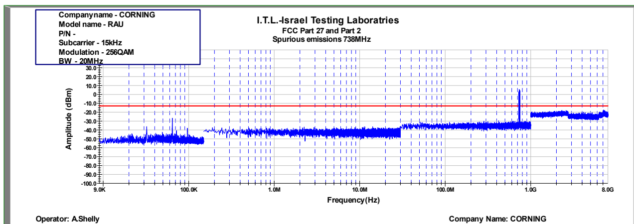
Figure 495: Spurious Emissions at Antenna Terminal 256QAM 20MHz B.W.; 738.0MHz, 15kHz
