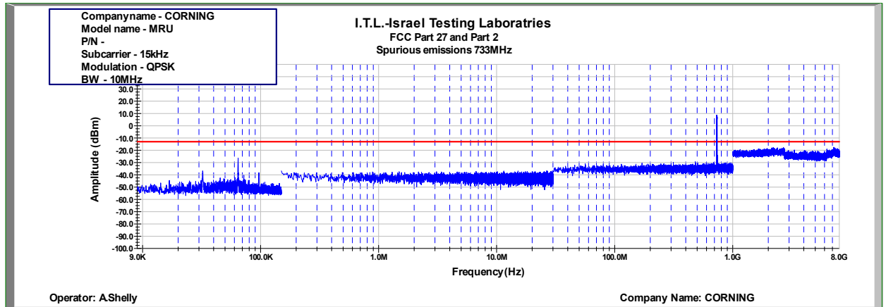
Figure 510: Spurious Emissions at Antenna Terminal QPSK 10MHz B.W.; 733.0MHz, 15kHz
