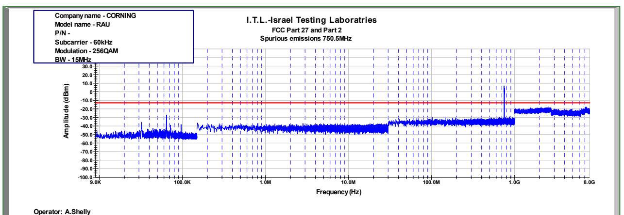
Figure 494: Spurious Emissions at Antenna Terminal 256QAM 15MHz B.W.; 750.5MHz, 60kHz
