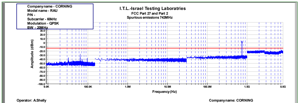
Figure 535: Spurious Emissions at Antenna Terminal QPSK 20MHz B.W.; 743.0MHz, 60kHz
