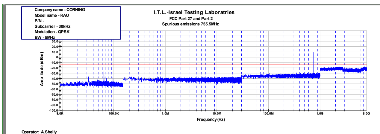
Figure 509: Spurious Emissions at Antenna Terminal QPSK 5MHz B.W.; 755.5MHz, 30kHz
