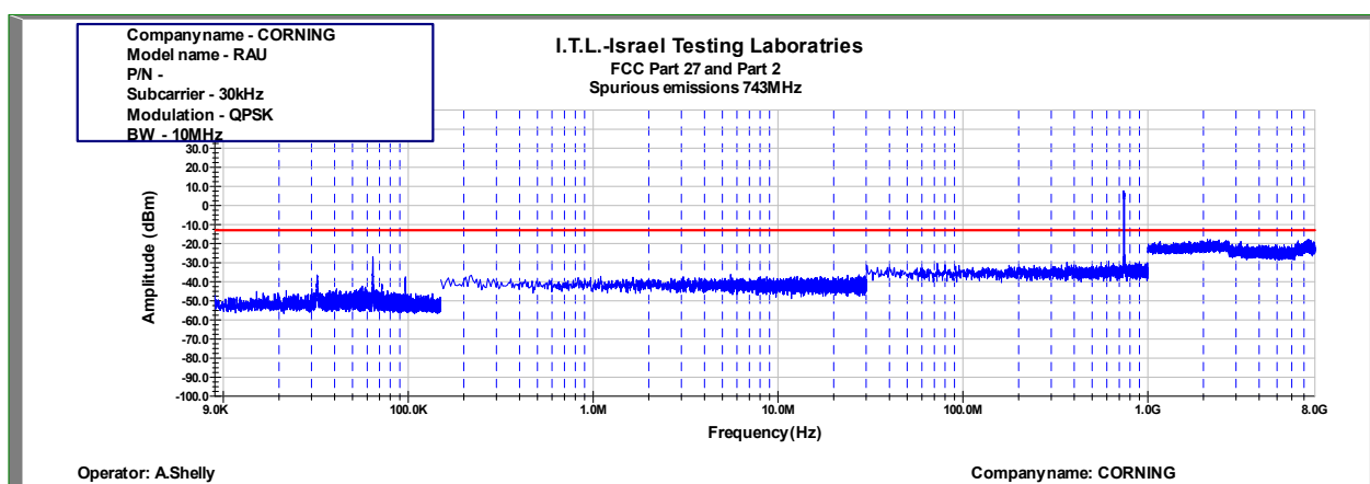
Figure 514: Spurious Emissions at Antenna Terminal QPSK 10MHz B.W.; 743.0MHz, 30kHz
