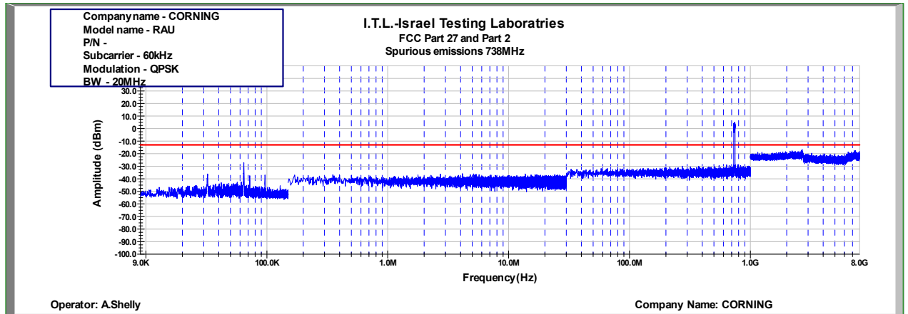
Figure 534: Spurious Emissions at Antenna Terminal QPSK 20MHz B.W.; 738.0MHz, 60kHz
