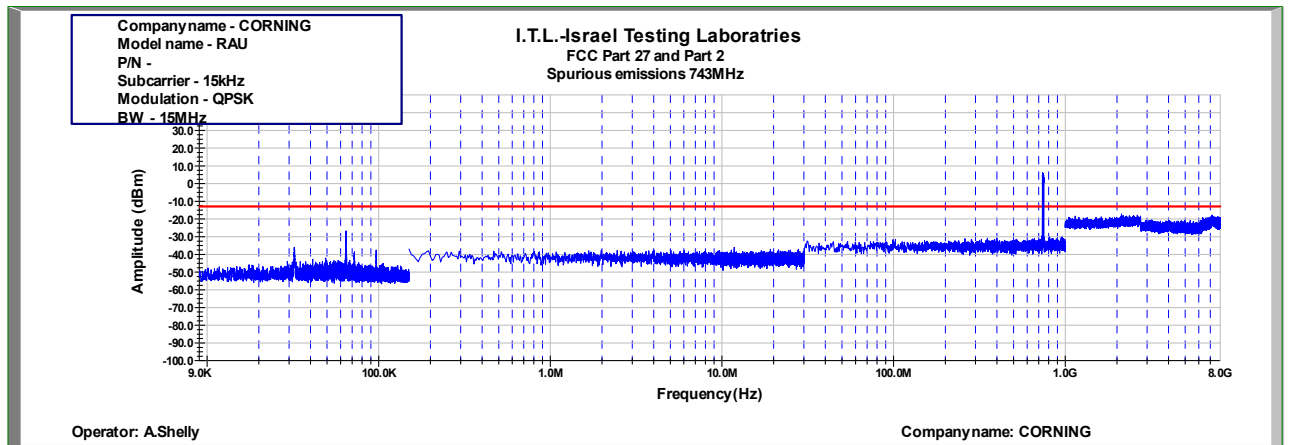
Figure 520: Spurious Emissions at Antenna Terminal QPSK 15MHz B.W.; 743.0MHz, 15kHz
