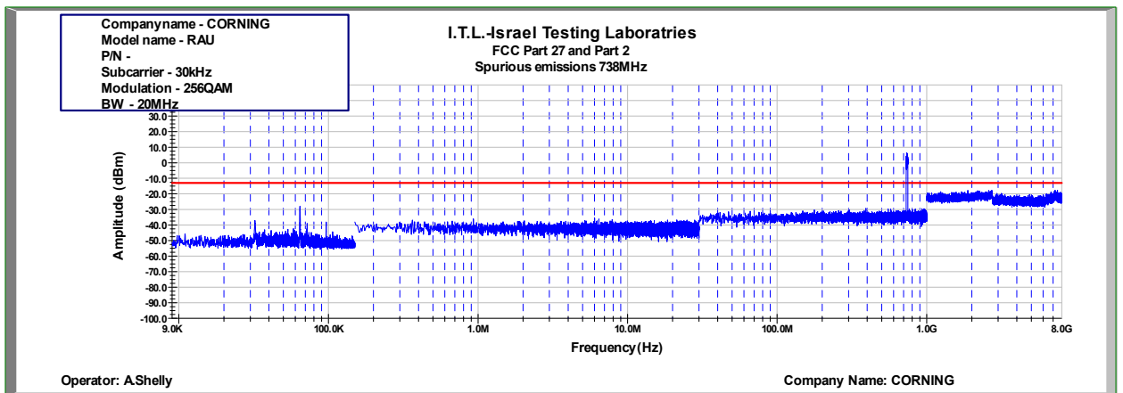
Figure 498: Spurious Emissions at Antenna Terminal 256QAM 20MHz B.W.; 738.0MHz, 30kHz
