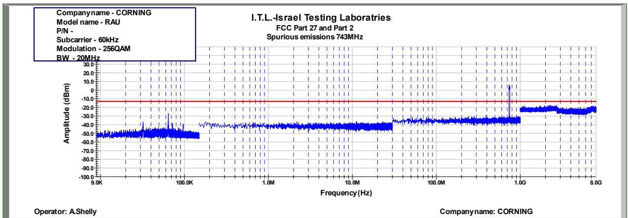
Figure 502: Spurious Emissions at Antenna Terminal 256QAM 20MHz B.W.; 743.0MHz, 60kHz
