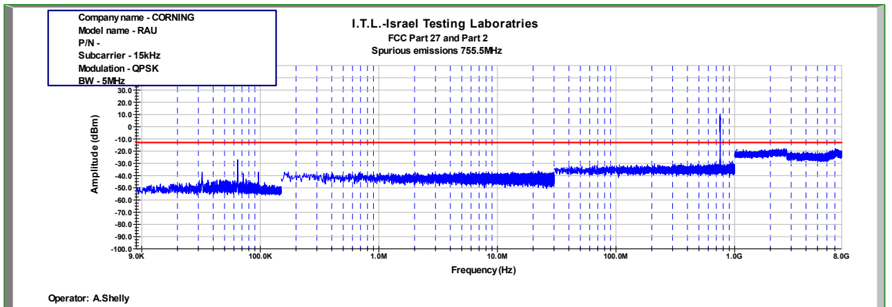
Figure 506: Spurious Emissions at Antenna Terminal QPSK 5MHz B.W.; 755.5MHz, 15kHz
