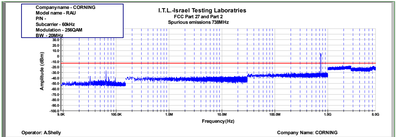
Figure 501: Spurious Emissions at Antenna Terminal 256QAM 20MHz B.W.; 738.0MHz, 60kHz
