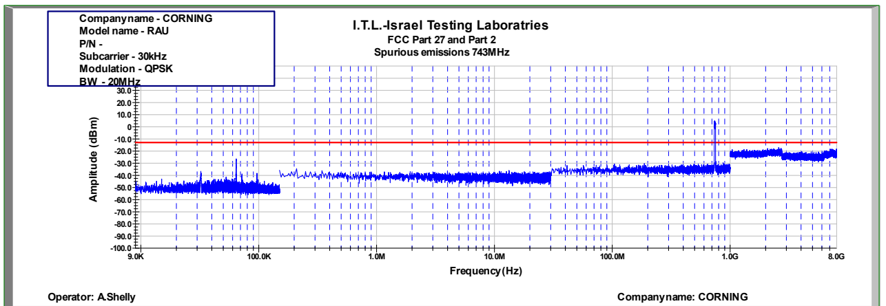
Figure 532: Spurious Emissions at Antenna Terminal QPSK 20MHz B.W.; 743.0MHz, 30kHz
