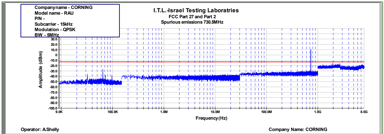
Figure 504: Spurious Emissions at Antenna Terminal QPSK 5MHz B.W.; 730.5MHz, 15kHz
