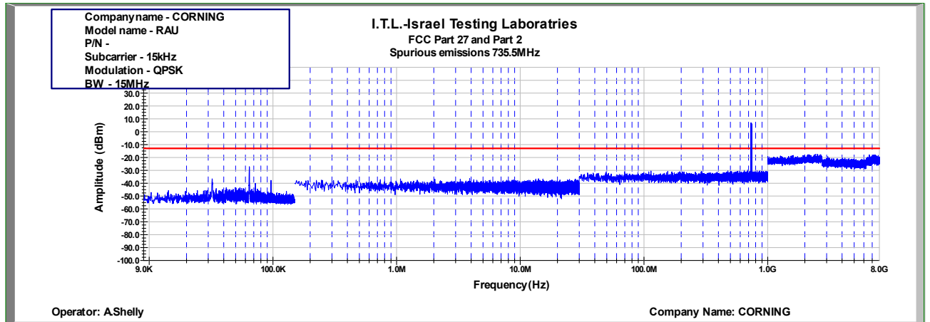
Figure 519: Spurious Emissions at Antenna Terminal QPSK 15MHz B.W.; 735.5MHz, 15kHz
