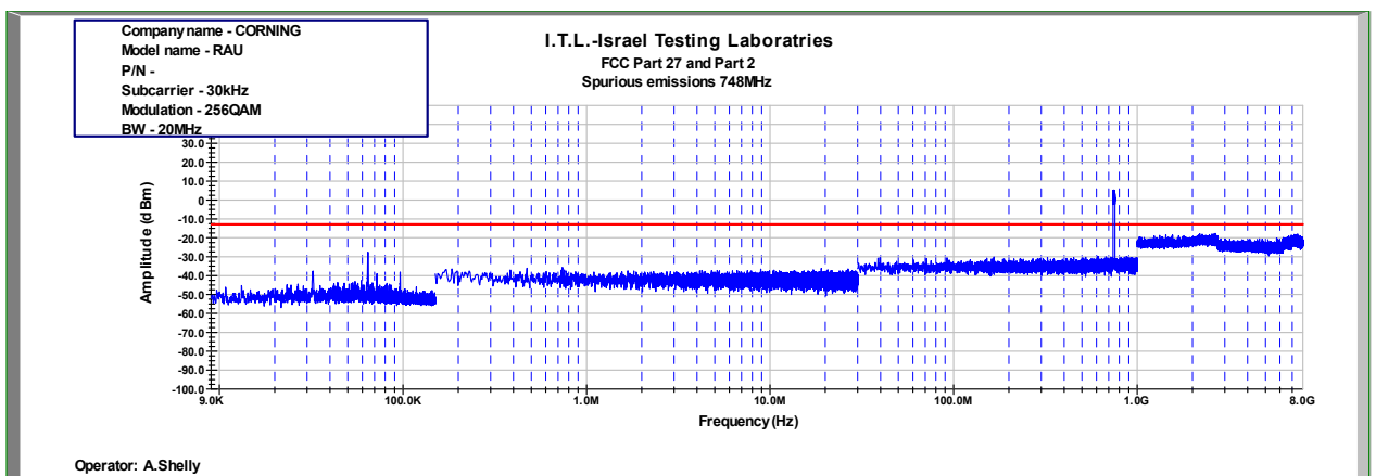
Figure 500: Spurious Emissions at Antenna Terminal 256QAM 20MHz B.W.; 748.0MHz, 30kHz
