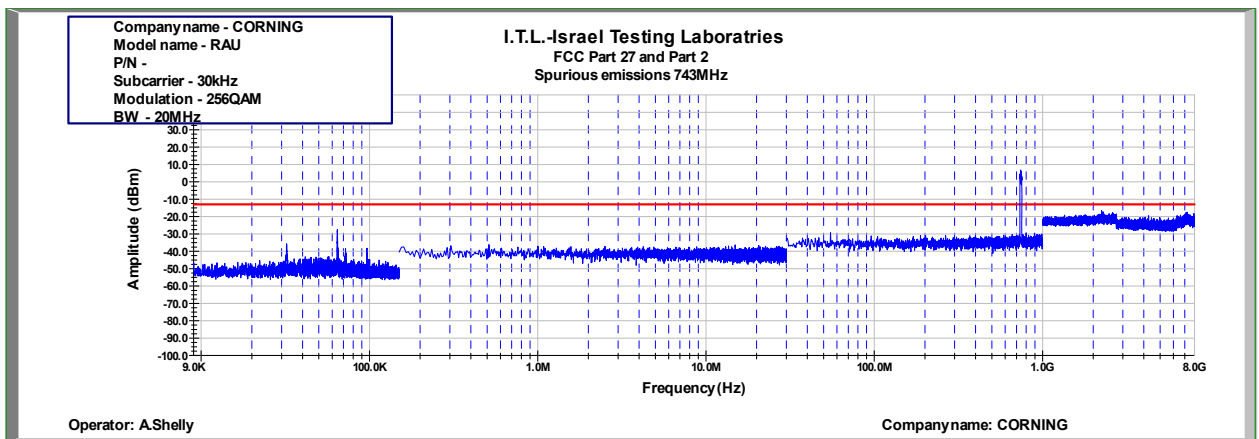
Figure 499: Spurious Emissions at Antenna Terminal 256QAM 20MHz B.W.; 743.0MHz, 30kHz
