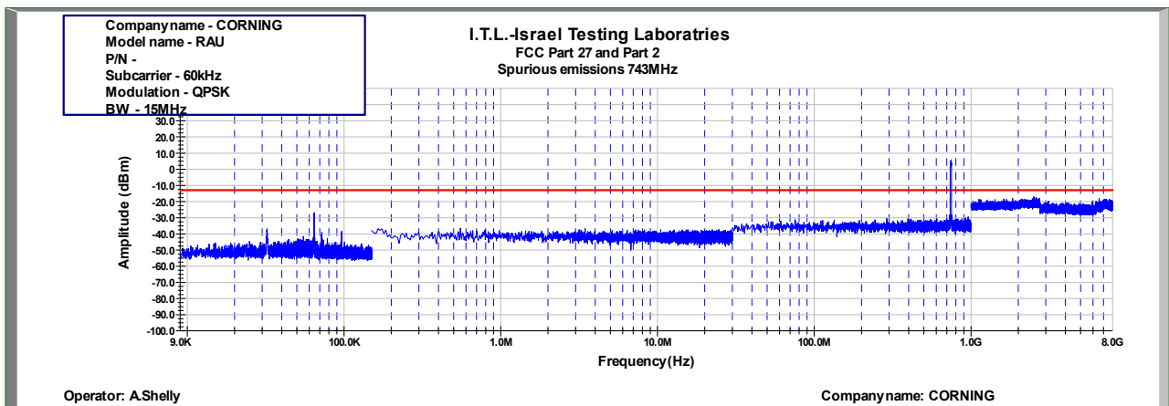
Figure 526: Spurious Emissions at Antenna Terminal QPSK 15MHz B.W.; 743.0MHz, 60kHz
