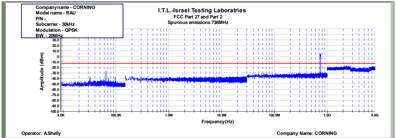
Figure 531: Spurious Emissions at Antenna Terminal QPSK 20MHz B.W.; 738.0MHz, 30kHz
