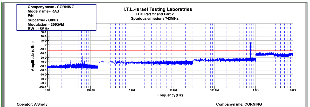
Figure 493: Spurious Emissions at Antenna Terminal 256QAM 15MHz B.W.; 743.0MHz, 60kHz
