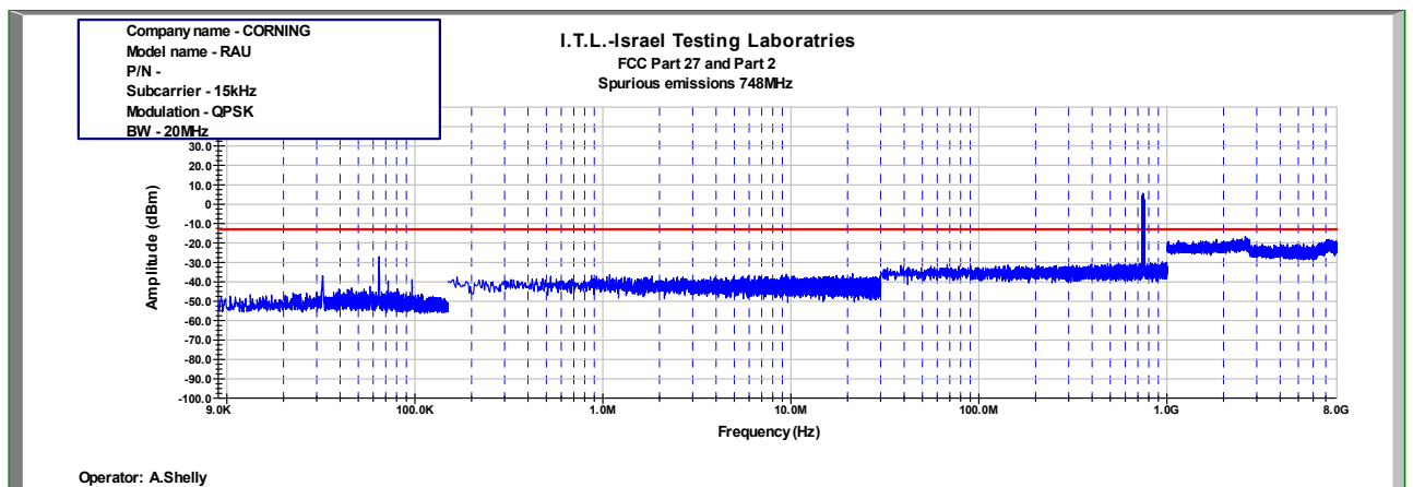
Figure 530: Spurious Emissions at Antenna Terminal QPSK 20MHz B.W.; 748.0MHz, 15kHz
