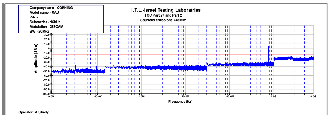
Figure 497: Spurious Emissions at Antenna Terminal 256QAM 20MHz B.W.; 748.0MHz, 15kHz
