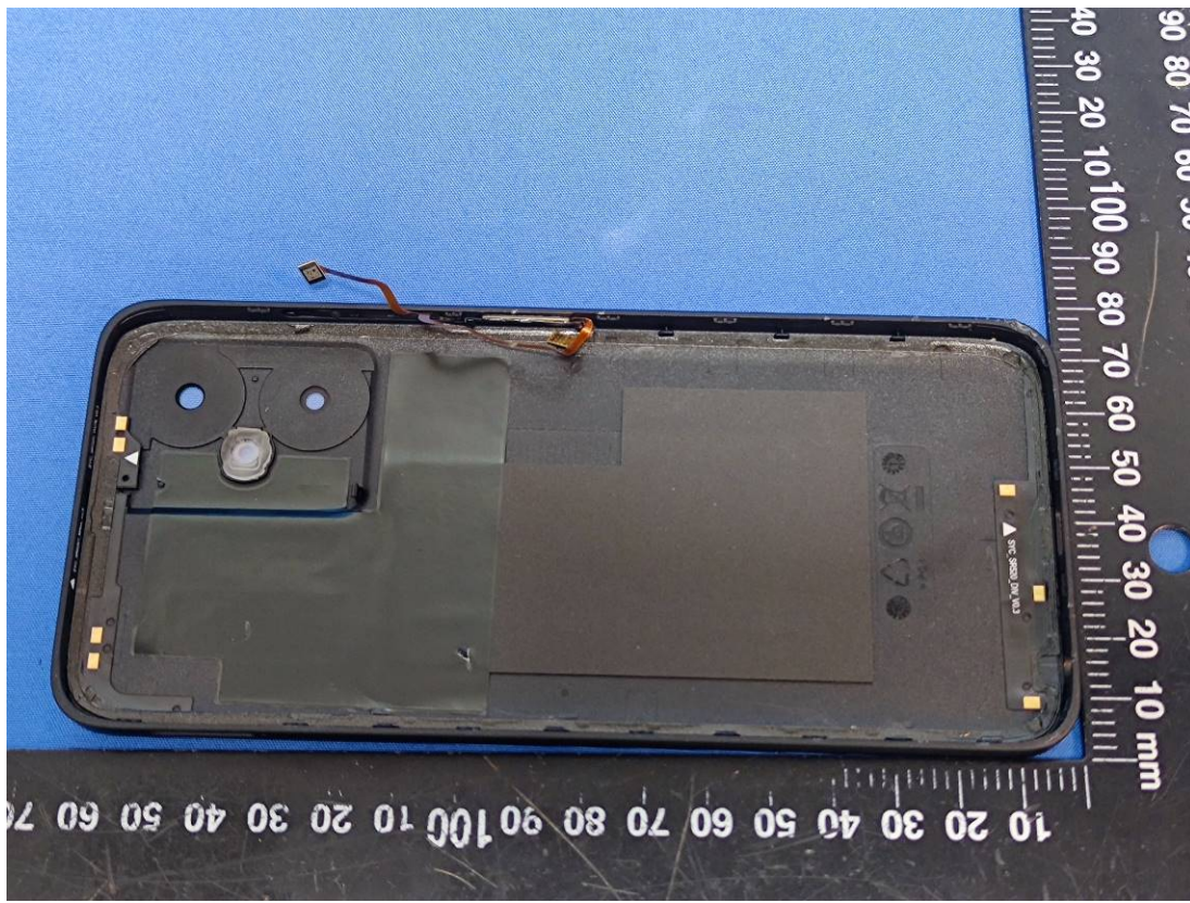
LTE DIV Antenna(only for receive)
