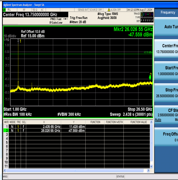
11B-Ant2-2437-1000~26500-PASS
