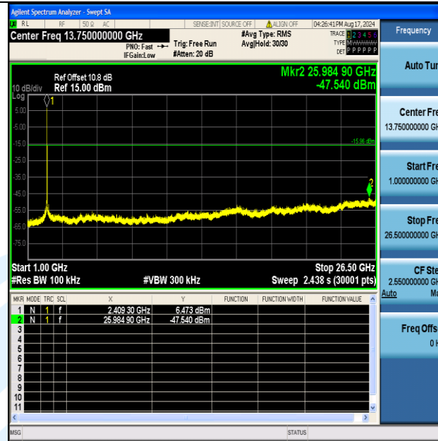
11G-Ant2-2412-1000~26500-PASS
