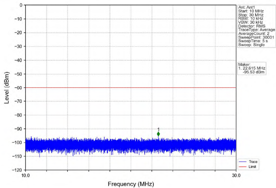
n48_30kHz_SISO_NTNV_10MHz_CP-OFDM_QPSK_3624.99MHz_Edge_1RB_Left
