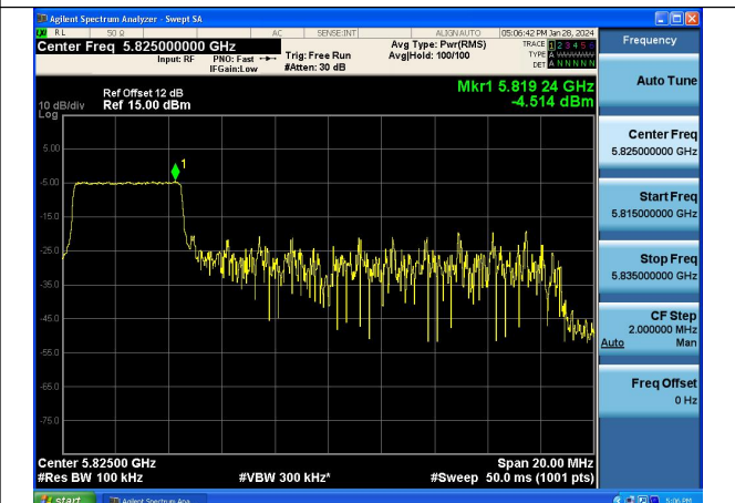
Mode:802.11ax HE20 Tone:52T Frequency:5825MHz Ant:Chain1
