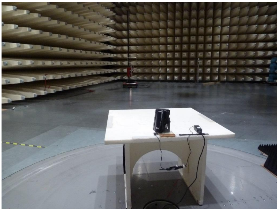
Photo 6 (RSE set-up /semi-anechoic chamber):
