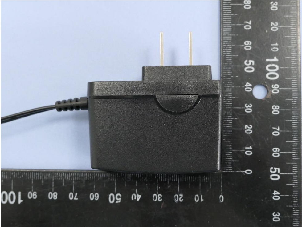
(17) EUT Photo (Brand: tp-link, M/N: T090060-2B1)
