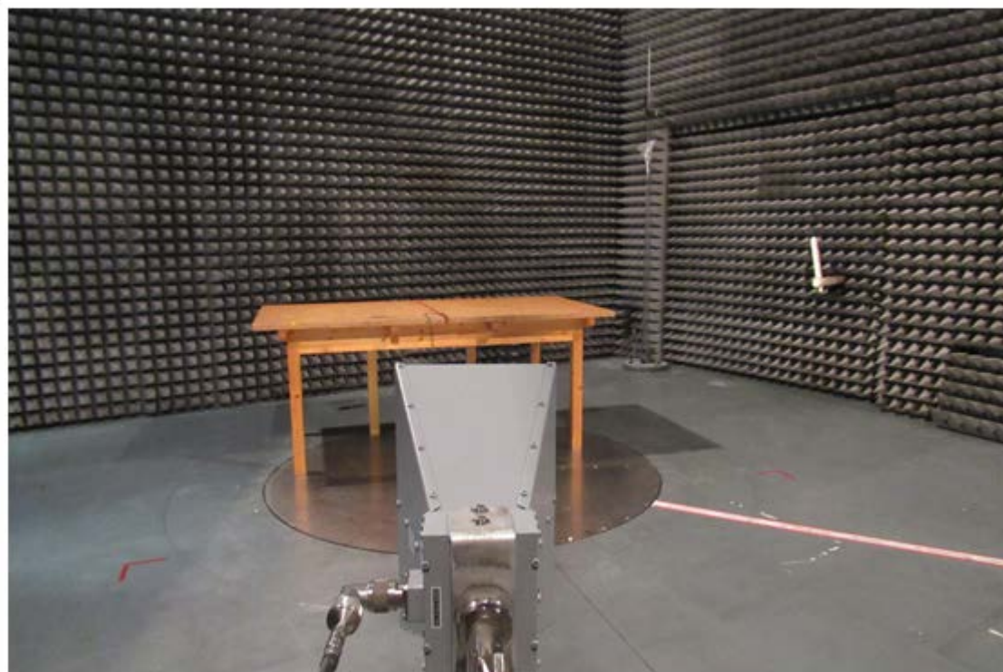
Radiated Setup
