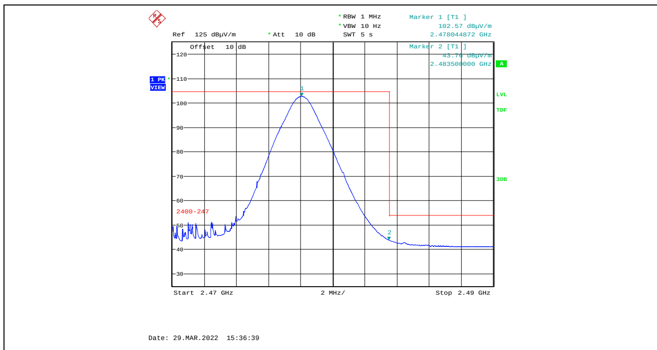
Plot 5.4.4.5.2.8. Band-Edge RF Radiated Emissions at 3 m, Horizontal Polarization, Average High End of Frequency Band, 2478 MHz, 8 dBm Power Setting, 2 Mbps
