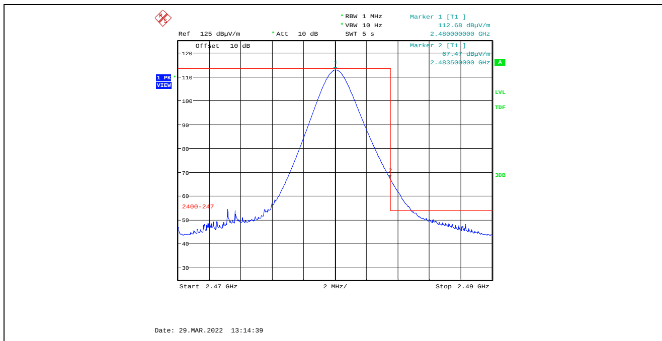
Plot 5.4.4.2.2.6. Band-Edge RF Radiated Emissions at 3 m, Vertical Polarization, Average High End of Frequency Band, 2480 MHz, 8 dBm Power Setting, 1 Mbps Marker 2: 67.47 dBμV/m – 33.51 dB Duty Cycle Factor = 33.96 dBμV/m (Limit 54 dBμV/m)
