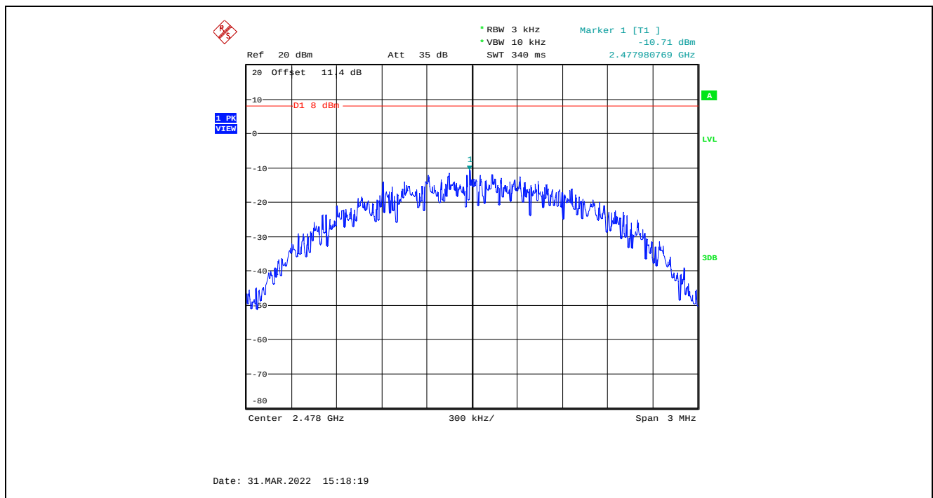
Plot 5.5.4.6. Power Spectral Density, GFSK Modulation, 2 Mbps, 8 dBm Power Setting, 2478 MHz
