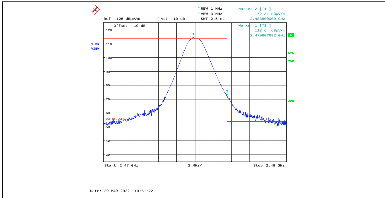
Plot 5.4.4.4.2.5. Band-Edge RF Radiated Emissions at 3 m, Vertical Polarization, Peak High End of Frequency Band, 2480 MHz, 8 dBm Power Setting, 1 Mbps
