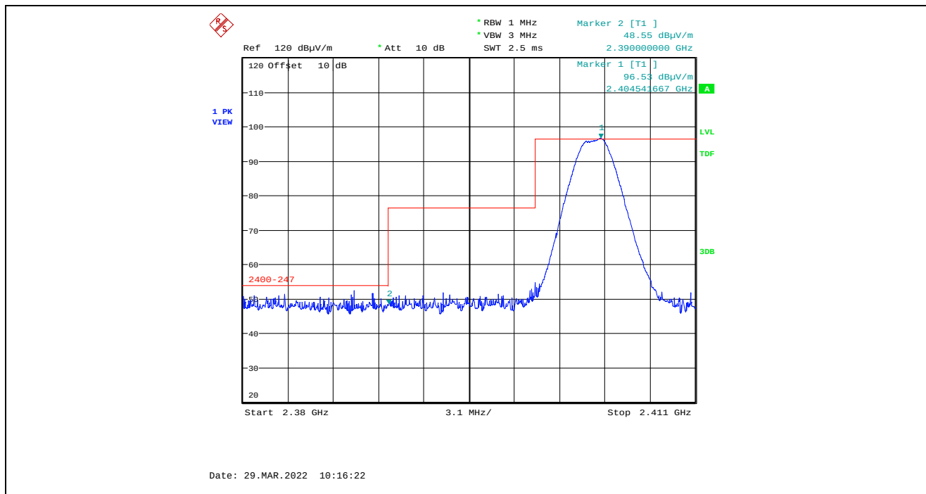
Plot 5.4.4.7.2.3. Band-Edge RF Radiated Emissions at 3 m, Horizontal Polarization, Peak Low End of Frequency Band, 2404 MHz, 8 dBm Power Setting, 2 Mbps
