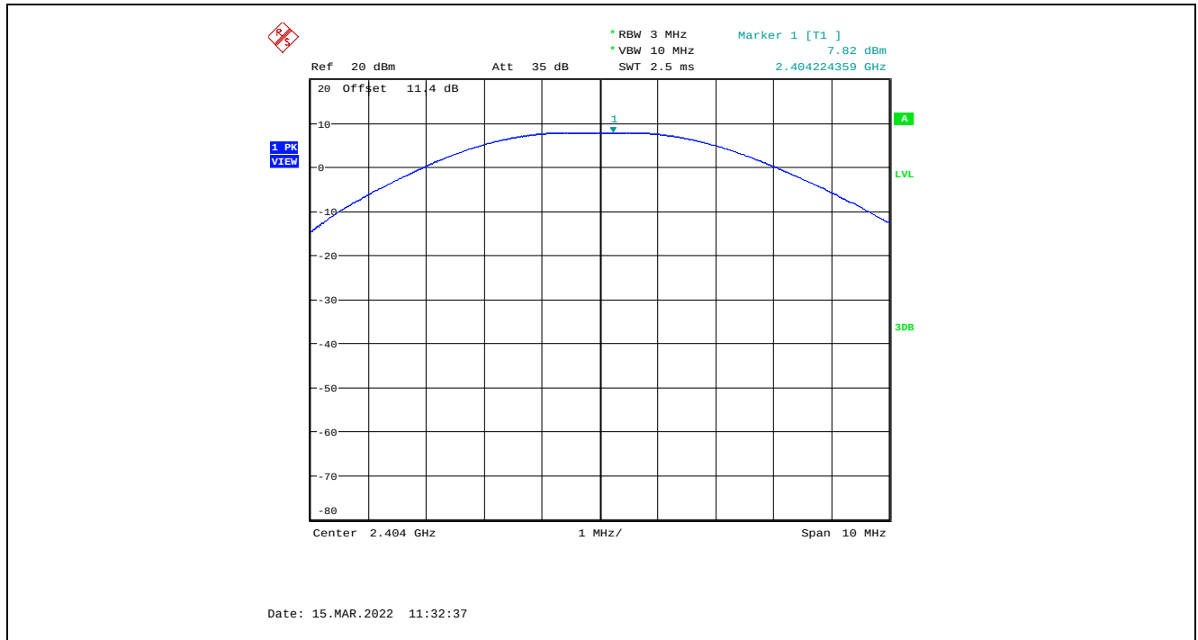
Plot 5.3.4.7. Maximum Peak Conducted Output Power, GFSK Modulation, 2 Mbps, 8 dBm Power Setting, 2404 MHz
