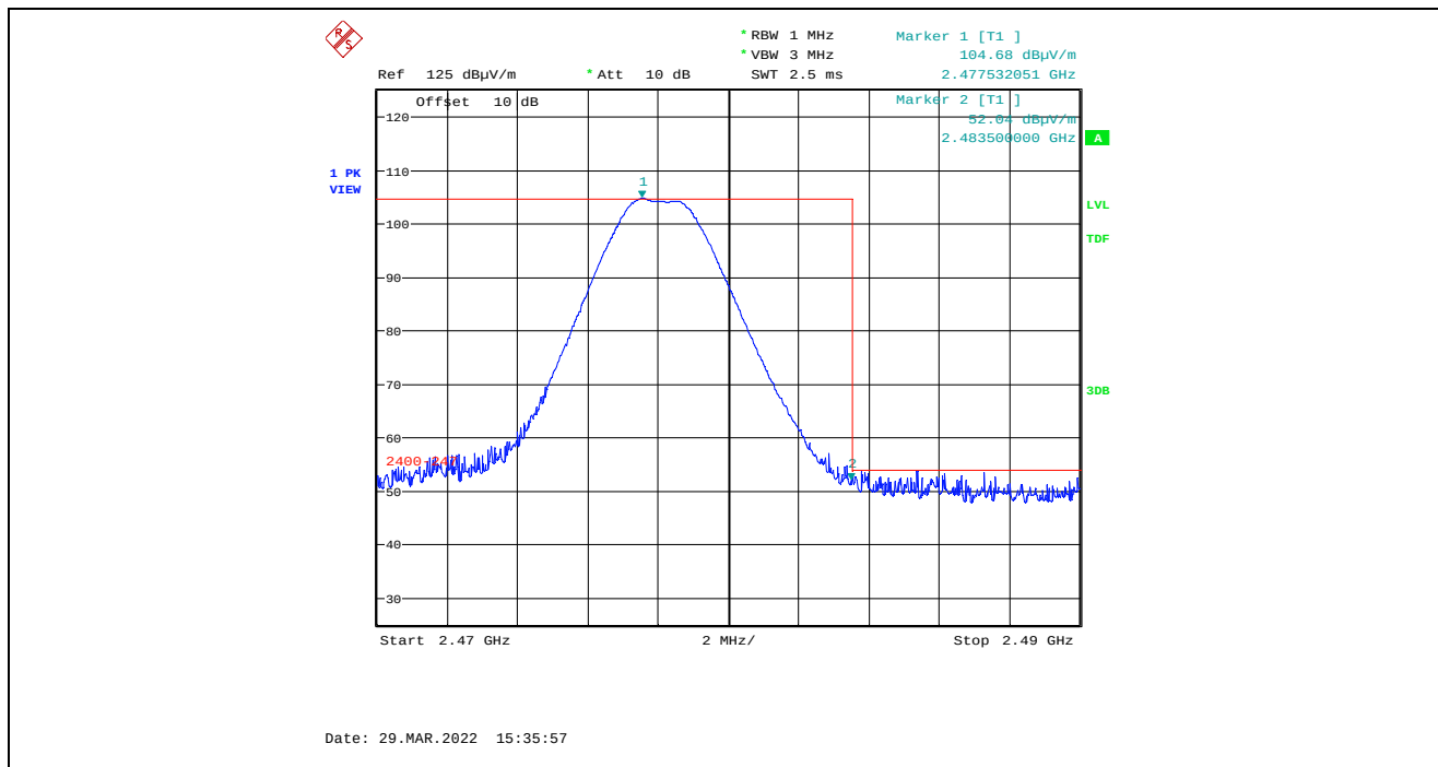
Plot 5.4.4.5.2.7. Band-Edge RF Radiated Emissions at 3 m, Horizontal Polarization, Peak High End of Frequency Band, 2478 MHz, 8 dBm Power Setting, 2 Mbps
