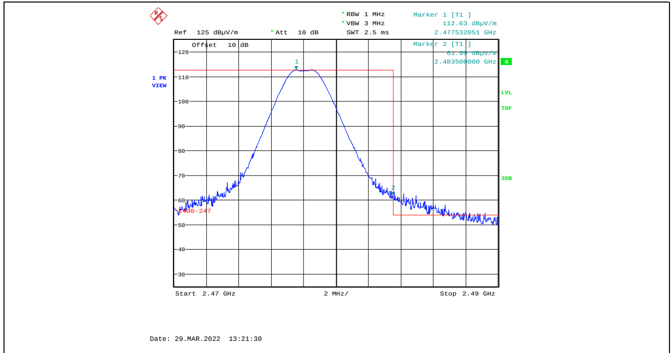
Plot 5.4.4.6.2.5. Band-Edge RF Radiated Emissions at 3 m, Vertical Polarization, Peak High End of Frequency Band, 2478 MHz, 8 dBm Power Setting, 2 Mbps
