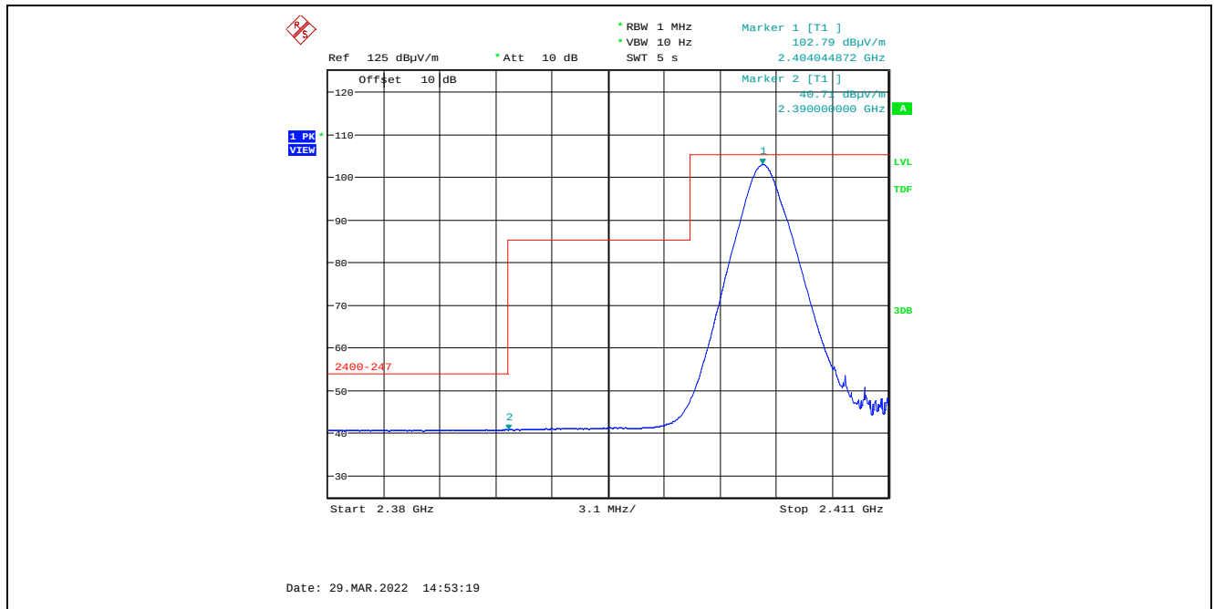
Plot 5.4.4.5.2.2. Band-Edge RF Radiated Emissions at 3 m, Vertical Polarization, Average Low End of Frequency Band, 2404 MHz, 8 dBm Power Setting, 2 Mbps
