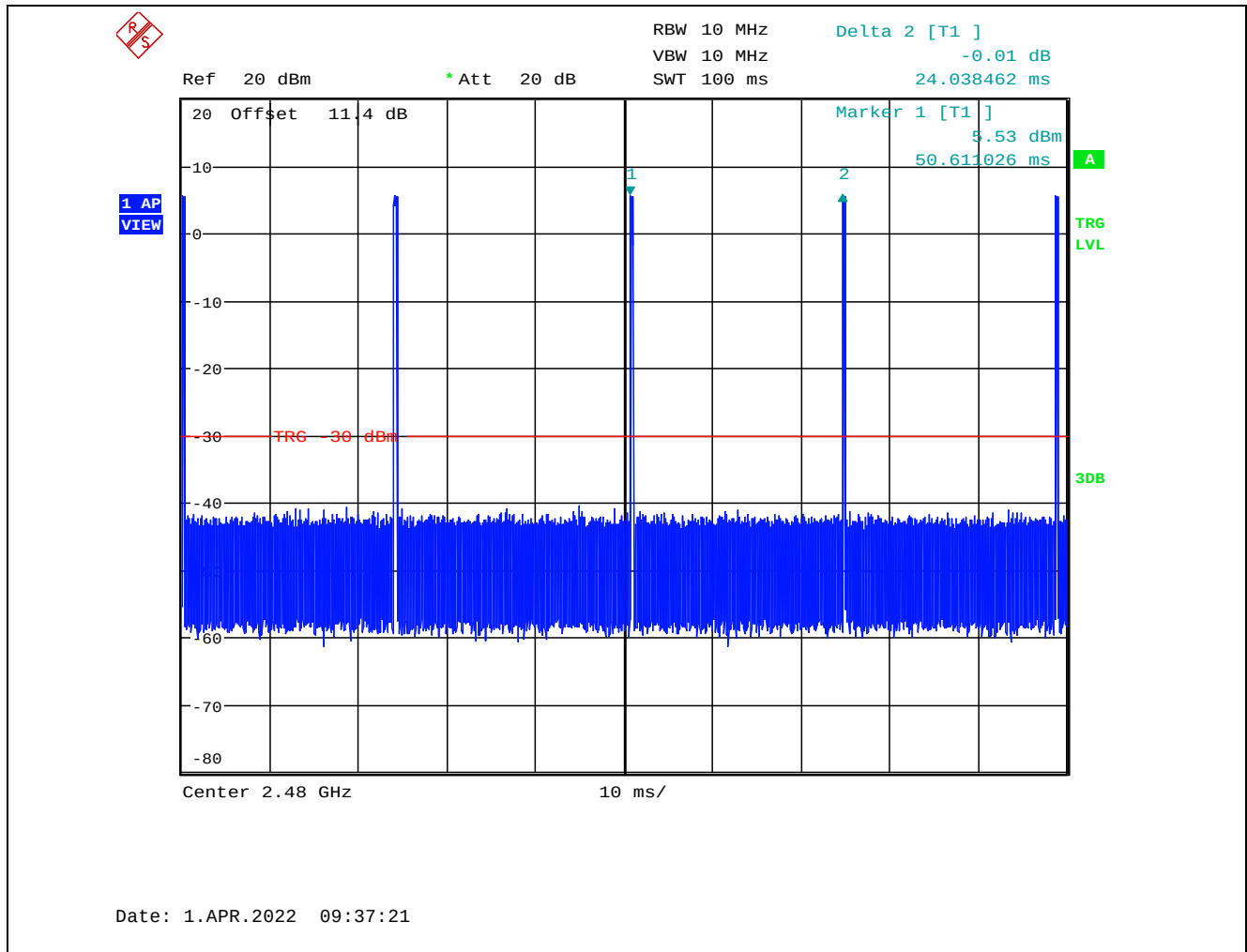
Plot 5.7.4.1.2. Duty Cycle (5 Pulses in 100 ms)
