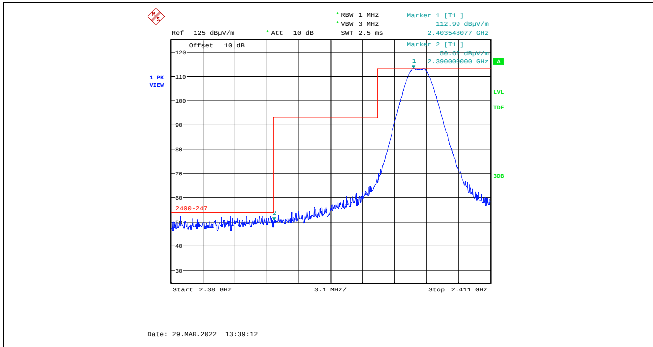
Plot 5.4.4.6.2.3. Band-Edge RF Radiated Emissions at 3 m, Horizontal Polarization, Peak Low End of Frequency Band, 2404 MHz, 8 dBm Power Setting, 2 Mbps
