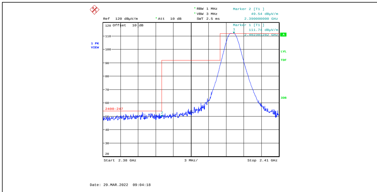
Plot 5.4.4.3.2.1. Band-Edge RF Radiated Emissions at 3 m, Vertical Polarization, Peak Low End of Frequency Band, 2402 MHz, 8 dBm Power Setting, 1 Mbps
