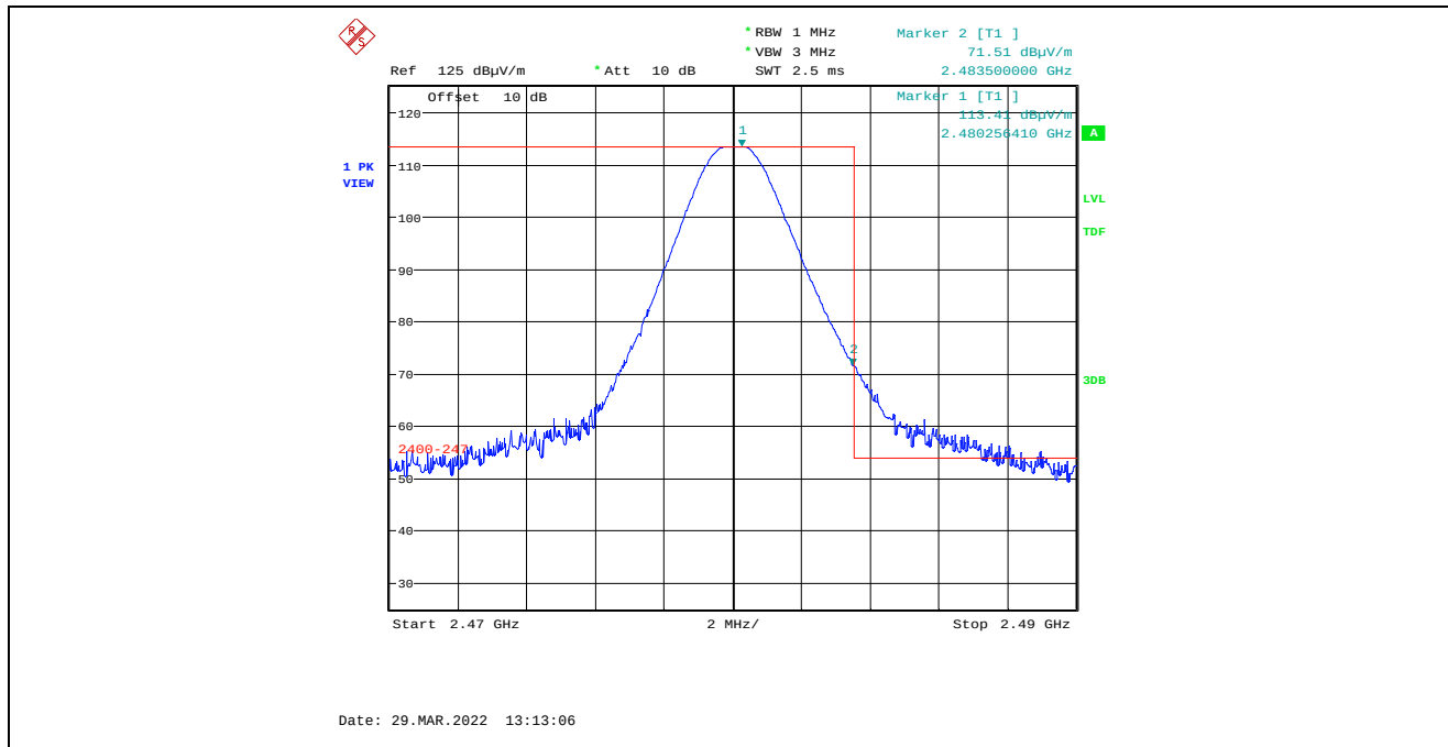
Plot 5.4.4.2.2.5. Band-Edge RF Radiated Emissions at 3 m, Vertical Polarization, Peak High End of Frequency Band, 2480 MHz, 8 dBm Power Setting, 1 Mbps
