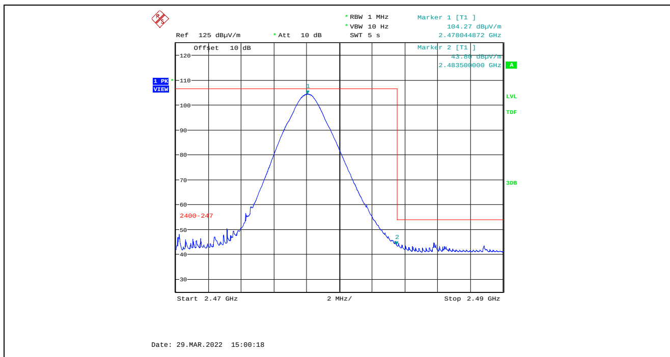
Plot 5.4.4.5.2.6. Band-Edge RF Radiated Emissions at 3 m, Vertical Polarization, Average High End of Frequency Band, 2478 MHz, 8 dBm Power Setting, 2 Mbps
