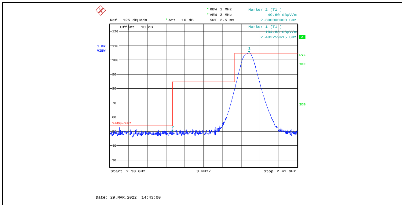
Plot 5.4.4.1.2.1. Band-Edge RF Radiated Emissions at 3 m, Vertical Polarization, Peak Low End of Frequency Band, 2402 MHz, 8 dBm Power Setting, 1 Mbps
