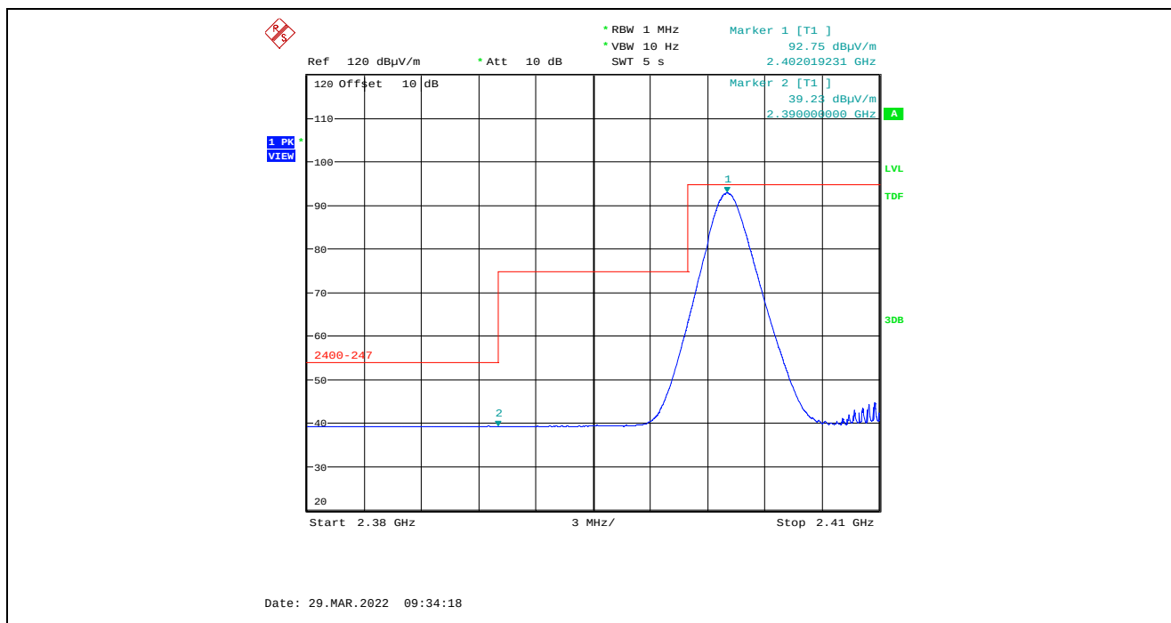
Plot 5.4.4.3.2.4. Band-Edge RF Radiated Emissions at 3 m, Horizontal Polarization, Average Low End of Frequency Band, 2402 MHz, 8 dBm Power Setting, 1 Mbps
