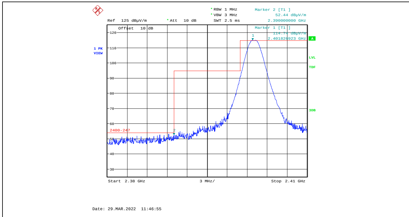
Plot 5.4.4.4.2.3. Band-Edge RF Radiated Emissions at 3 m, Horizontal Polarization, Peak Low End of Frequency Band, 2402 MHz, 8 dBm Power Setting, 1 Mbps
