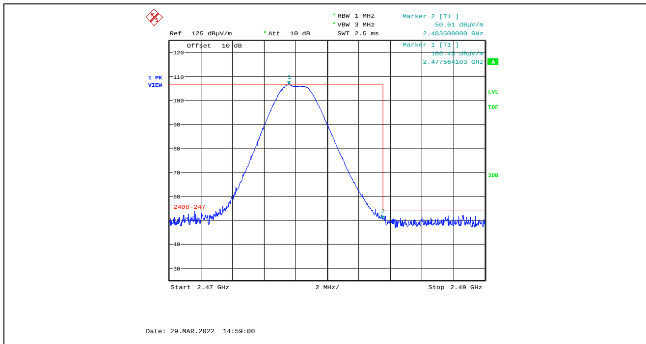
Plot 5.4.4.5.2.5. Band-Edge RF Radiated Emissions at 3 m, Vertical Polarization, Peak High End of Frequency Band, 2478 MHz, 8 dBm Power Setting, 2 Mbps
