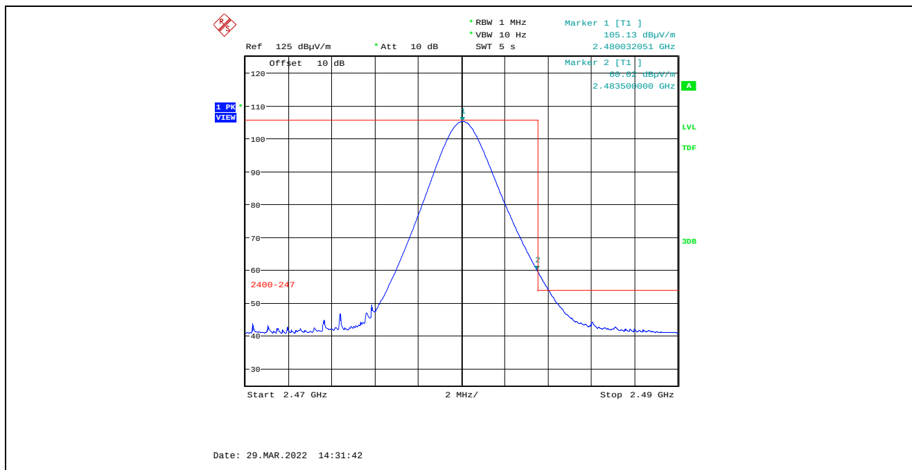
Plot 5.4.4.1.2.6. Band-Edge RF Radiated Emissions at 3 m, Vertical Polarization, Average High End of Frequency Band, 2480 MHz, 8 dBm Power Setting, 1 Mbps Marker 2: 60.02 dBμV/m – 33.51 dB Duty Cycle Factor = 26.51 dBμV/m (Limit 54 dBμV/m)
