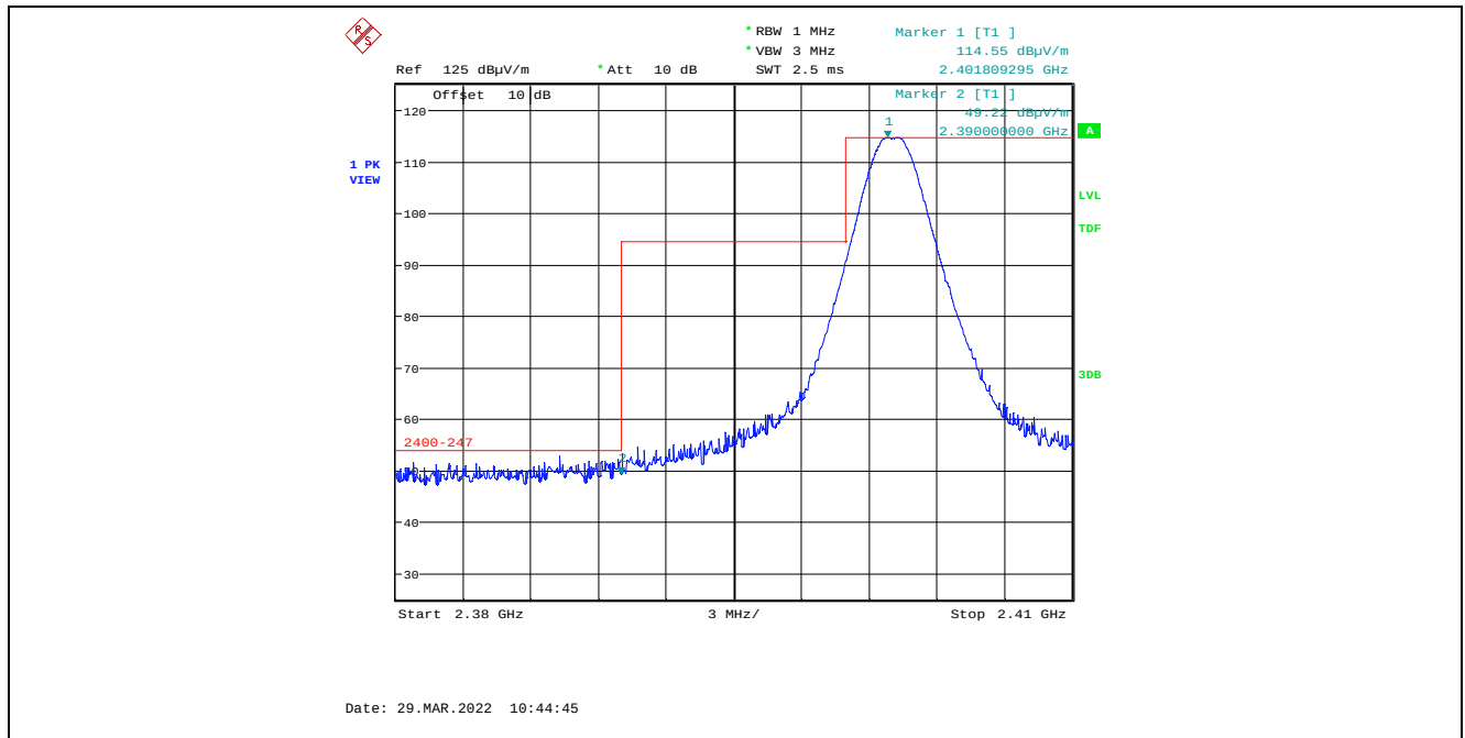
Plot 5.4.4.4.2.1. Band-Edge RF Radiated Emissions at 3 m, Vertical Polarization, Peak Low End of Frequency Band, 2402 MHz, 8 dBm Power Setting, 1 Mbps
