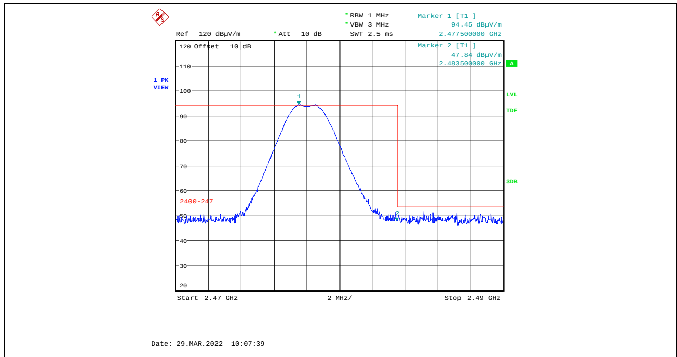
Plot 5.4.4.7.2.7. Band-Edge RF Radiated Emissions at 3 m, Horizontal Polarization, Peak High End of Frequency Band, 2478 MHz, 8 dBm Power Setting, 2 Mbps
