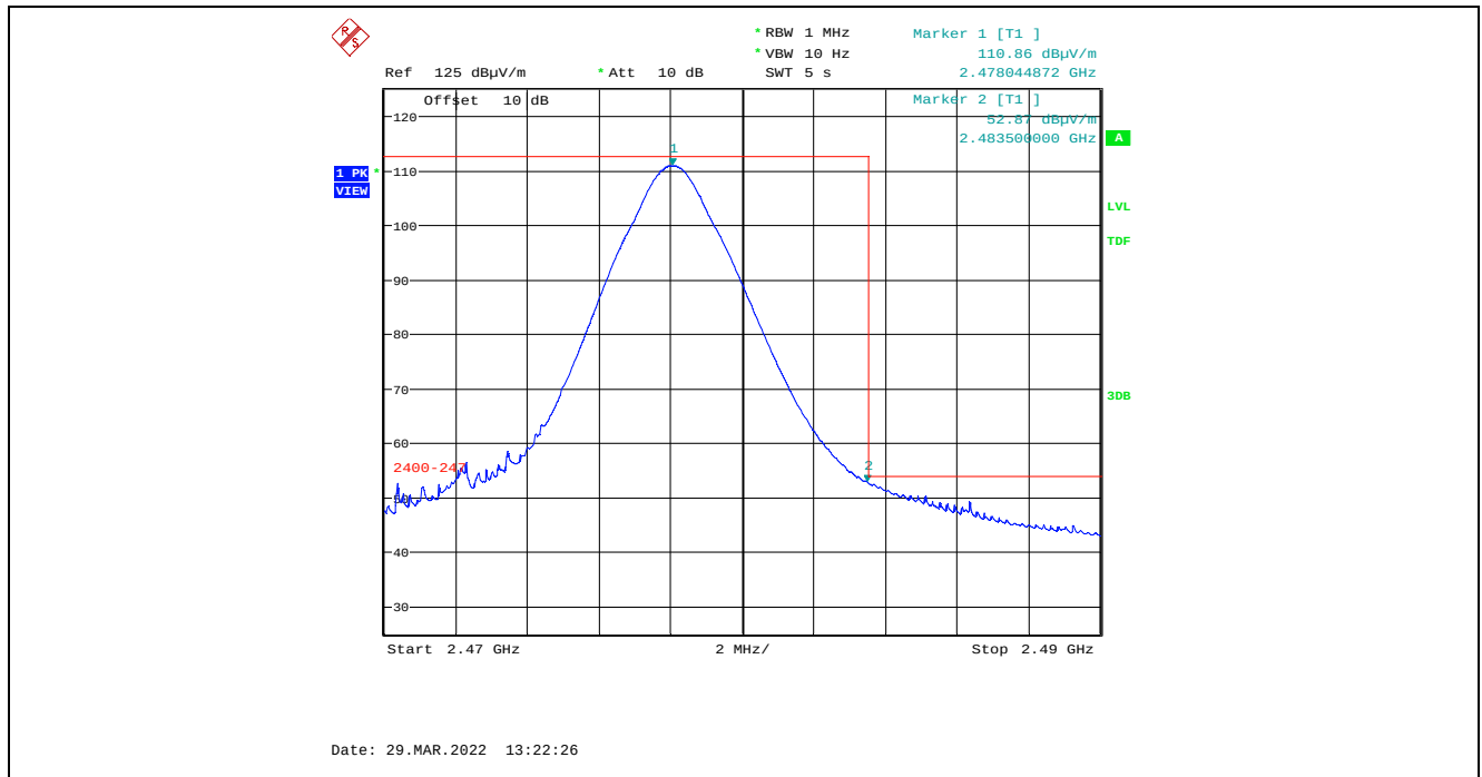
Plot 5.4.4.6.2.6. Band-Edge RF Radiated Emissions at 3 m, Vertical Polarization, Average High End of Frequency Band, 2478 MHz, 8 dBm Power Setting, 2 Mbps
