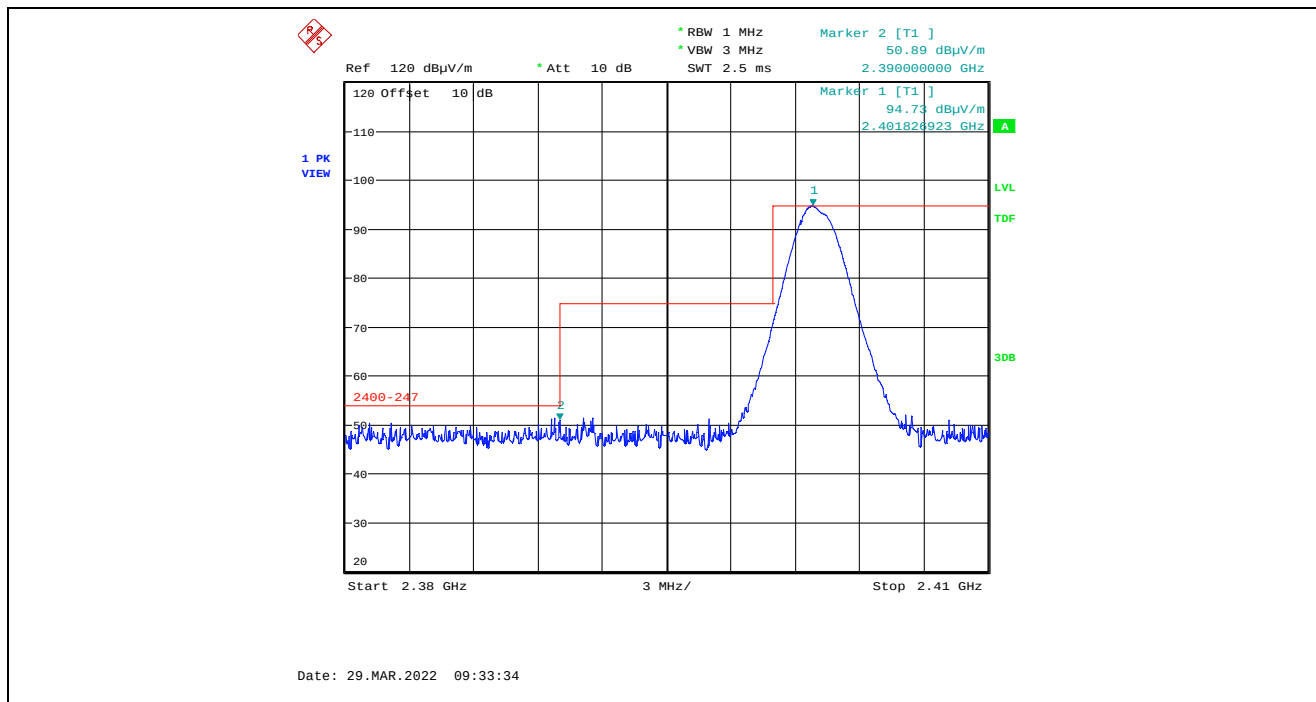
Plot 5.4.4.3.2.3. Band-Edge RF Radiated Emissions at 3 m, Horizontal Polarization, Peak Low End of Frequency Band, 2402 MHz, 8 dBm Power Setting, 1 Mbps
