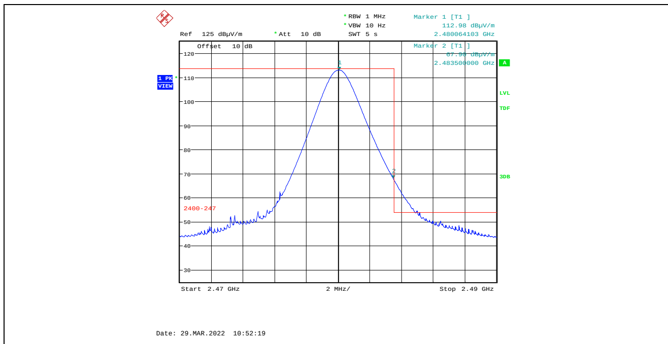
Plot 5.4.4.4.2.6. Band-Edge RF Radiated Emissions at 3 m, Vertical Polarization, Average High End of Frequency Band, 2480 MHz, 8 dBm Power Setting, 1 Mbps Marker 2: 67.90 dBμV/m – 33.51 dB Duty Cycle Factor = 34.39 dBμV/m (Limit 54 dBμV/m)
