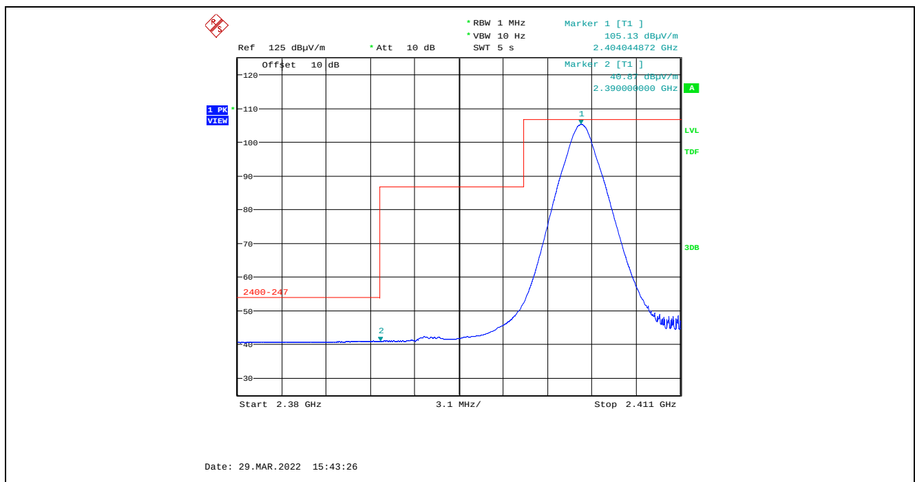
Plot 5.4.4.5.2.4. Band-Edge RF Radiated Emissions at 3 m, Horizontal Polarization, Average Low End of Frequency Band, 2404 MHz, 8 dBm Power Setting, 2 Mbps
