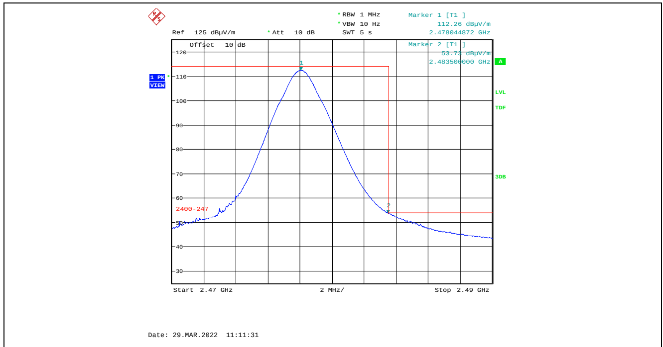
Plot 5.4.4.8.2.6. Band-Edge RF Radiated Emissions at 3 m, Vertical Polarization, Average High End of Frequency Band, 2478 MHz, 8 dBm Power Setting, 2 Mbps
