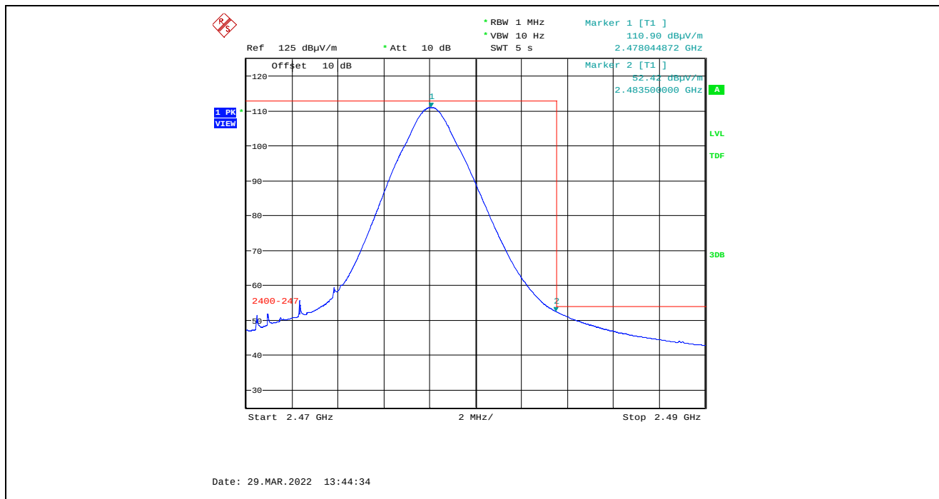
Plot 5.4.4.6.2.8. Band-Edge RF Radiated Emissions at 3 m, Horizontal Polarization, Average High End of Frequency Band, 2478 MHz, 8 dBm Power Setting, 2 Mbps
