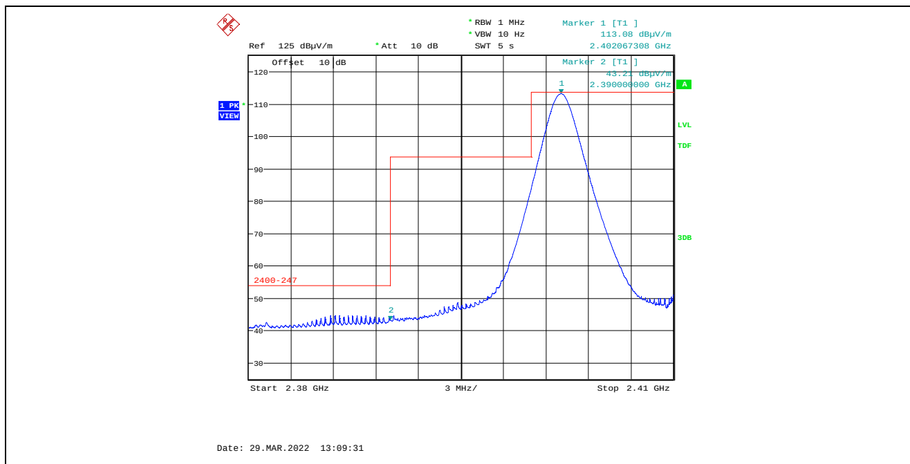
Plot 5.4.4.2.2.2. Band-Edge RF Radiated Emissions at 3 m, Vertical Polarization, Average Low End of Frequency Band, 2402 MHz, 8 dBm Power Setting, 1 Mbps
