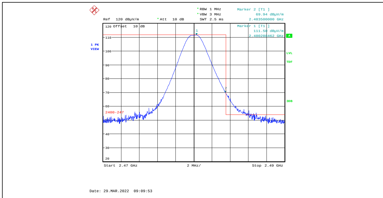
Plot 5.4.4.3.2.5. Band-Edge RF Radiated Emissions at 3 m, Vertical Polarization, Peak High End of Frequency Band, 2480 MHz, 8 dBm Power Setting, 1 Mbps
