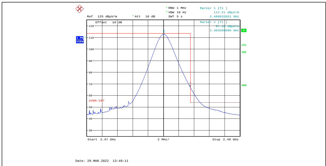
Plot 5.4.4.2.8. Band-Edge RF Radiated Emissions at 3 m, Horizontal Polarization, Average High End of Frequency Band, 2480 MHz, 8 dBm Power Setting, 1 Mbps Marker 2: 67.28 dBμV/m – 33.51 dB Duty Cycle Factor = 33.77 dBμV/m (Limit 54 dBμV/m)
