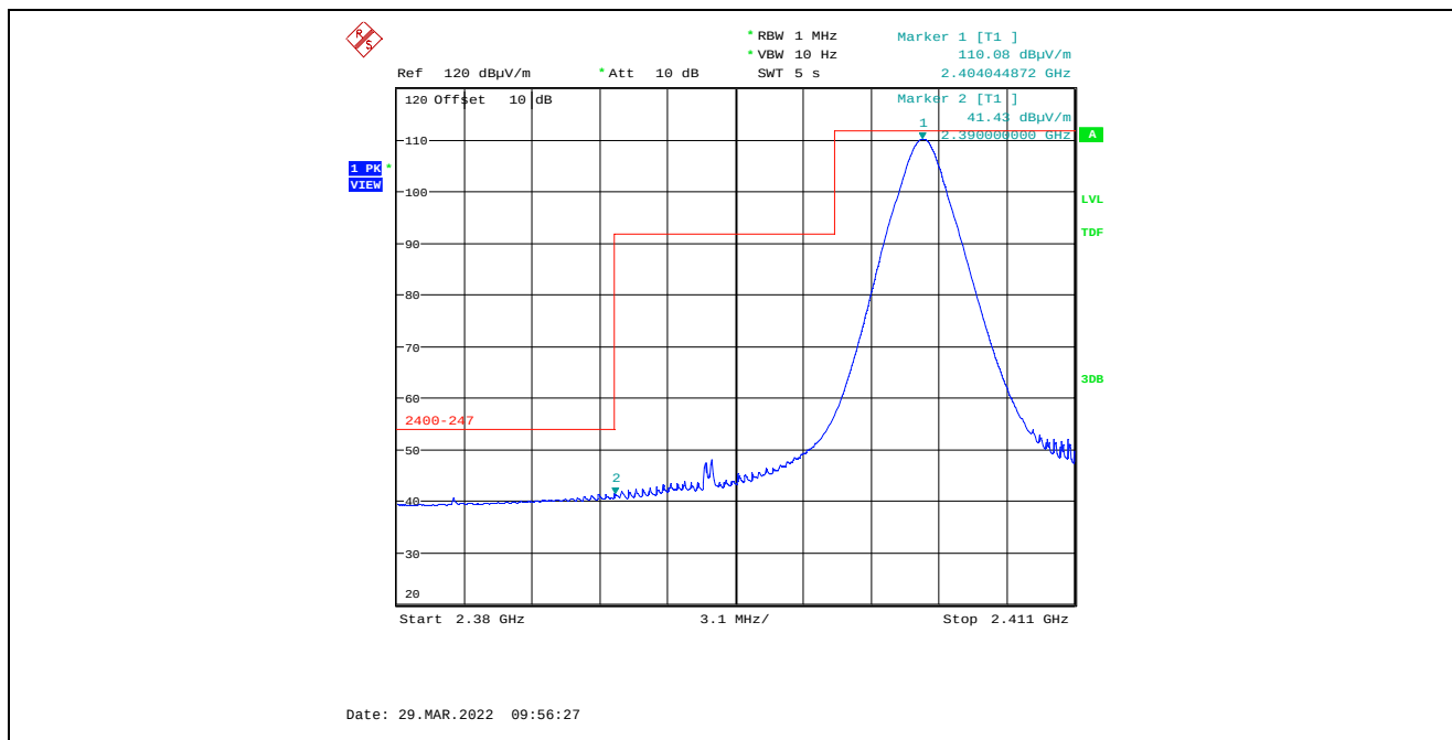
Plot 5.4.4.7.2.2. Band-Edge RF Radiated Emissions at 3 m, Vertical Polarization, Average Low End of Frequency Band, 2404 MHz, 8 dBm Power Setting, 2 Mbps
