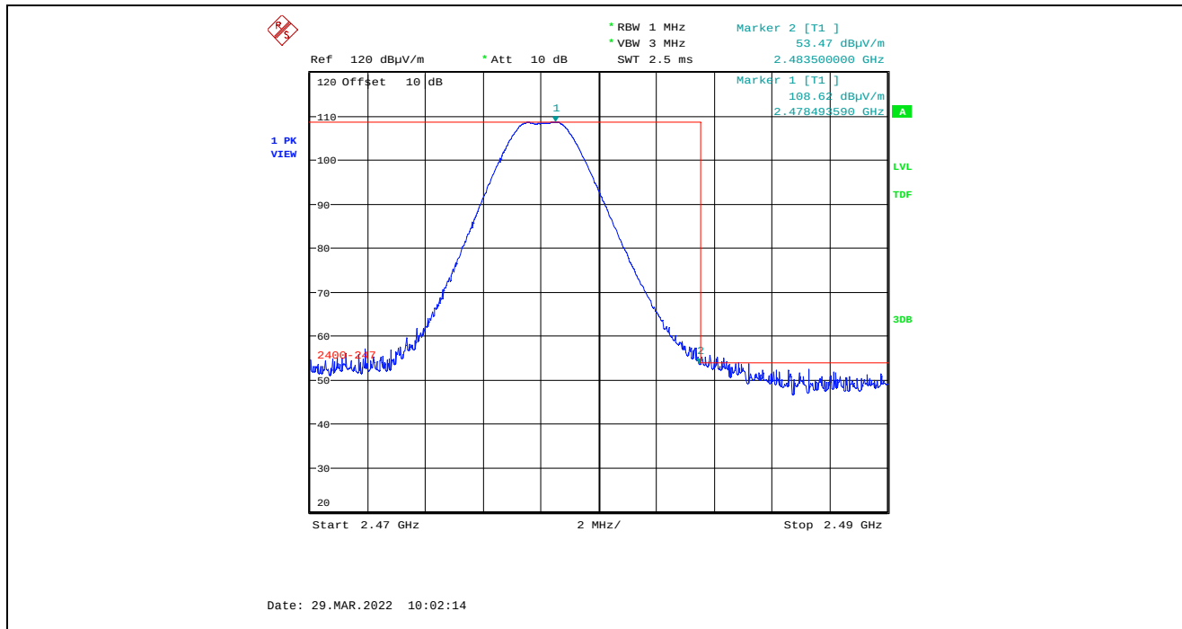
Plot 5.4.4.7.2.5. Band-Edge RF Radiated Emissions at 3 m, Vertical Polarization, Peak High End of Frequency Band, 2478 MHz, 8 dBm Power Setting, 2 Mbps
