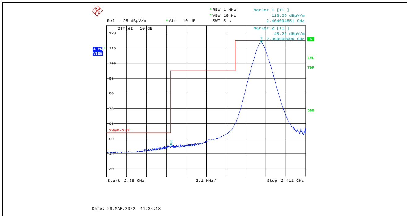
Plot 5.4.4.8.2.4. Band-Edge RF Radiated Emissions at 3 m, Horizontal Polarization, Average Low End of Frequency Band, 2404 MHz, 8 dBm Power Setting, 2 Mbps
