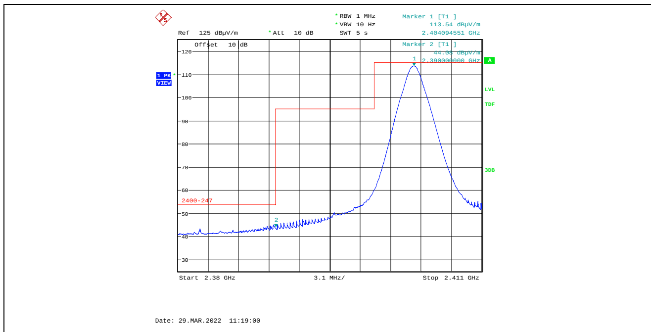
Plot 5.4.4.8.2.2. Band-Edge RF Radiated Emissions at 3 m, Vertical Polarization, Average Low End of Frequency Band, 2404 MHz, 8 dBm Power Setting, 2 Mbps
