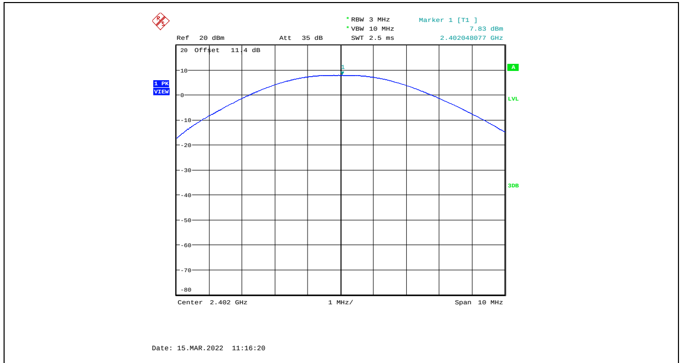
Plot 5.3.4.1. Maximum Peak Conducted Output Power, GFSK Modulation, 1 Mbps, 8 dBm Power Setting, 2402 MHz
