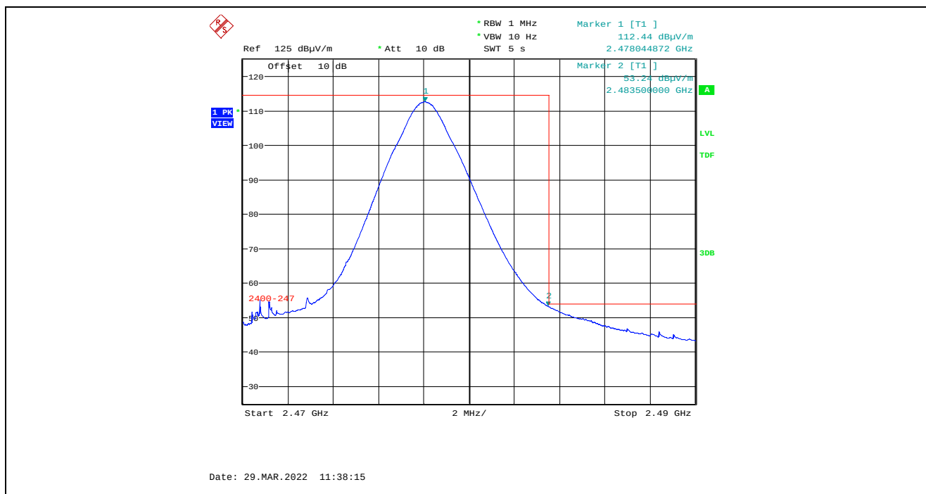
Plot 5.4.4.8.2.8. Band-Edge RF Radiated Emissions at 3 m, Horizontal Polarization, Average High End of Frequency Band, 2478 MHz, 8 dBm Power Setting, 2 Mbps
