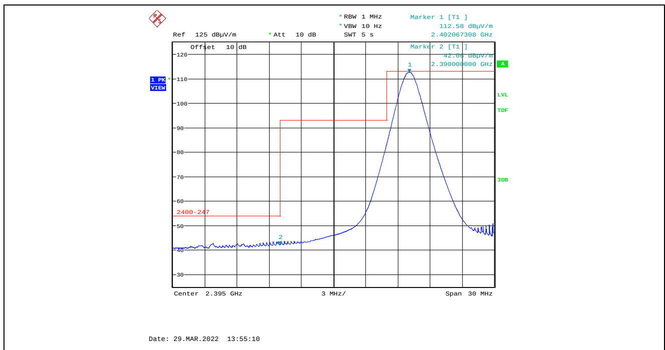
Plot 5.4.4.2.2.4. Band-Edge RF Radiated Emissions at 3 m, Horizontal Polarization, Average Low End of Frequency Band, 2402 MHz, 8 dBm Power Setting, 1 Mbps
