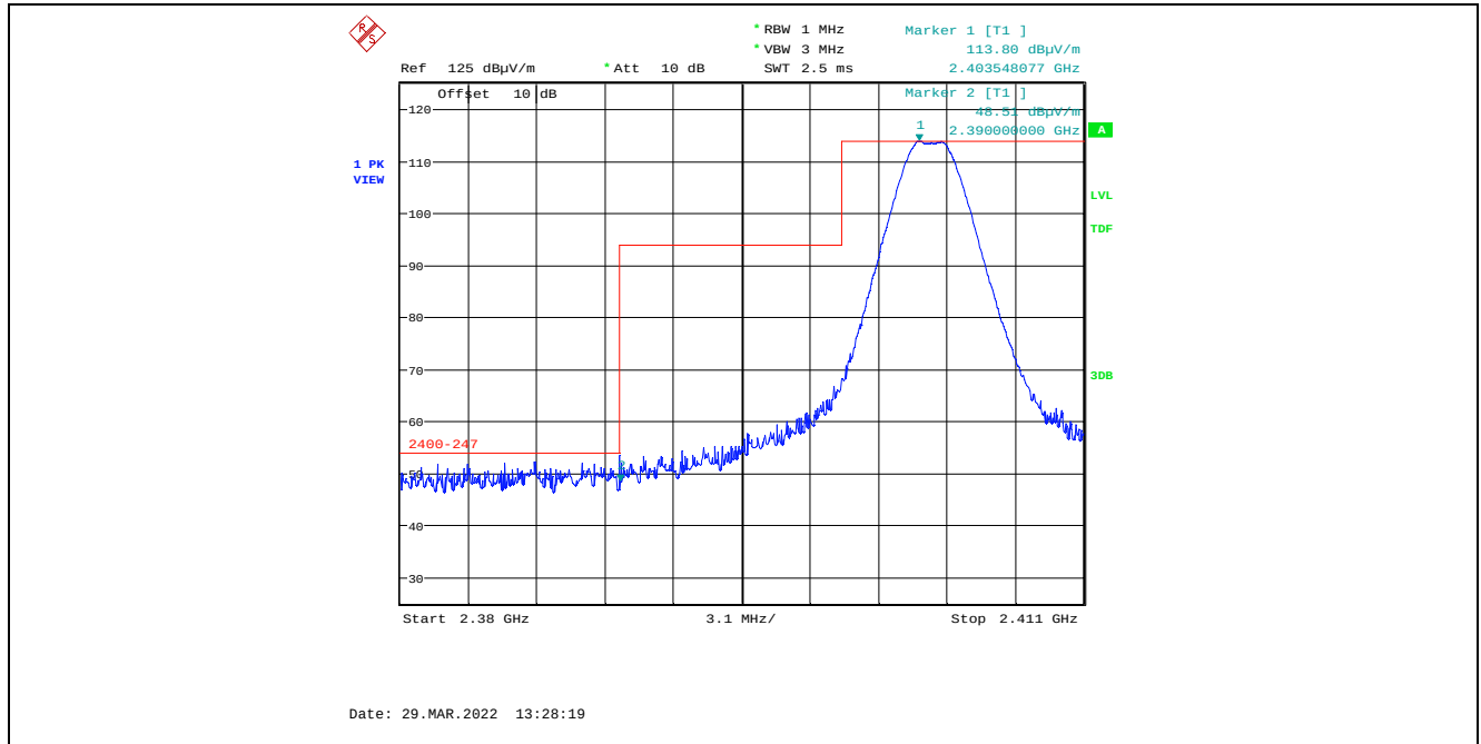
Plot 5.4.4.6.2.1. Band-Edge RF Radiated Emissions at 3 m, Vertical Polarization, Peak Low End of Frequency Band, 2404 MHz, 8 dBm Power Setting, 2 Mbps
