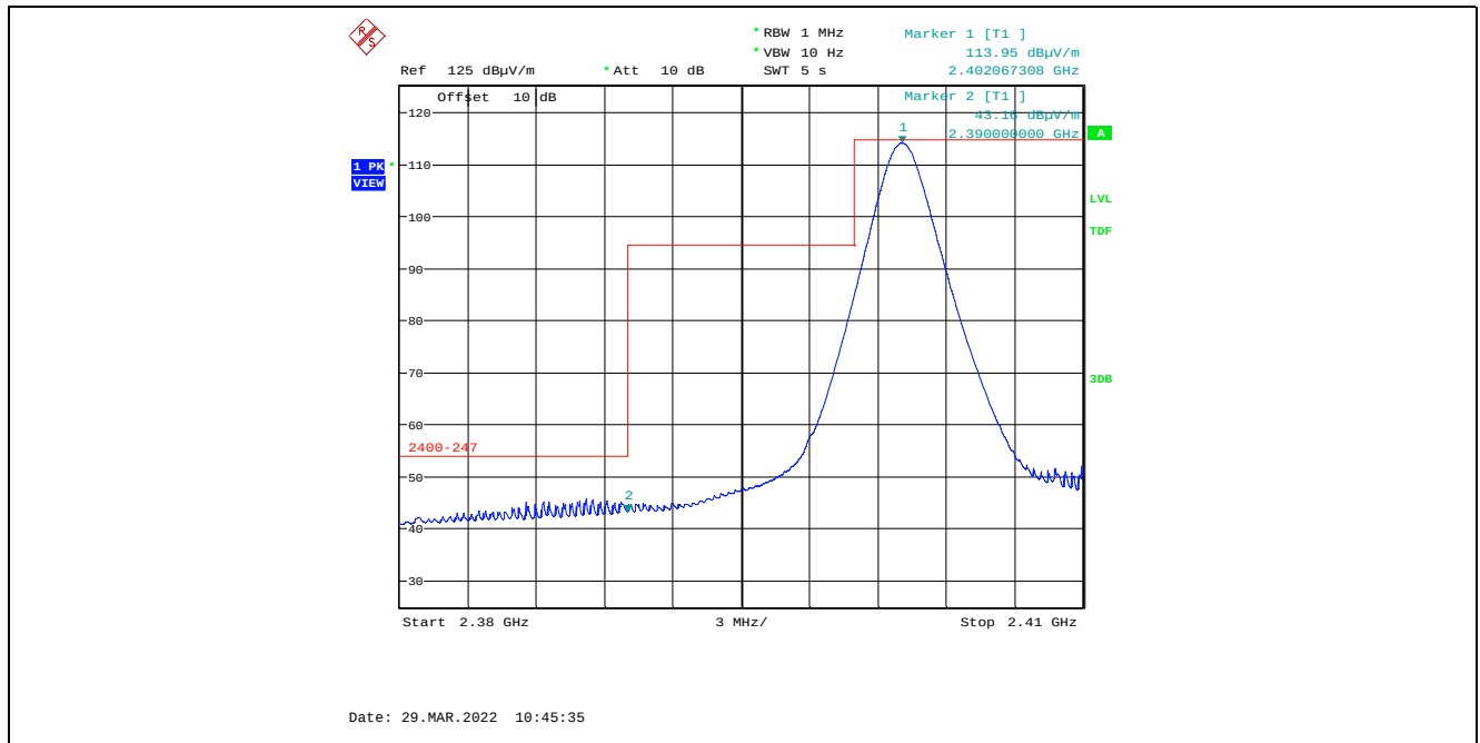
Plot 5.4.4.4.2.2. Band-Edge RF Radiated Emissions at 3 m, Vertical Polarization, Average Low End of Frequency Band, 2402 MHz, 8 dBm Power Setting, 1 Mbps
