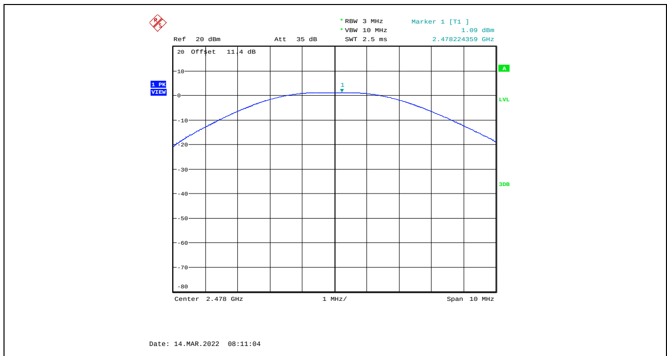
Plot 5.3.4.12. Maximum Peak Conducted Output Power, GFSK Modulation, 2 Mbps, -2 dBm Power Setting, 2478 MHz
