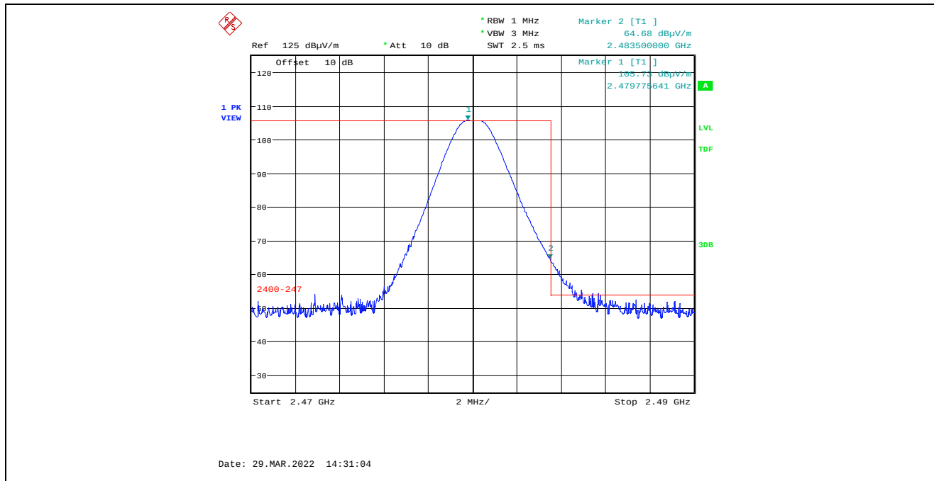
Plot 5.4.4.1.2.5. Band-Edge RF Radiated Emissions at 3 m, Vertical Polarization, Peak High End of Frequency Band, 2480 MHz, 8 dBm Power Setting, 1 Mbps
