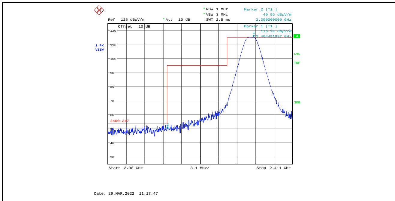
Plot 5.4.4.8.2.1. Band-Edge RF Radiated Emissions at 3 m, Vertical Polarization, Peak Low End of Frequency Band, 2404 MHz, 8 dBm Power Setting, 2 Mbps
