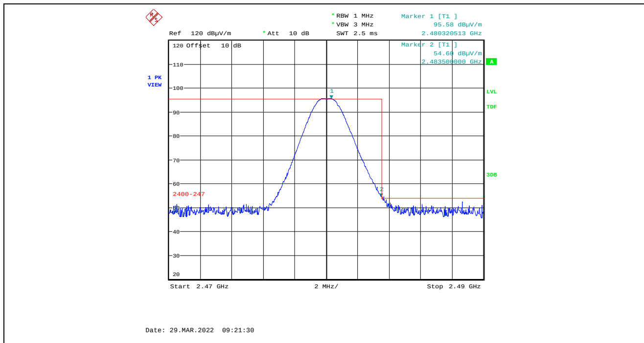
Plot 5.4.4.3.2.7. Band-Edge RF Radiated Emissions at 3 m, Horizontal Polarization, Peak High End of Frequency Band, 2480 MHz, 8 dBm Power Setting, 1 Mbps
