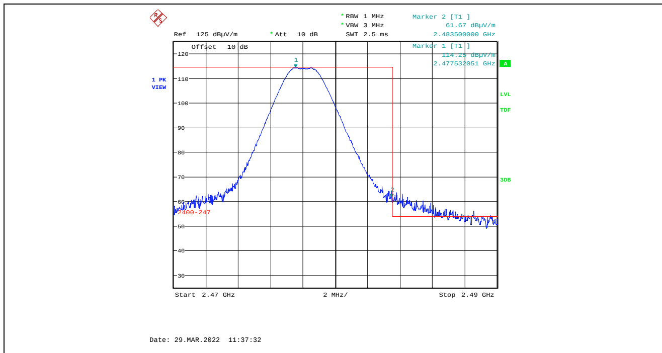
Plot 5.4.4.8.2.7. Band-Edge RF Radiated Emissions at 3 m, Horizontal Polarization, Peak High End of Frequency Band, 2478 MHz, 8 dBm Power Setting, 2 Mbps
