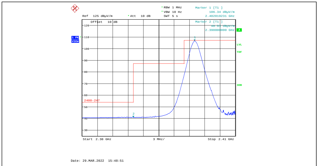
Plot 5.4.4.1.2.4. Band-Edge RF Radiated Emissions at 3 m, Horizontal Polarization, Average Low End of Frequency Band, 2402 MHz, 8 dBm Power Setting, 1 Mbps
