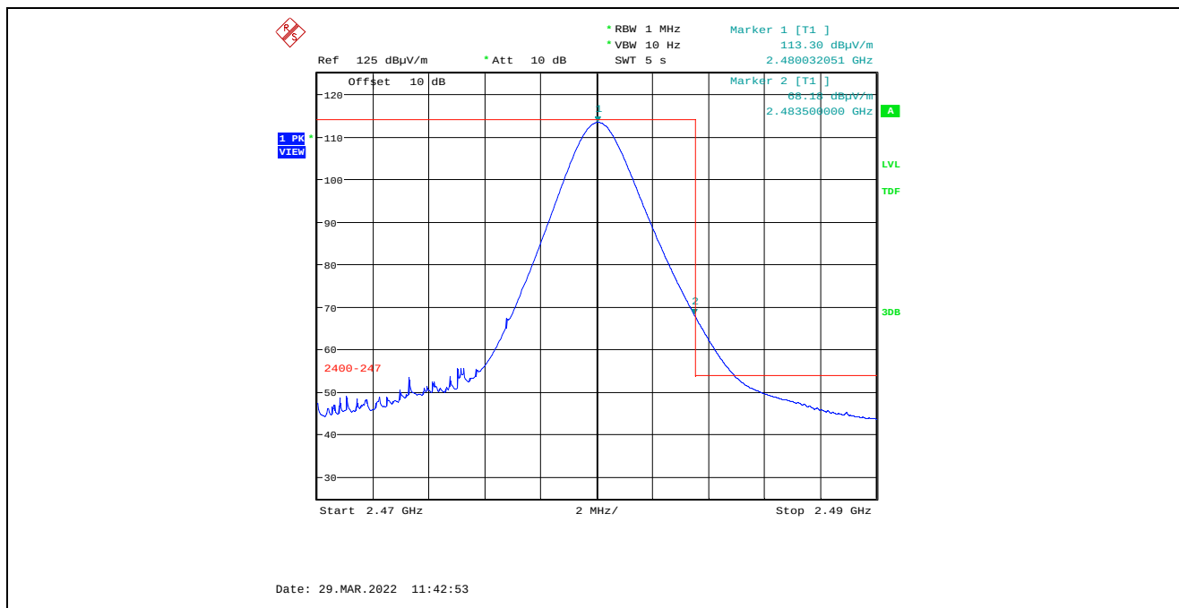
Plot 5.4.4.4.2.8. Band-Edge RF Radiated Emissions at 3 m, Horizontal Polarization, Average High End of Frequency Band, 2480 MHz, 8 dBm Power Setting, 1 Mbps Marker 2: 68.18 dBμV/m – 33.51 dB Duty Cycle Factor = 34.67 dBμV/m (Limit 54 dBμV/m)
