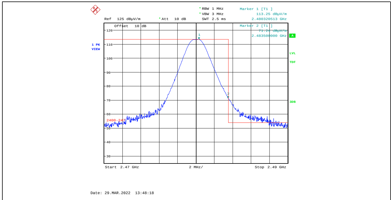
Plot 5.4.4.2.7. Band-Edge RF Radiated Emissions at 3 m, Horizontal Polarization, Peak High End of Frequency Band, 2480 MHz, 8 dBm Power Setting, 1 Mbps
