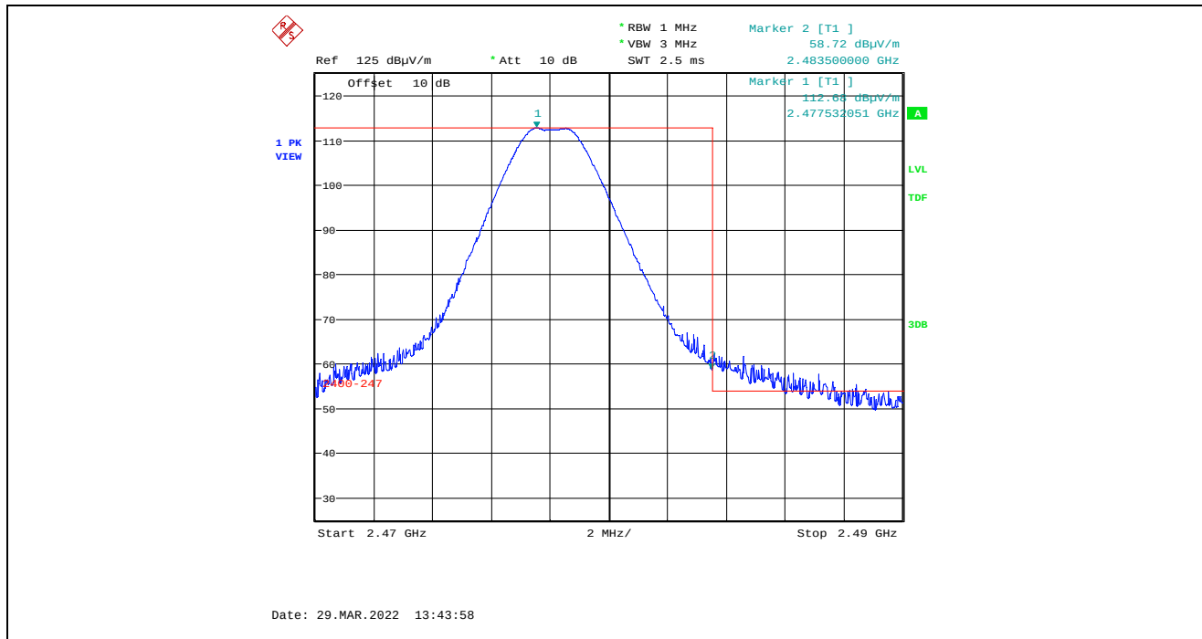
Plot 5.4.4.6.2.7. Band-Edge RF Radiated Emissions at 3 m, Horizontal Polarization, Peak High End of Frequency Band, 2478 MHz, 8 dBm Power Setting, 2 Mbps
