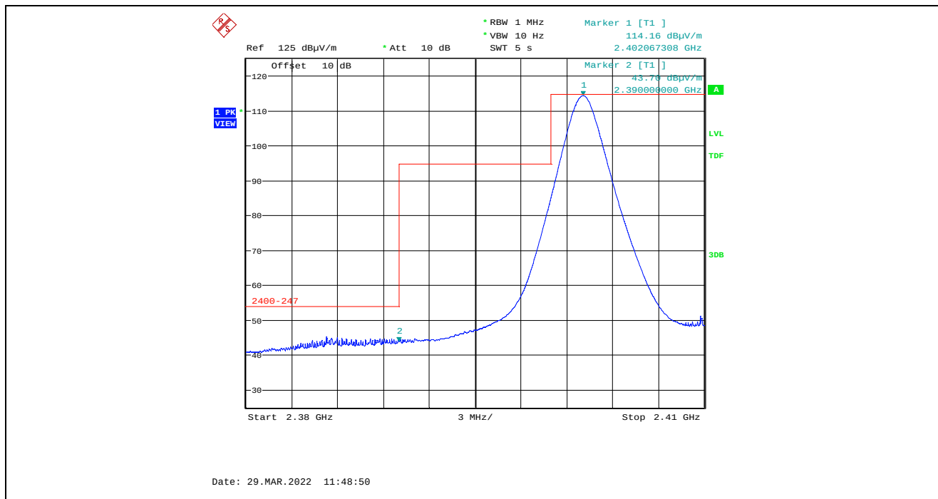
Plot 5.4.4.4.2.4. Band-Edge RF Radiated Emissions at 3 m, Horizontal Polarization, Average Low End of Frequency Band, 2402 MHz, 8 dBm Power Setting, 1 Mbps
