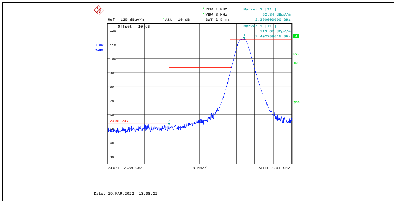
Plot 5.4.4.2.2.1. Band-Edge RF Radiated Emissions at 3 m, Vertical Polarization, Peak Low End of Frequency Band, 2402 MHz, 8 dBm Power Setting, 1 Mbps
