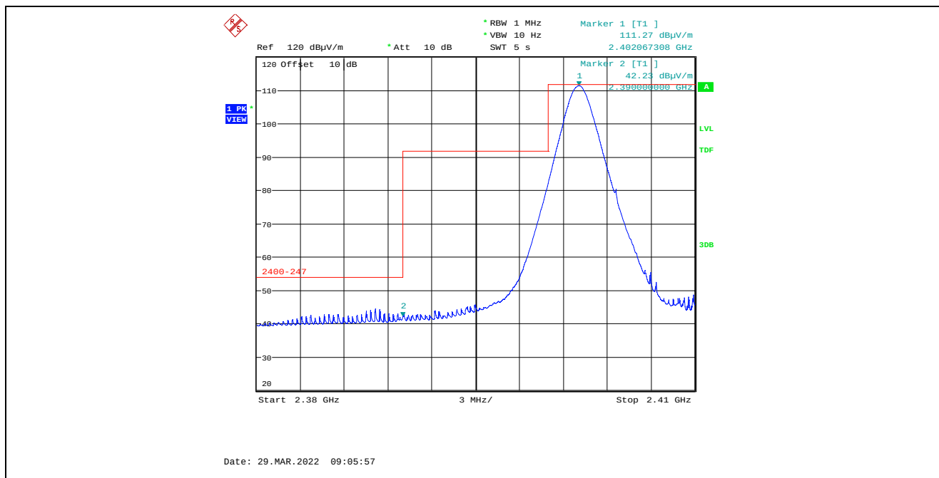
Plot 5.4.4.3.2.2. Band-Edge RF Radiated Emissions at 3 m, Vertical Polarization, Average Low End of Frequency Band, 2402 MHz, 8 dBm Power Setting, 1 Mbps
