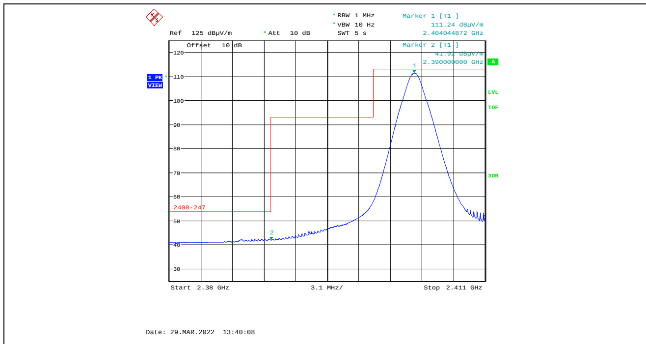
Plot 5.4.4.6.2.4. Band-Edge RF Radiated Emissions at 3 m, Horizontal Polarization, Average Low End of Frequency Band, 2404 MHz, 8 dBm Power Setting, 2 Mbps
