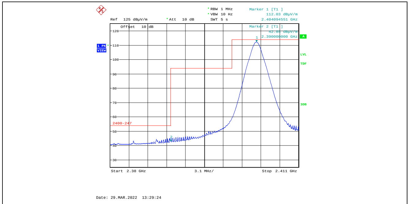
Plot 5.4.4.6.2.2. Band-Edge RF Radiated Emissions at 3 m, Vertical Polarization, Average Low End of Frequency Band, 2404 MHz, 8 dBm Power Setting, 2 Mbps
