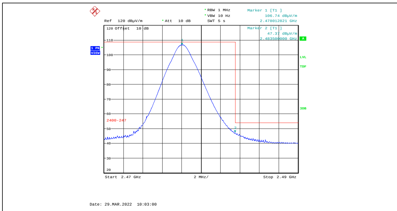
Plot 5.4.4.7.2.6. Band-Edge RF Radiated Emissions at 3 m, Vertical Polarization, Average High End of Frequency Band, 2478 MHz, 8 dBm Power Setting, 2 Mbps
