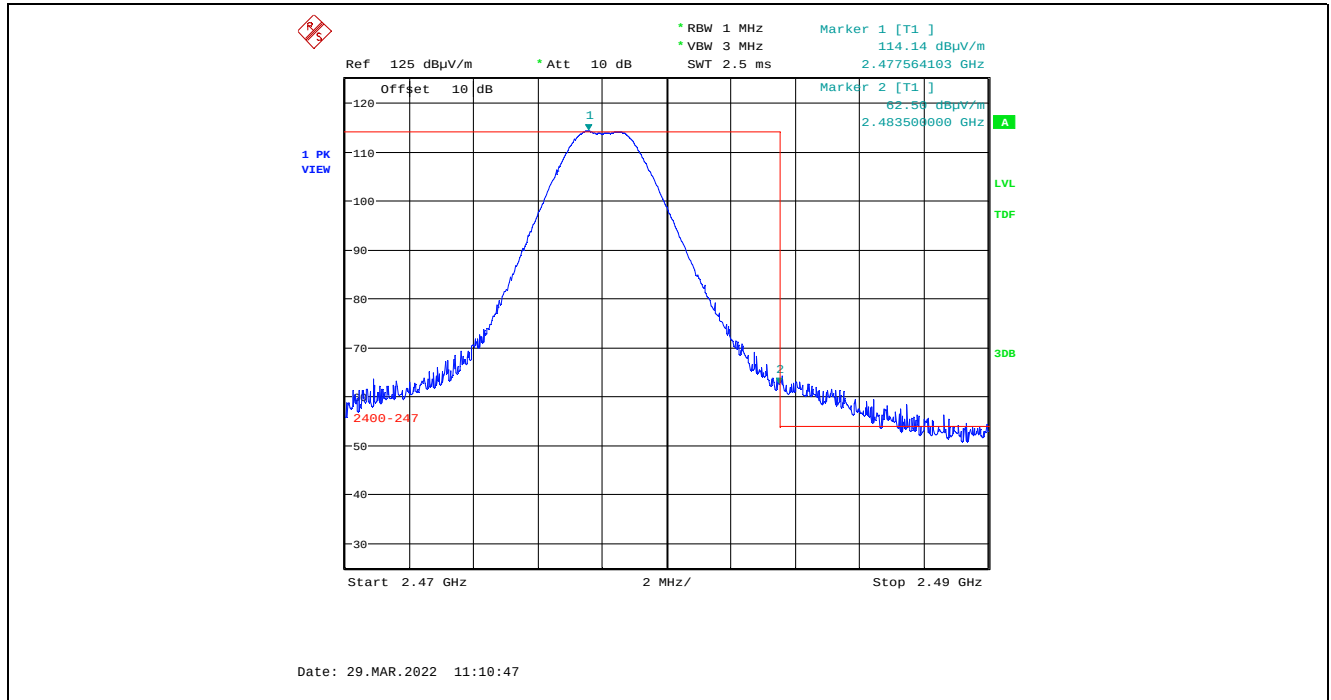
Plot 5.4.4.8.2.5. Band-Edge RF Radiated Emissions at 3 m, Vertical Polarization, Peak High End of Frequency Band, 2478 MHz, 8 dBm Power Setting, 2 Mbps
