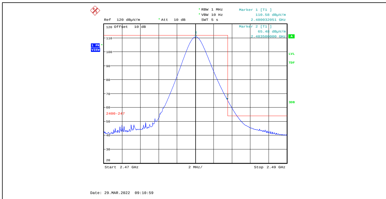
Plot 5.4.4.3.2.6. Band-Edge RF Radiated Emissions at 3 m, Vertical Polarization, Average High End of Frequency Band, 2480 MHz, 8 dBm Power Setting, 1 Mbps Marker 2: 65.48 dBμV/m – 33.51 dB Duty Cycle Factor = 31.97 dBμV/m (Limit 54 dBμV/m)
