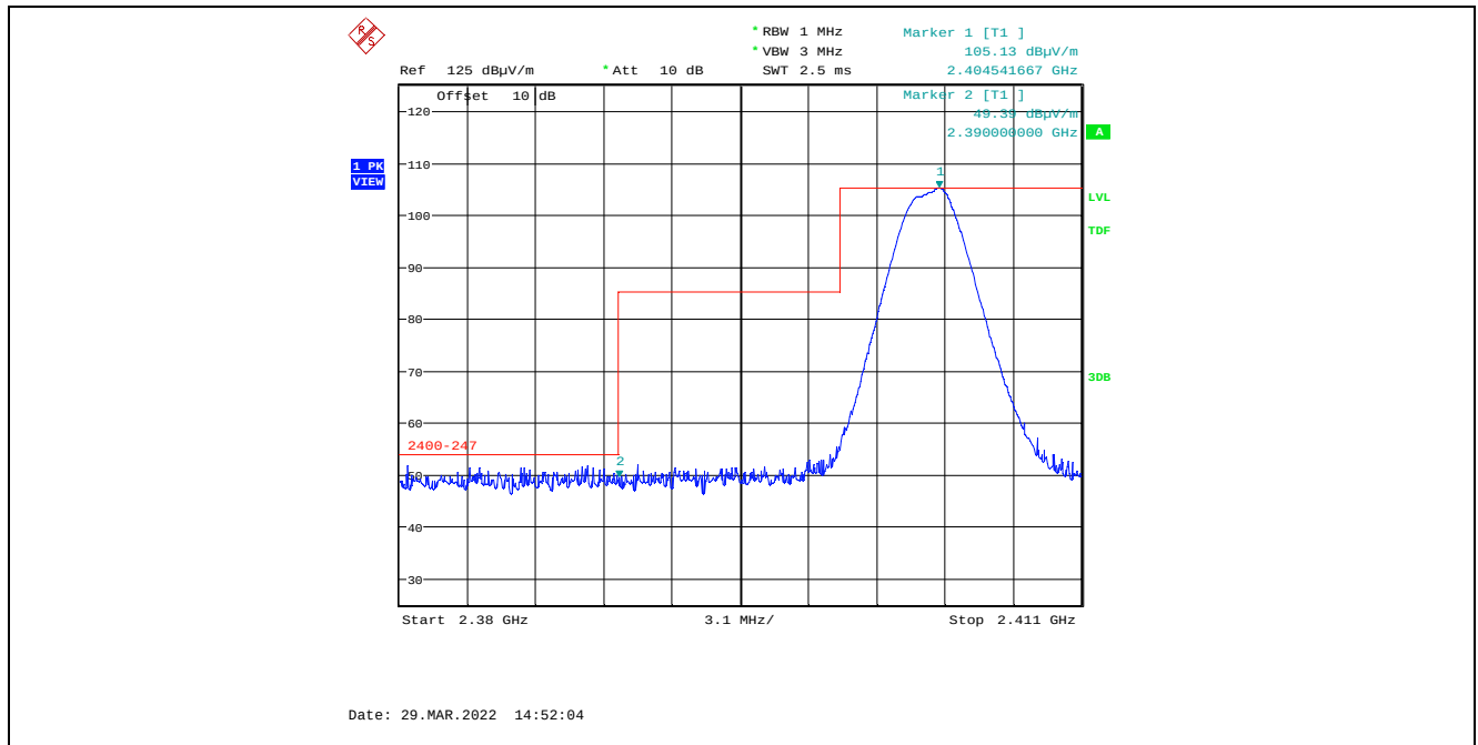
Plot 5.4.4.5.2.1. Band-Edge RF Radiated Emissions at 3 m, Vertical Polarization, Peak Low End of Frequency Band, 2404 MHz, 8 dBm Power Setting, 2 Mbps
