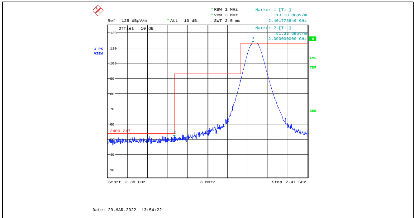
Plot 5.4.4.2.2.3. Band-Edge RF Radiated Emissions at 3 m, Horizontal Polarization, Peak Low End of Frequency Band, 2402 MHz, 8 dBm Power Setting, 1 Mbps
