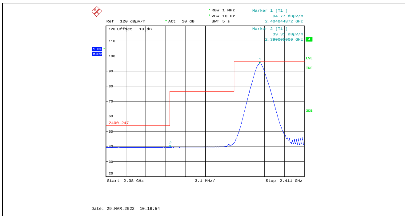
Plot 5.4.4.7.2.4. Band-Edge RF Radiated Emissions at 3 m, Horizontal Polarization, Average Low End of Frequency Band, 2404 MHz, 8 dBm Power Setting, 2 Mbps
