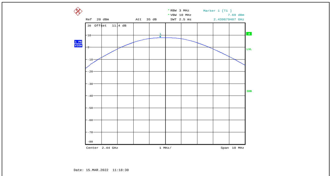
Plot 5.3.4.2. Maximum Peak Conducted Output Power, GFSK Modulation, 1 Mbps, 8 dBm Power Setting, 2440 MHz
