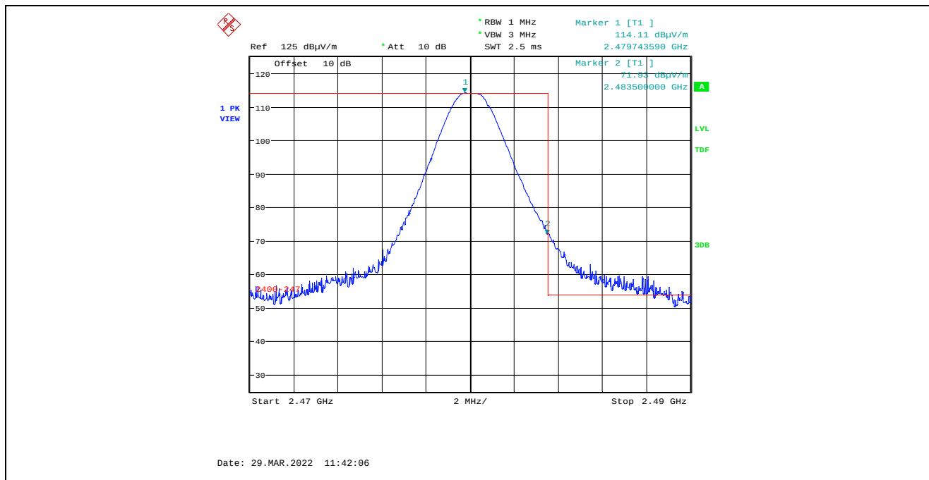
Plot 5.4.4.4.2.7. Band-Edge RF Radiated Emissions at 3 m, Horizontal Polarization, Peak High End of Frequency Band, 2480 MHz, 8 dBm Power Setting, 1 Mbps
