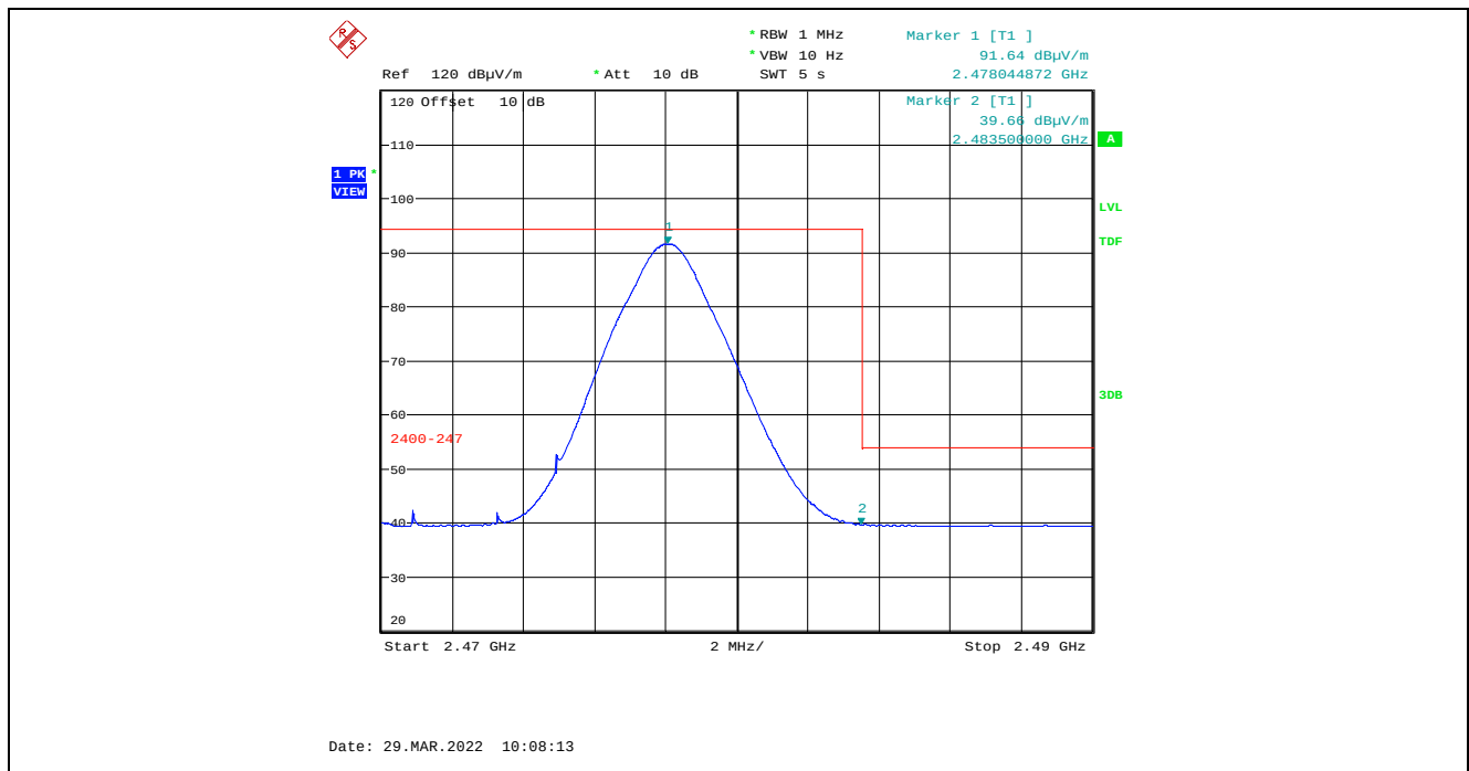
Plot 5.4.4.7.2.8. Band-Edge RF Radiated Emissions at 3 m, Horizontal Polarization, Average High End of Frequency Band, 2478 MHz, 8 dBm Power Setting, 2 Mbps
