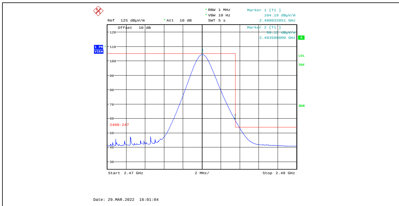
Plot 5.4.4.1.2.8. Band-Edge RF Radiated Emissions at 3 m, Horizontal Polarization, Average High End of Frequency Band, 2480 MHz, 8 dBm Power Setting, 1 Mbps Marker 2: 59.12 dBμV/m – 33.51 dB Duty Cycle Factor = 25.61 dBμV/m (Limit 54 dBμV/m)
