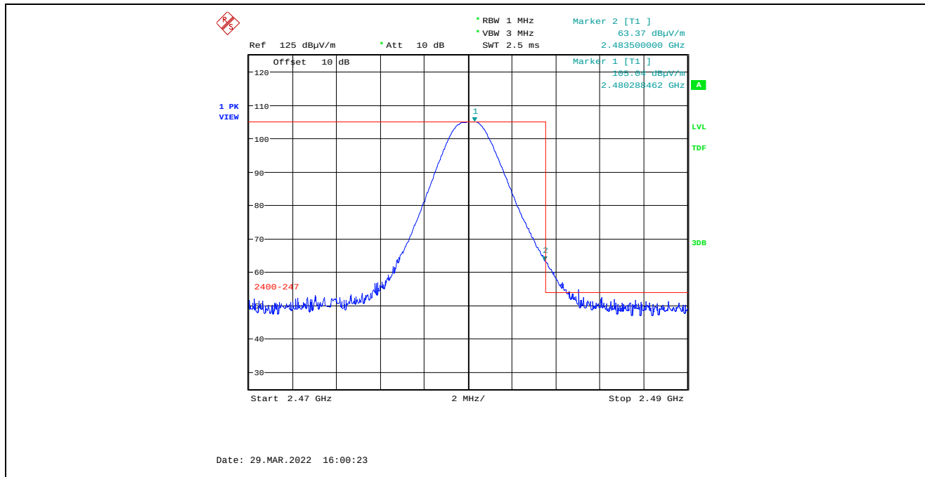
Plot 5.4.4.1.2.7. Band-Edge RF Radiated Emissions at 3 m, Horizontal Polarization, Peak High End of Frequency Band, 2480 MHz, 8 dBm Power Setting, 1 Mbps
