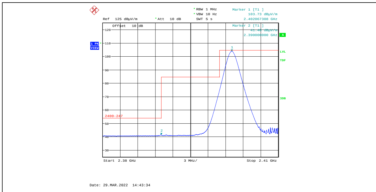
Plot 5.4.4.1.2.2. Band-Edge RF Radiated Emissions at 3 m, Vertical Polarization, Average Low End of Frequency Band, 2402 MHz, 8 dBm Power Setting, 1 Mbps
