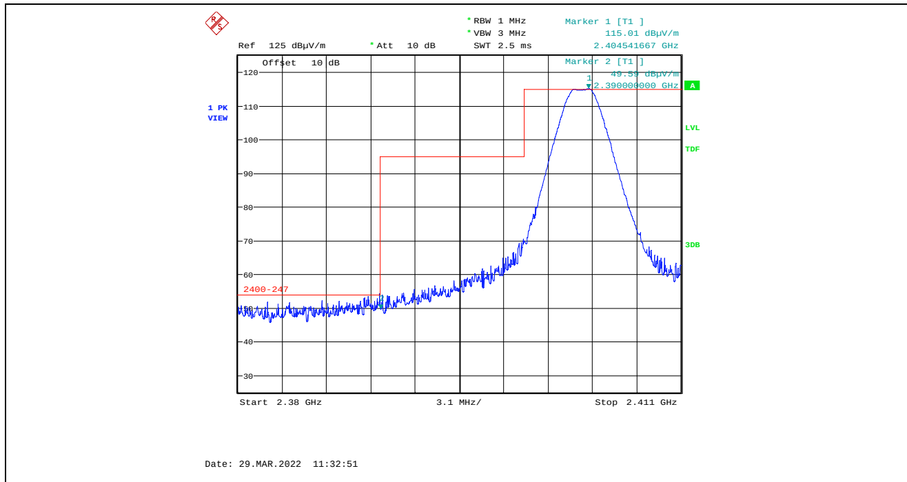
Plot 5.4.4.8.2.3. Band-Edge RF Radiated Emissions at 3 m, Horizontal Polarization, Peak Low End of Frequency Band, 2404 MHz, 8 dBm Power Setting, 2 Mbps
