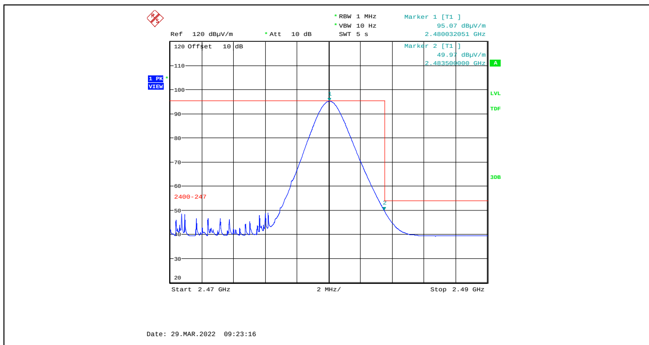
Plot 5.4.4.3.2.8. Band-Edge RF Radiated Emissions at 3 m, Horizontal Polarization, Average High End of Frequency Band, 2480 MHz, 8 dBm Power Setting, 1 Mbps
