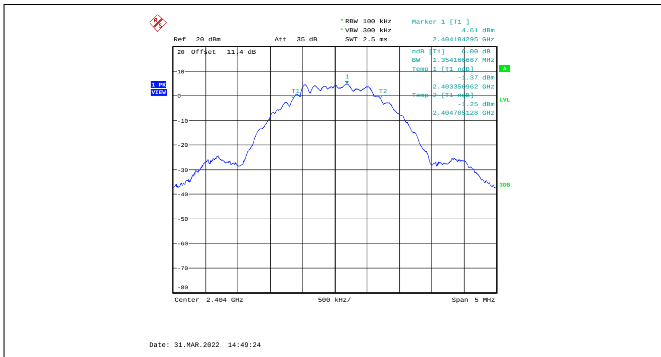
Plot 5.2.4.4. 6 dB Bandwidth, GFSK Modulation, 8 dBm Power Setting, 2 Mbps, 2404 MHz
