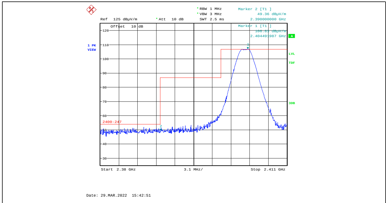
Plot 5.4.4.5.2.3. Band-Edge RF Radiated Emissions at 3 m, Horizontal Polarization, Peak Low End of Frequency Band, 2404 MHz, 8 dBm Power Setting, 2 Mbps
