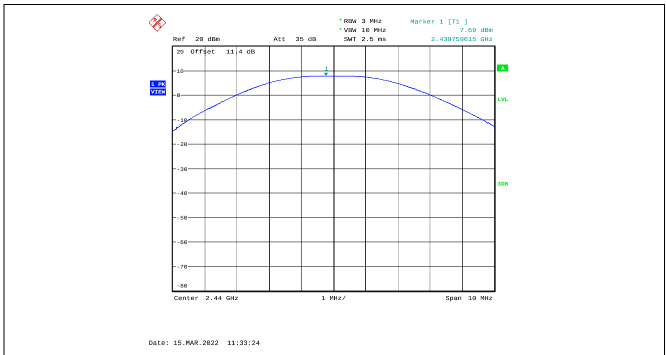
Plot 5.3.4.8. Maximum Peak Conducted Output Power, GFSK Modulation, 2 Mbps, 8 dBm Power Setting, 2440 MHz
