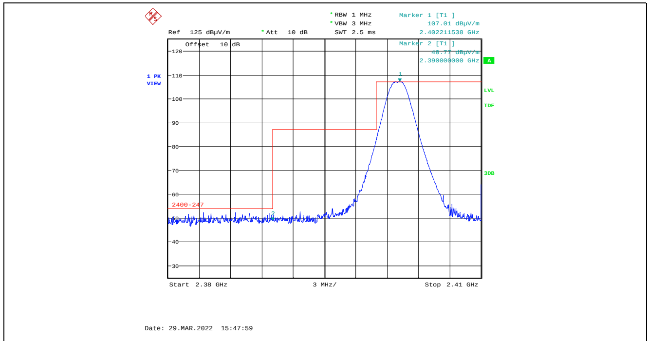
Plot 5.4.4.1.2.3. Band-Edge RF Radiated Emissions at 3 m, Horizontal Polarization, Peak Low End of Frequency Band, 2402 MHz, 8 dBm Power Setting, 1 Mbps
