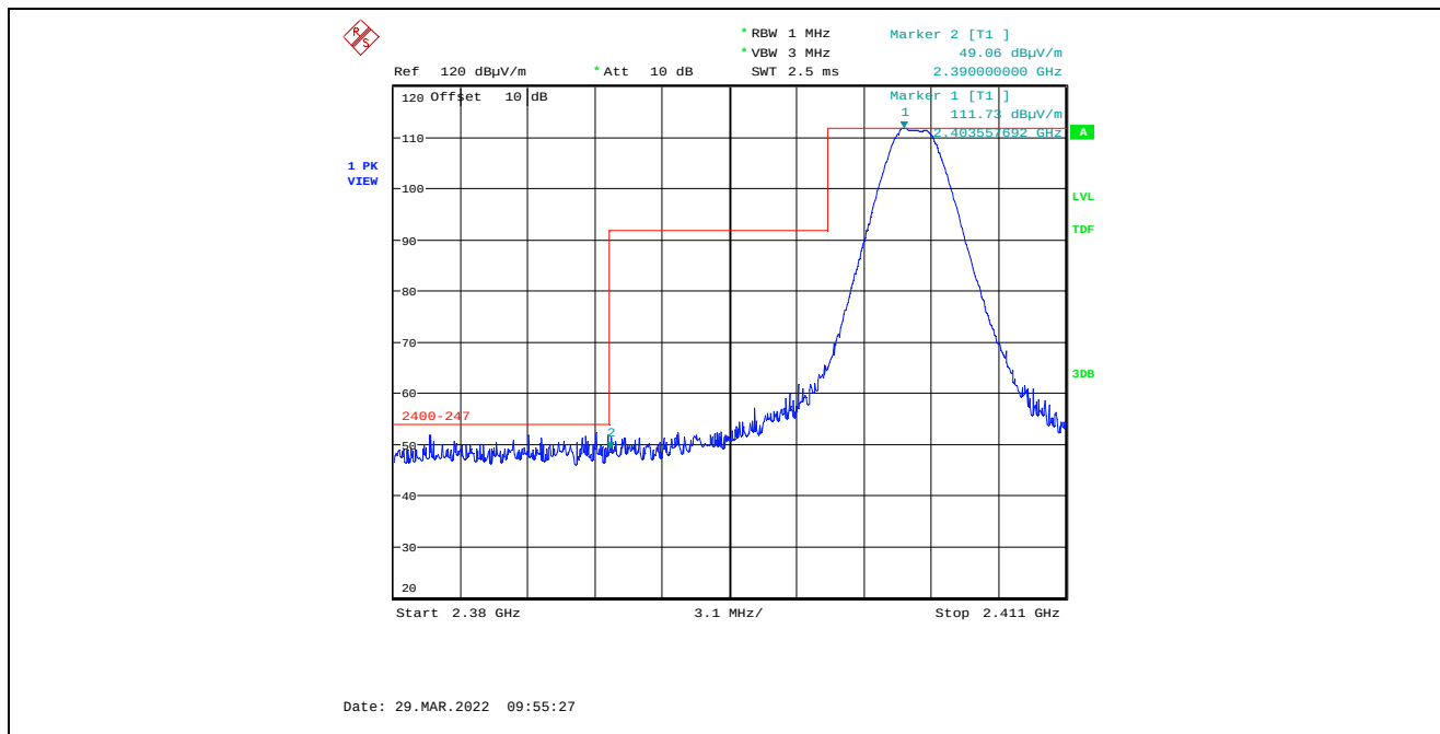
Plot 5.4.4.7.2.1. Band-Edge RF Radiated Emissions at 3 m, Vertical Polarization, Peak Low End of Frequency Band, 2404 MHz, 8 dBm Power Setting, 2 Mbps
