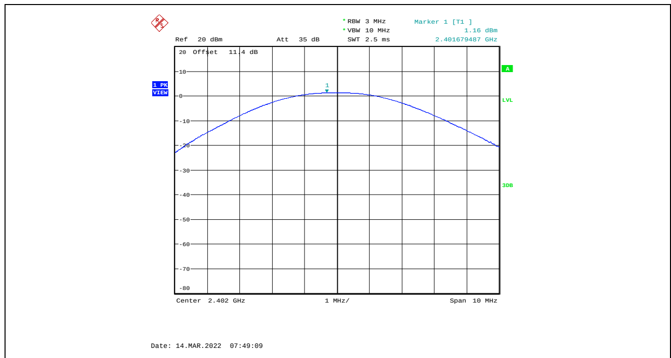
Plot 5.3.4.4. Maximum Peak Conducted Output Power, GFSK Modulation, 1 Mbps, -2 dBm Power Setting, 2402 MHz
