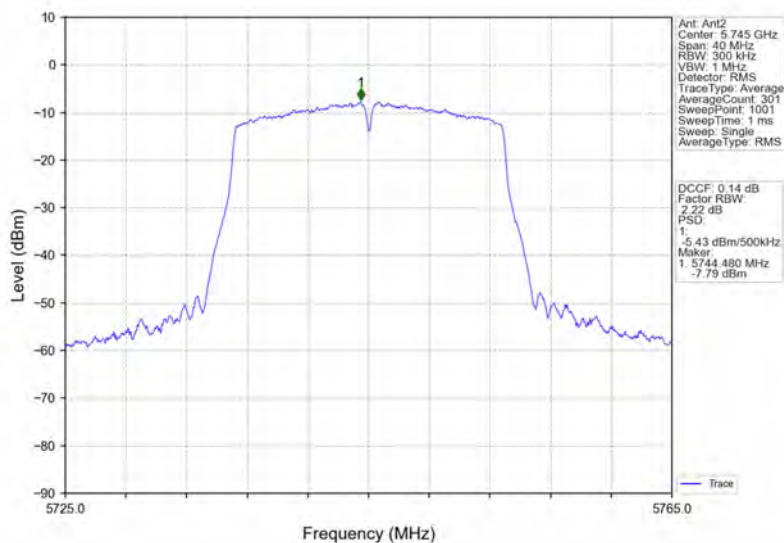
802.11n(HT20)_LCH_5745MHz_Ant2_NTNV
