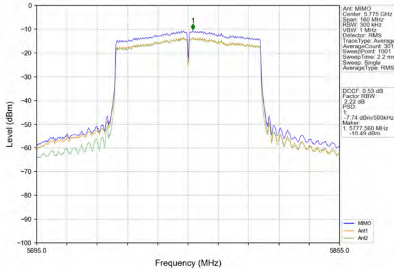
802.11ac(VHT80)_MCH_5775MHz_MIMO_NTNV
