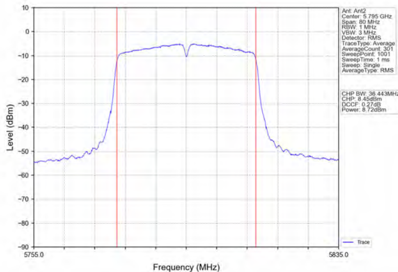
802.11ac(VHT40)_HCH_5795MHz_Ant2_NTNV
