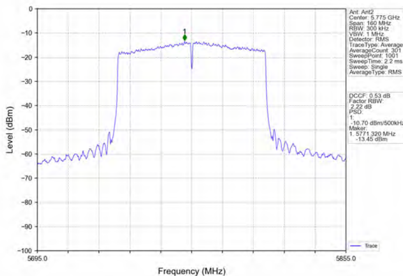
802.11ac(VHT80)_MCH_5775MHz_Ant2_NTNV
