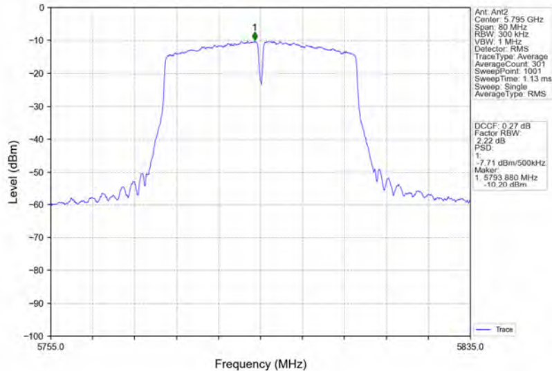
802.11ac(VHT40)_HCH_5795MHz_MIMO_NTNV
