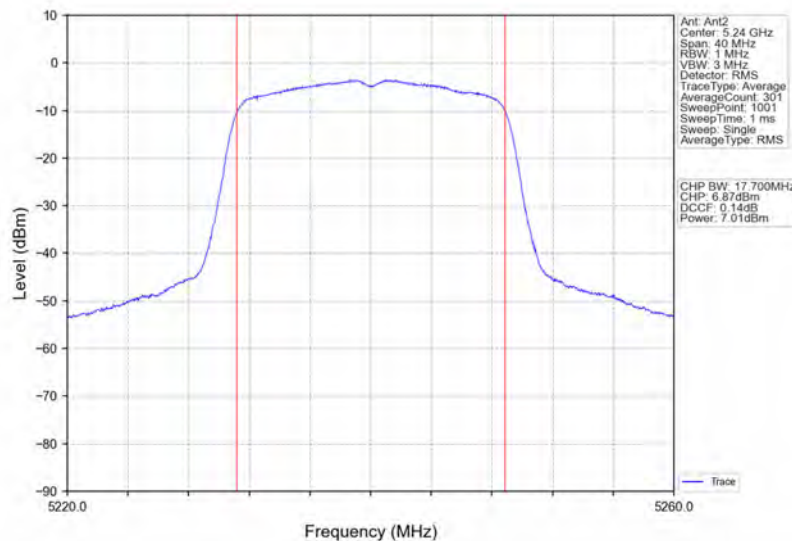
802.11n(HT20)_HCH_5240MHz_Ant2_NTNV
