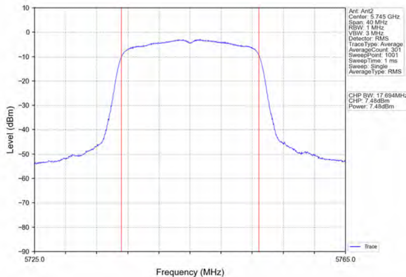
802.11ac(VHT20)_LCH_5745MHz_Ant2_NTNV
