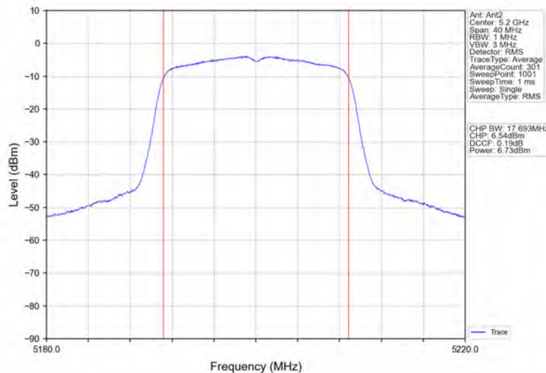
802.11ac(VHT20)_MCH_5200MHz_Ant2_NTNV
