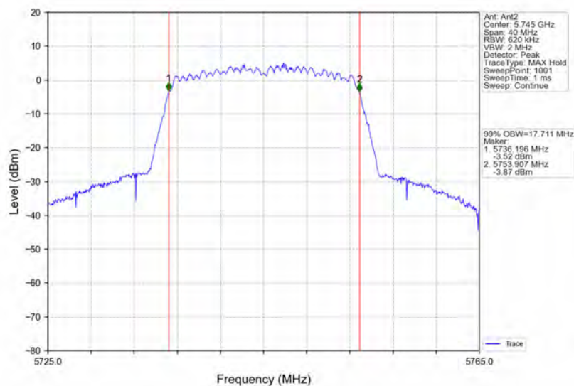
802.11n(HT20)_LCH_5745MHz_Ant2_NTNV
