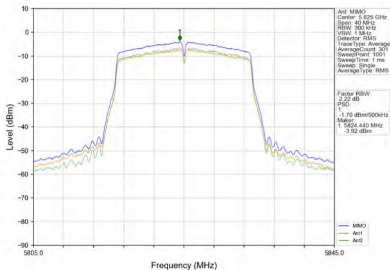
802.11ac(VHT20)_HCH_5825MHz_MIMO_NTNV
