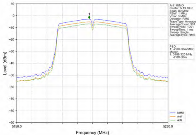
802.11n(HT40)_LCH_5190MHz_MIMO_NTNV
