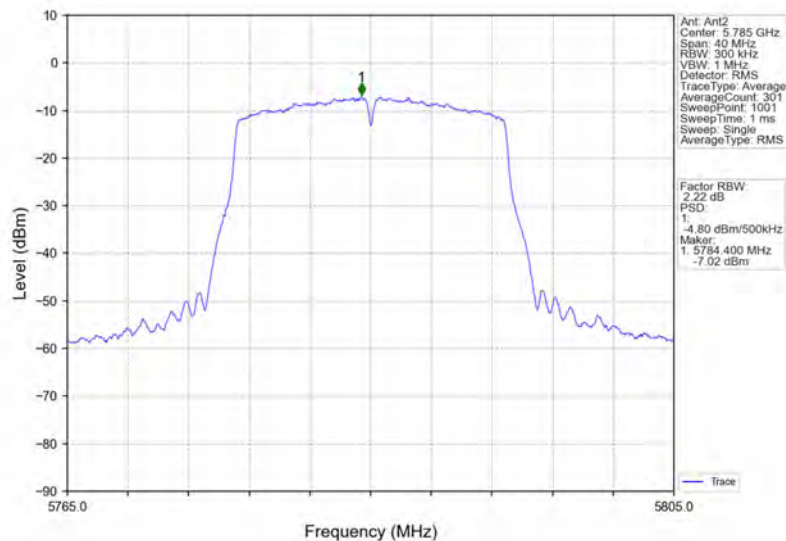
802.11ac(VHT20)_MCH_5785MHz_Ant2_NTNV
