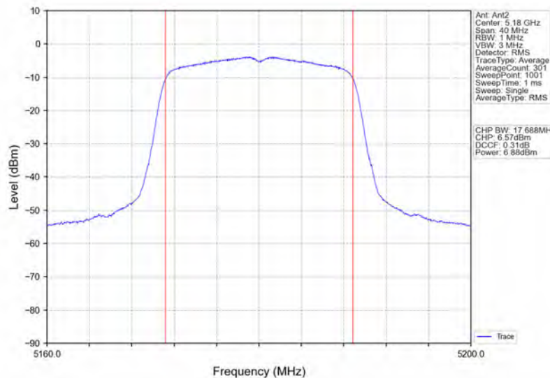
802.11ac(VHT20)_LCH_5180MHz_Ant2_NTNV
