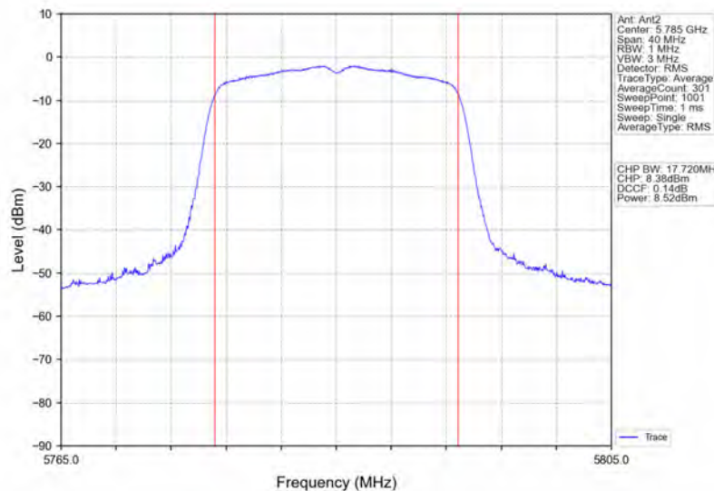
802.11n(HT20)_MCH_5785MHz_Ant2_NTNV
