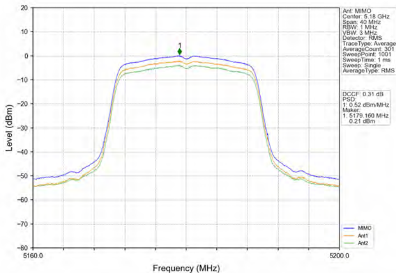
802.11ac(VHT20)_LCH_5180MHz_MIMO_NTNV
