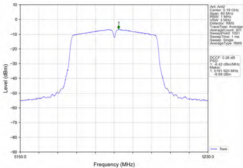
802.11ac(VHT40)_LCH_5190MHz_Ant2_NTNV
