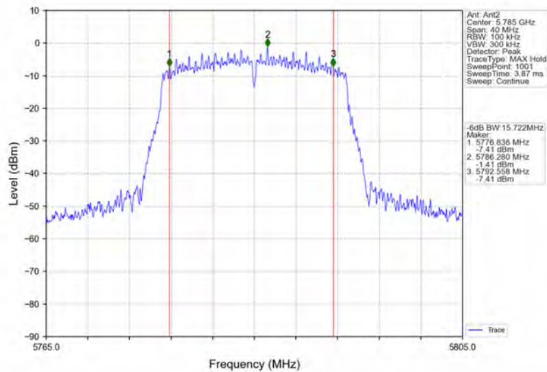
802.11ac(VHT20)_MCH_5785MHz_Ant2_NTNV
