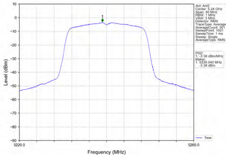
802.11ac(VHT20)_HCH_5240MHz_MIMO_NTNV
