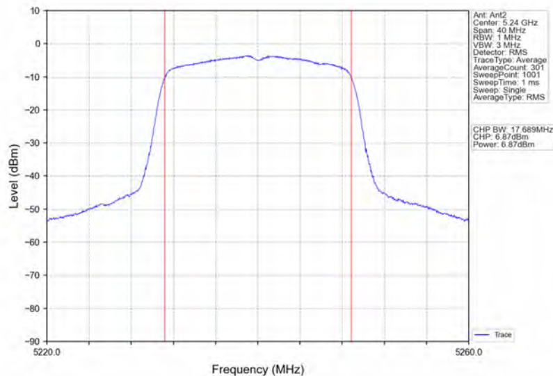
802.11ac(VHT20)_HCH_5240MHz_Ant2_NTNV
