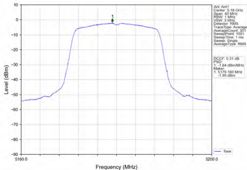
802.11ac(VHT20)_LCH_5180MHz_Ant1_NTNV
