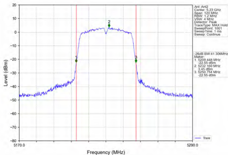
802.11ac(VHT40)_HCH_5230MHz_Ant2_NTNV
