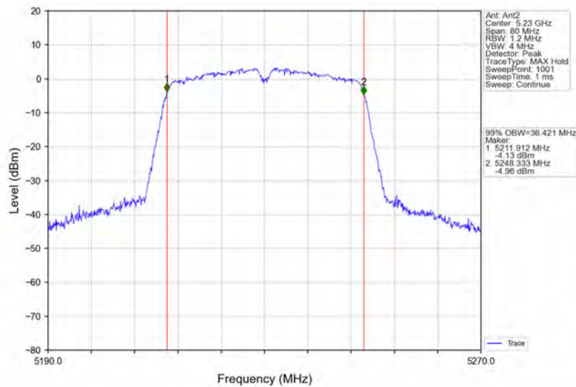
802.11ac(VHT40)_HCH_5230MHz_Ant2_NTNV
