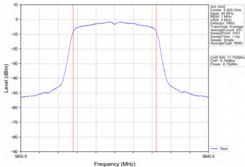
802.11ac(VHT20)_HCH_5825MHz_Ant2_NTNV
