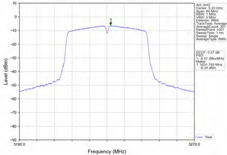
802.11ac(VHT40)_HCH_5230MHz_MIMO_NTNV
