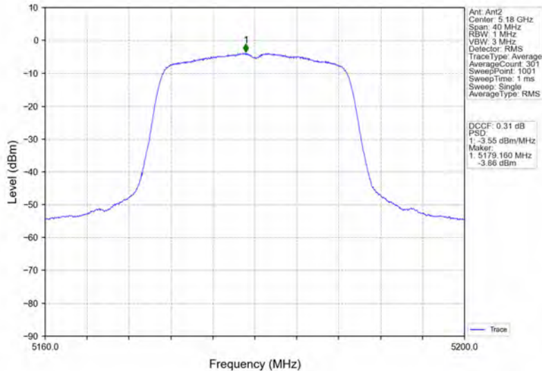
802.11ac(VHT20)_LCH_5180MHz_MIMO_NTNV
