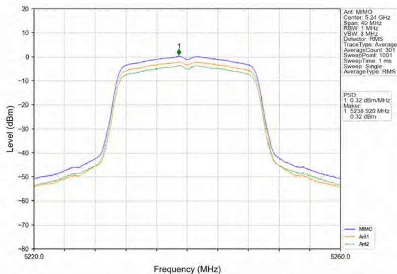
802.11ac(VHT20)_HCH_5240MHz_MIMO_NTNV
