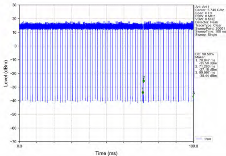
802.11a_LCH_5745MHz_Ant1_NTNV
