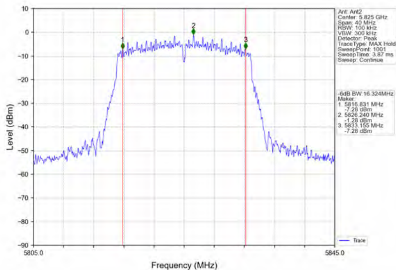
802.11ac(VHT20)_HCH_5825MHz_Ant2_NTNV
