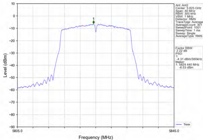
802.11ac(VHT20)_HCH_5825MHz_MIMO_NTNV
