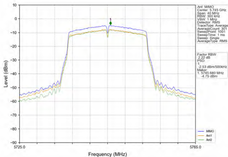
802.11ac(VHT20)_LCH_5745MHz_MIMO_NTNV
