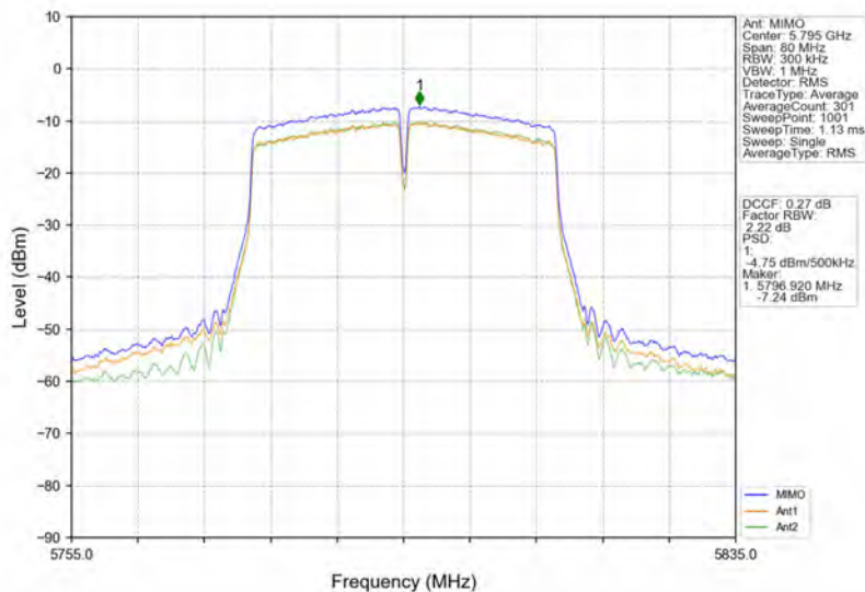
802.11ac(VHT40)_HCH_5795MHz_MIMO_NTNV
