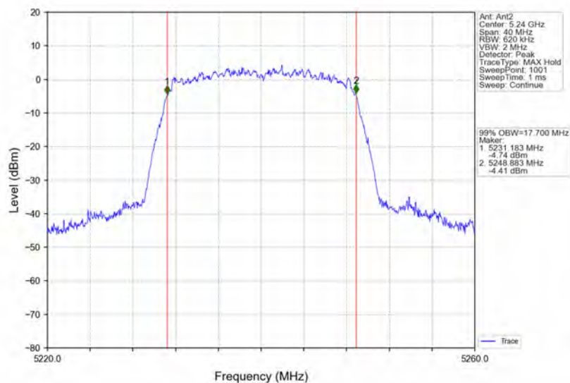
802.11n(HT20)_HCH_5240MHz_Ant2_NTNV
