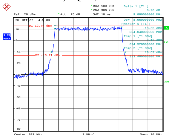
10M, 16QAM, Low Channel
