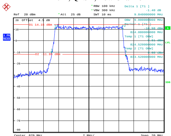
10M, QPSK, Low Channel
