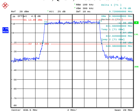
10M, QPSK, Middle Channel
