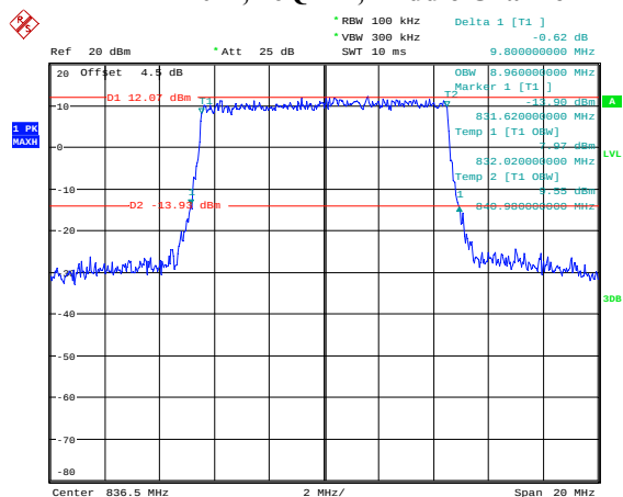
10M, 16QAM, Middle Channel
