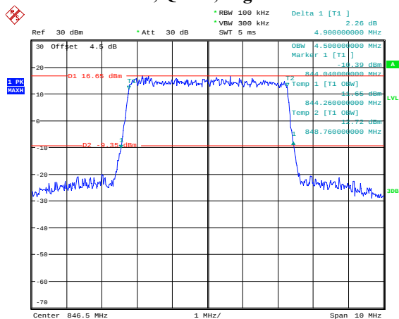
5M, QPSK, High Channel
