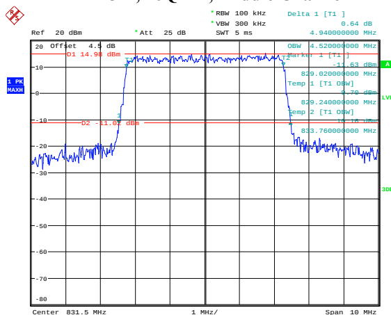
5M, 16QAM, Middle Channel
