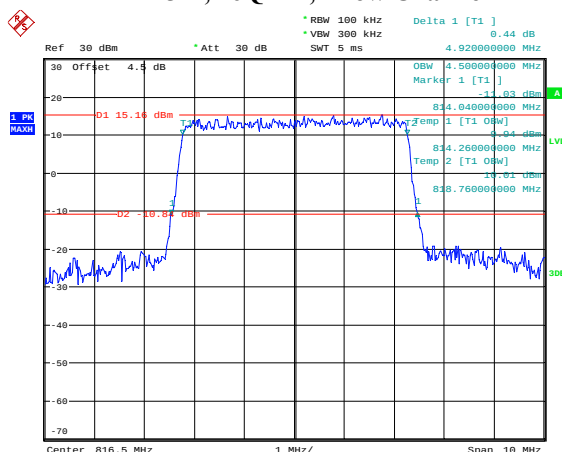
5M, 16QAM, Low Channel
