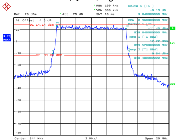
10M, QPSK, High Channel
