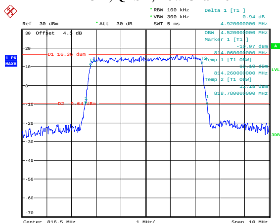
5M, QPSK, Low Channel
