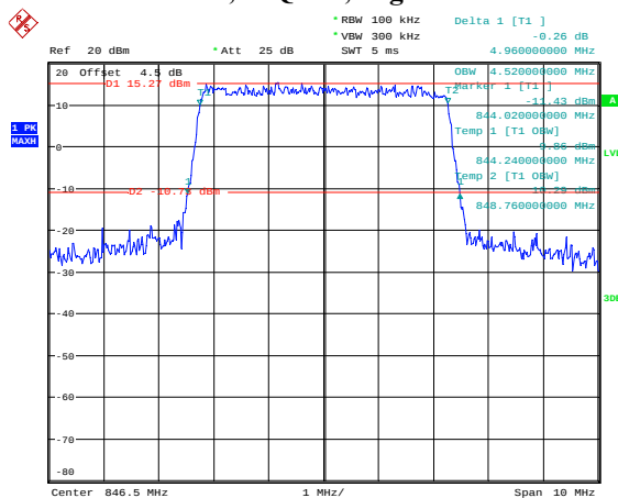
5M, 16QAM, High Channel
