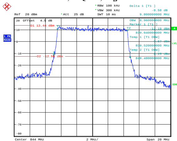
10M, 16QAM, High Channel
