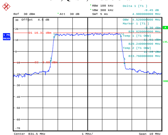
5M, QPSK, Middle Channel
