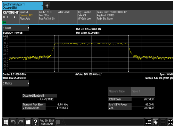
N30(5M)_CP- OFDM_QPSK_Outer_Full_Mid_CH
