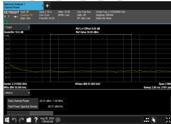
N30(10M)_DFT-s- OFDM_QPSK_Outer_Full_Low_CH_CHP_PASS
