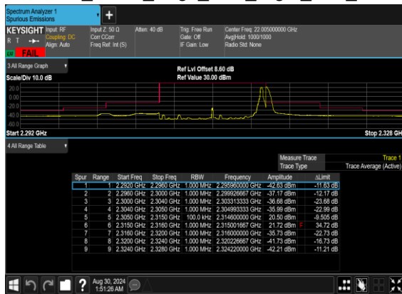
N30(10M)_DFT-s-OFDM_BPSK_Edge_1RB_Right_Low_CH
