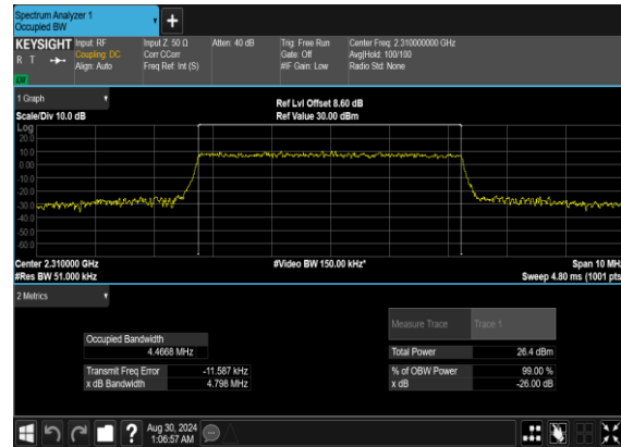
N30(5M)_CP-OFDM_16 QAM_Outer_Full_Mid_CH
