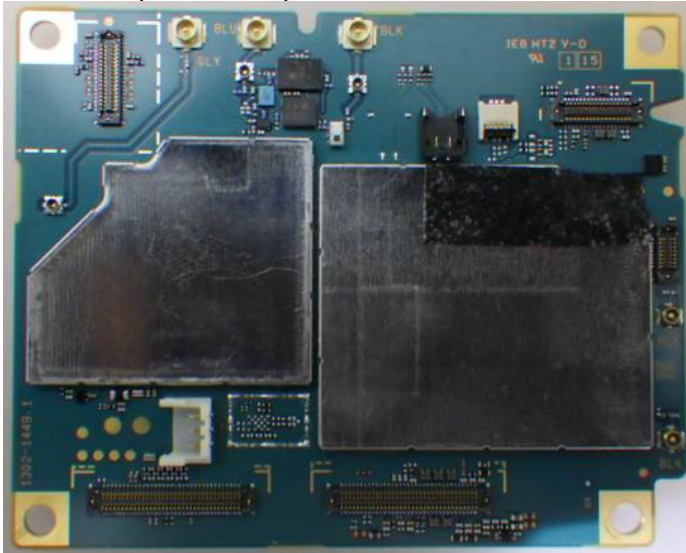
Main PBA(Outer Side)
