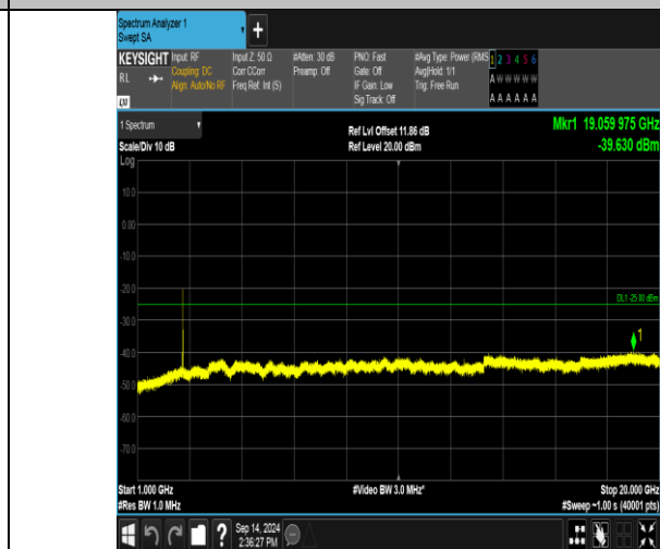
Band41_10MHz_QPSK_41190_1RB#49_1000~20000_1000~20000
