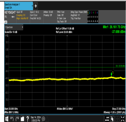
Band41_15MHz_16QAM_40115_1RB#74_20000-27000_20000-27000
