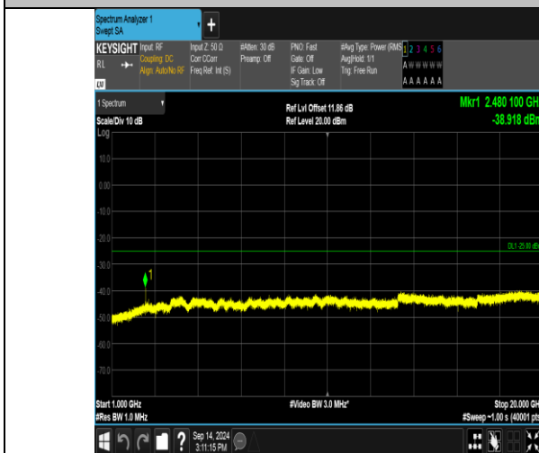
Band41_15MHz_16QAM_40590_1RB#74_1000~20000_1000~20000
