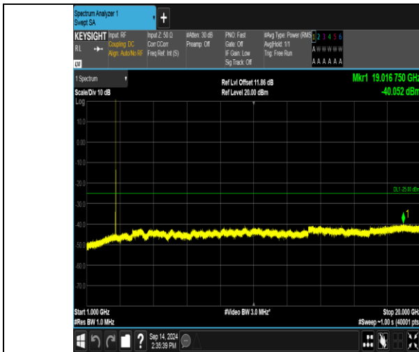
Band41_10MHz_16QAM_41190_1RB#0_1000~20000_1000~20000
