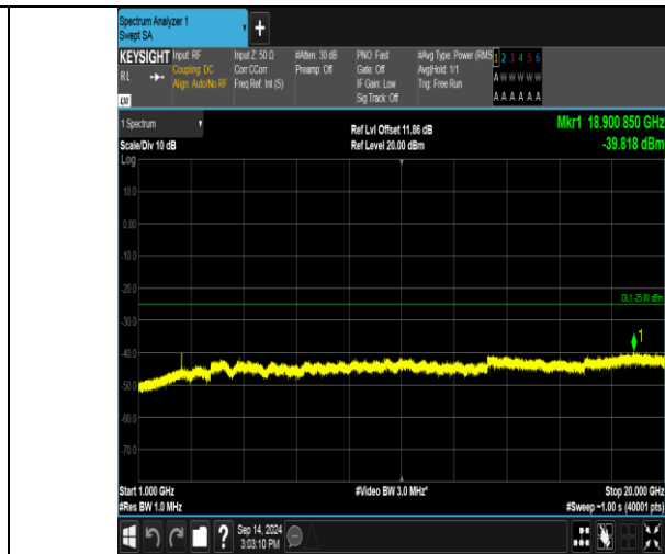
Band41_15MHz_QPSK_40115_1RB#0_1000~20000_1000~20000
