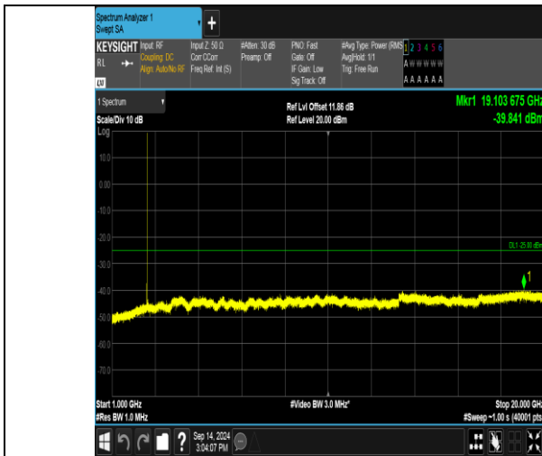
Band41_15MHz_16QAM_40115_1RB#0_1000~20000_1000~20000
