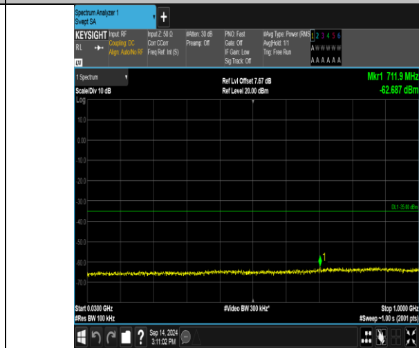
Band41_15MHz_16QAM_40590_1RB#74_30~1000_30~1000
