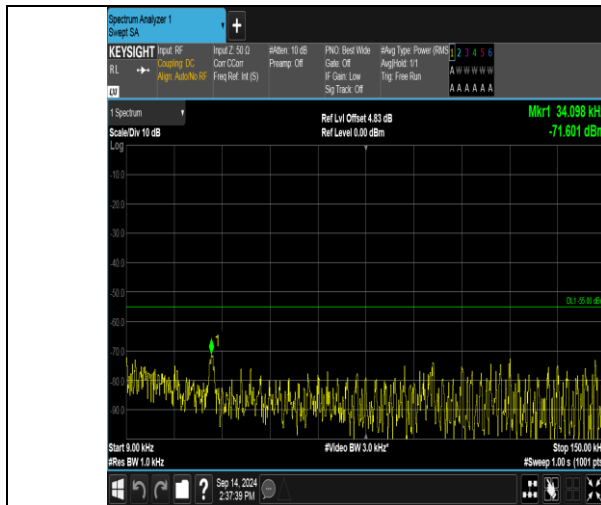
Band41_10MHz_QPSK_41190_50RB#0_0.009~0.15_0.009~0.15
