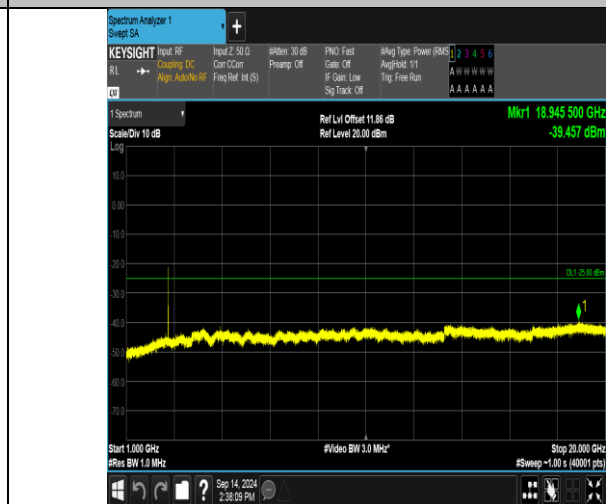
Band41_10MHz_QPSK_41190_50RB#0_1000~20000_1000~20000
