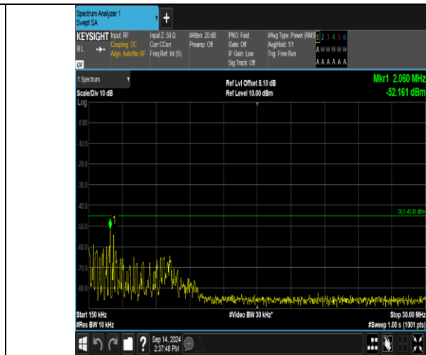
Band41_10MHz_QPSK_41190_50RB#0_0.15~30_0.15~30
