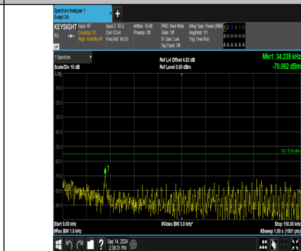
Band41_10MHz_16QAM_41190_50RB#0_0.009~0.15_0.009~0.15
