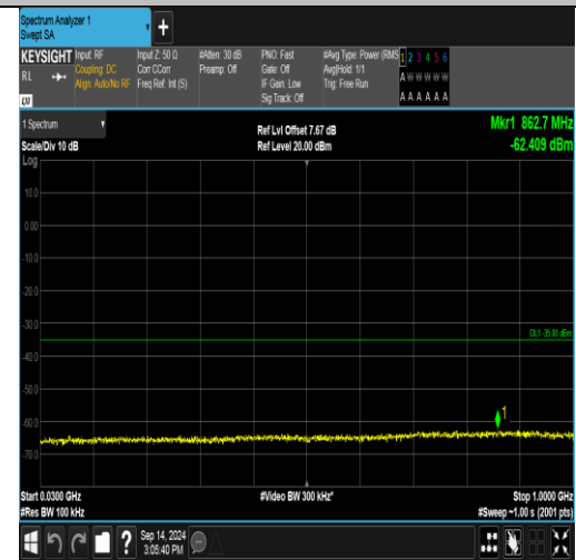
Band41_15MHz_16QAM_40115_1RB#74_30-1000_30-1000
