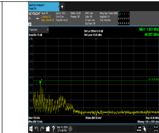
Band41_15MHz_QPSK_40590_75RB#0_0.15~30_0.15~30
