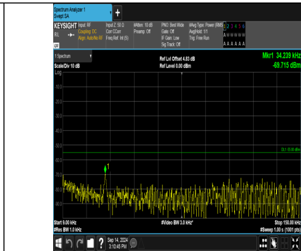
Band41_15MHz_16QAM_40590_1RB#74_0.009~0.15_0.009~0.15
