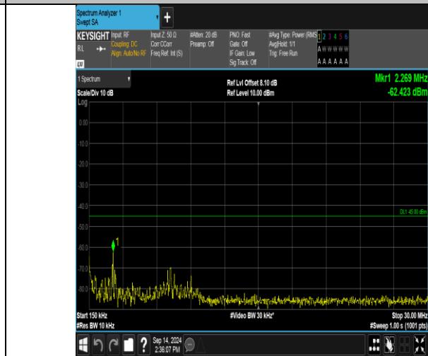
Band41_10MHz_QPSK_41190_1RB#49_0.15~30_0.15~30
