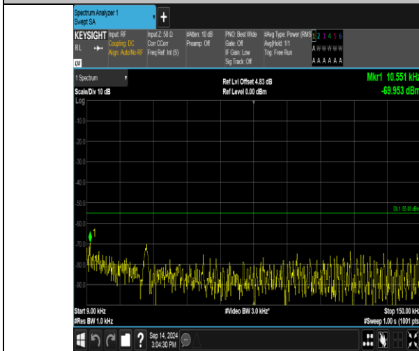
Band41_15MHz_QPSK_40115_1RB#74_0.009~0.15_0.009~0.15
