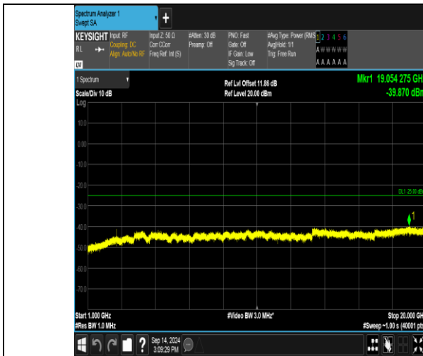
Band41_15MHz_16QAM_40590_1RB#0_1000~20000_1000~20000
