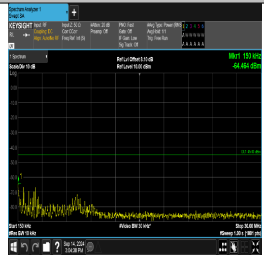
Band41_15MHz_QPSK_40115_1RB#74_0.15~30_0.15~30
