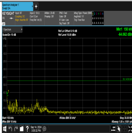
Band41_15MHz_16QAM_40115_1RB#74_0.15-30_0.15-30
