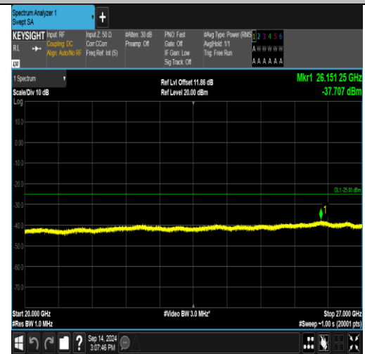
Band41_15MHz_16QAM_40115_75RB#0_20000~27000_20000~27000
