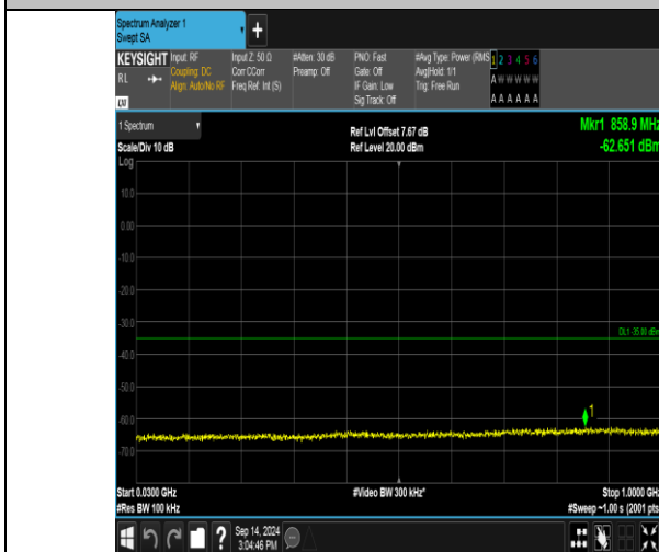
Band41_15MHz_QPSK_40115_1RB#74_30~1000_30~1000
