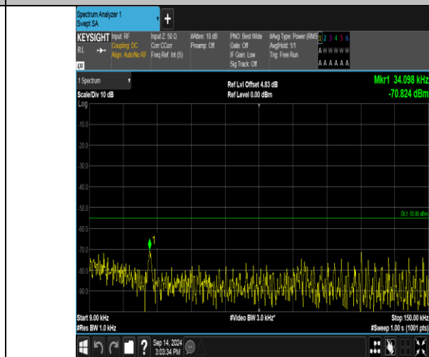
Band41_15MHz_16QAM_40115_1RB#0_0.009~0.15_0.009~0.15
