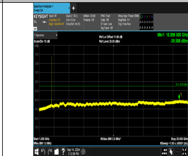
Band41_15MHz_QPSK_40590_75RB#0_1000~20000_1000~20000
