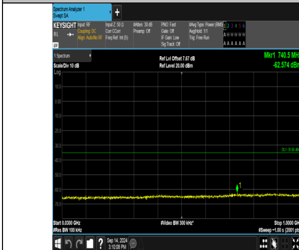
Band41_15MHz_QPSK_40590_1RB#74_30~1000_30~1000
