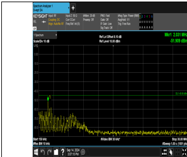
Band41_15MHz_16QAM_40115_75RB#0_0.15~30_0.15~30
