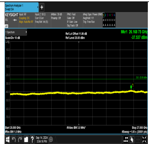
Band41_15MHz_16QAM_40115_1RB#0_20000~27000_20000~27000
