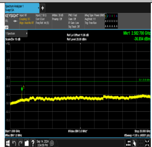
Band41_15MHz_QPSK_40115_1RB#74_1000~20000_1000~20000
