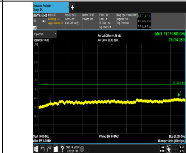
Band41_15MHz_QPSK_40590_1RB#74_1000~20000_1000~20000
