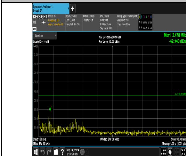
Band41_10MHz_16QAM_41190_1RB#0_0.15~30_0.15~30
