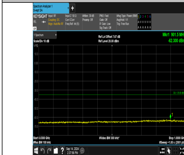
Band41_10MHz_QPSK_41190_50RB#0_30~1000_30~1000
