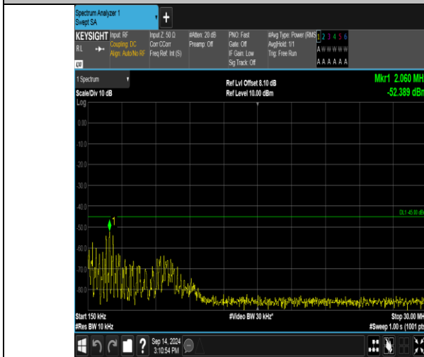
Band41_15MHz_16QAM_40590_1RB#74_0.15~30_0.15~30
