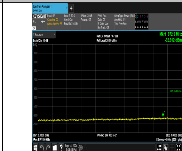
Band41_15MHz_16QAM_40115_1RB#0_30~1000_30~1000
