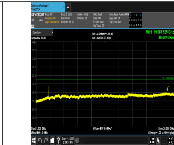
Band41_10MHz_QPSK_41190_1RB#0_1000~20000_1000~20000
