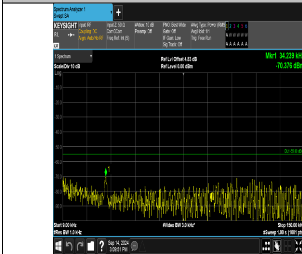
Band41_15MHz_QPSK_40590_1RB#74_0.009~0.15_0.009~0.15
