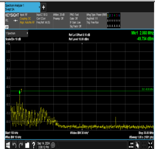
Band41_15MHz_QPSK_40590_1RB#0_0.15~30_0.15~30
