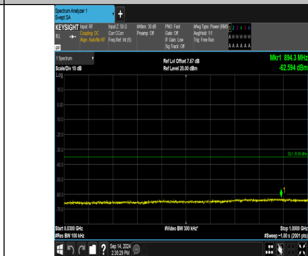
Band41_10MHz_16QAM_41190_1RB#0_30~1000_30~1000
