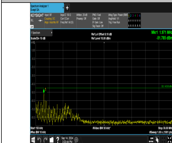
Band41_15MHz_16QAM_40115_1RB#0_0.15~30_0.15~30
