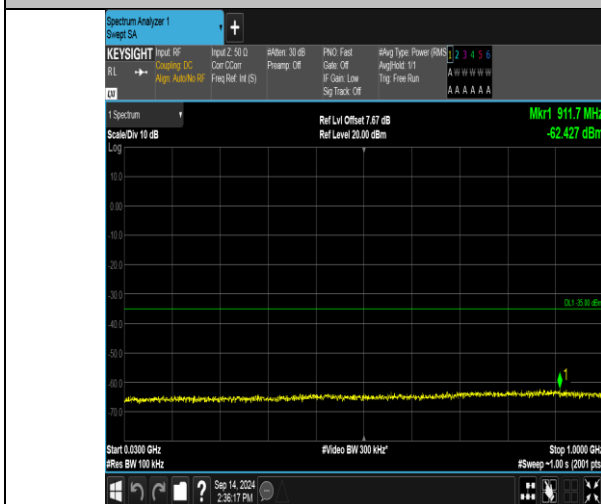
Band41_10MHz_QPSK_41190_1RB#49_30~1000_30~1000
