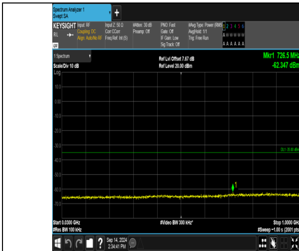
Band41_10MHz_QPSK_41190_1RB#0_30~1000_30~1000
