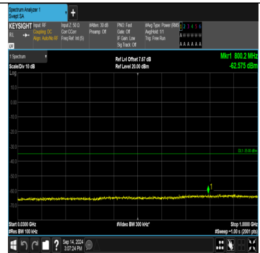
Band41_15MHz_16QAM_40115_75RB#0_30~1000_30~1000
