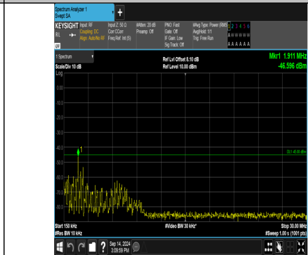
Band41_15MHz_QPSK_40590_1RB#74_0.15~30_0.15~30
