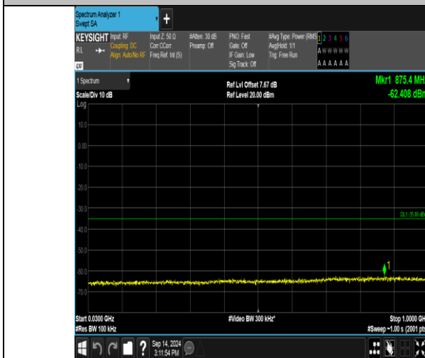
Band41_15MHz_QPSK_40590_75RB#0_30~1000_30~1000
