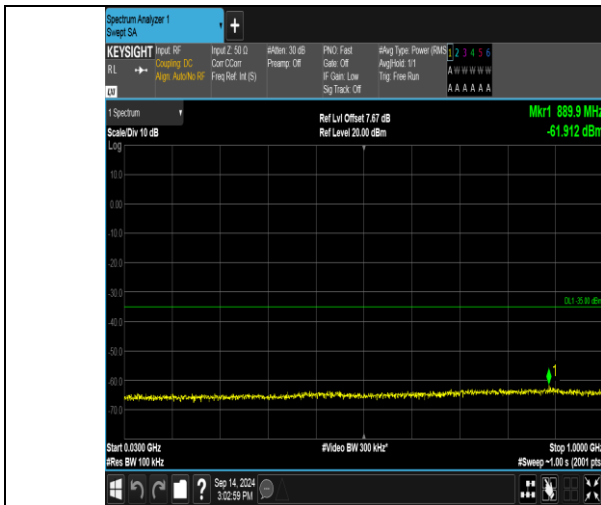
Band41_15MHz_QPSK_40115_1RB#0_30~1000_30~1000
