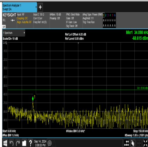
Band41_15MHz_QPSK_40590_1RB#0_0.009~0.15_0.009~0.15
