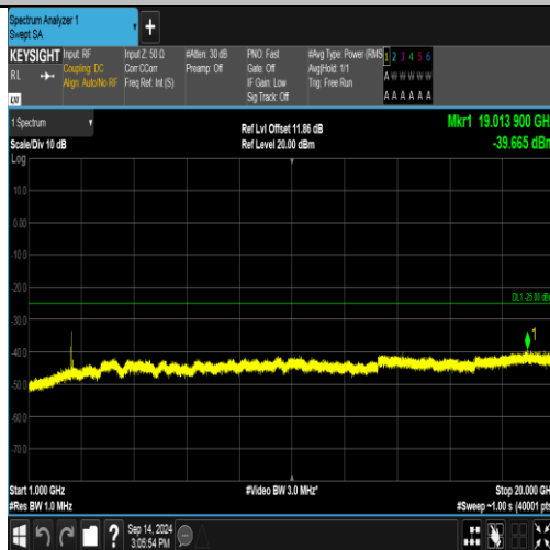
Band41_15MHz_16QAM_40115_1RB#74_1000-20000_1000-20000
