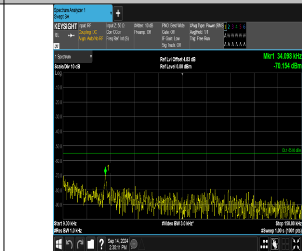
Band41_10MHz_16QAM_41190_1RB#0_0.009~0.15_0.009~0.15
