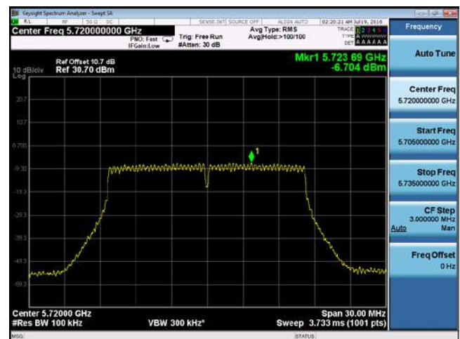
PSD-802.11a-CROSS-5720M-chain2
