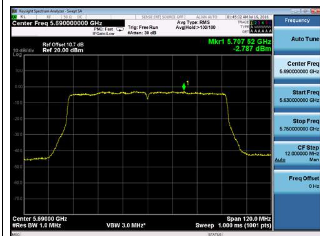
PSD-802.11ac-CROSS-5690M-chain1
