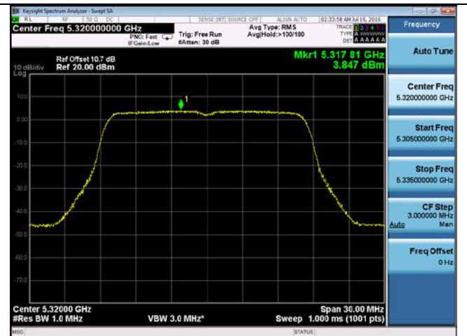
PSD-802.11a-5320M-chain2
