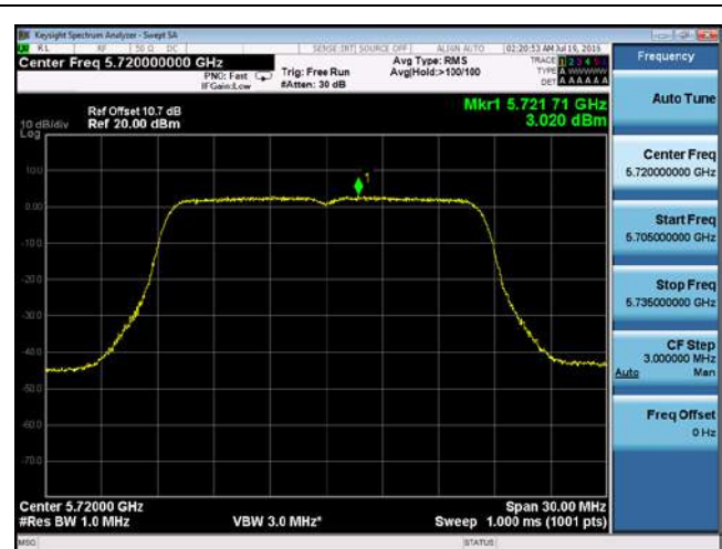
PSD-802.11a-CROSS-5720M-chain2
