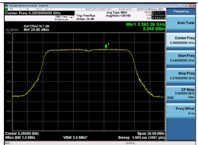
PSD-802.11a-5260M-chain4
