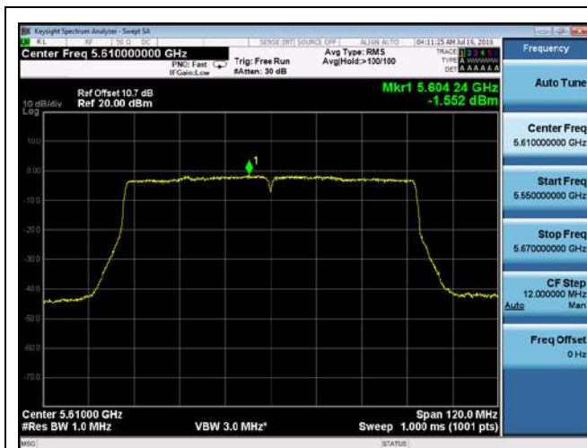
PSD-802.11ac-80M-5610M-chain3
