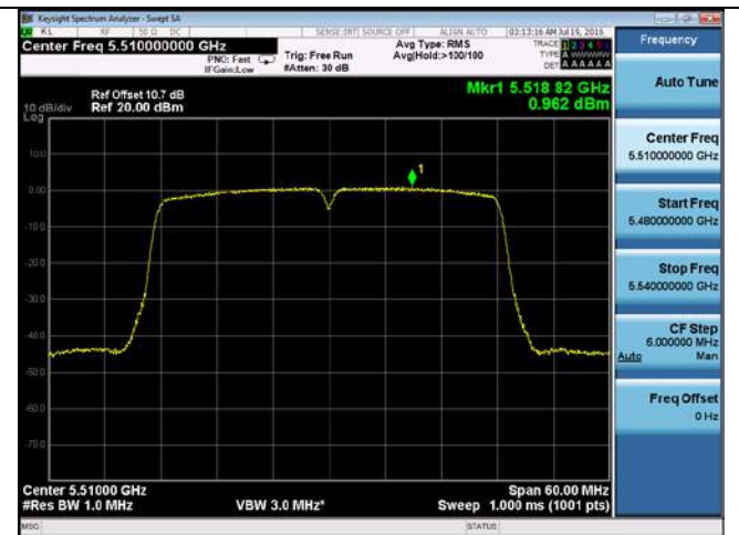
PSD-802.11n-40M-5510M-chain2
