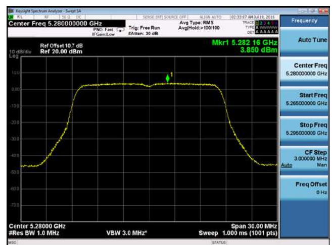
PSD-802.11a-5280M-chain2
