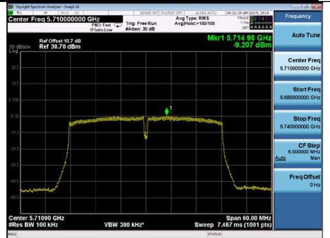
PSD-802.11n-40M-CROSS-5710M-chain4
