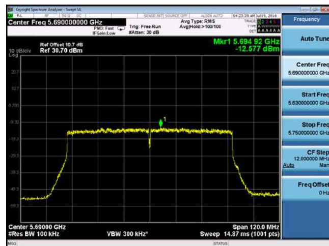
PSD-802.11ac-CROSS-5690M-chain3
