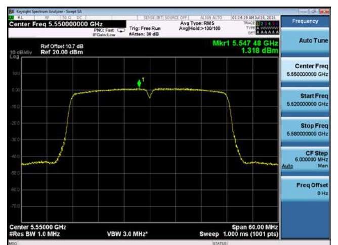
PSD-802.11n-40M-5550M-chain2
