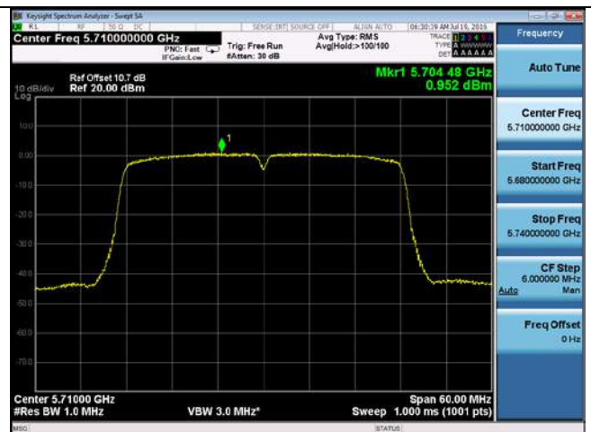
PSD-802.11n-40M-CROSS-5710M-chain4
