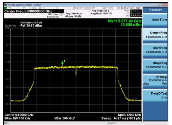
PSD-802.11ac-CROSS-5690M-chain2
