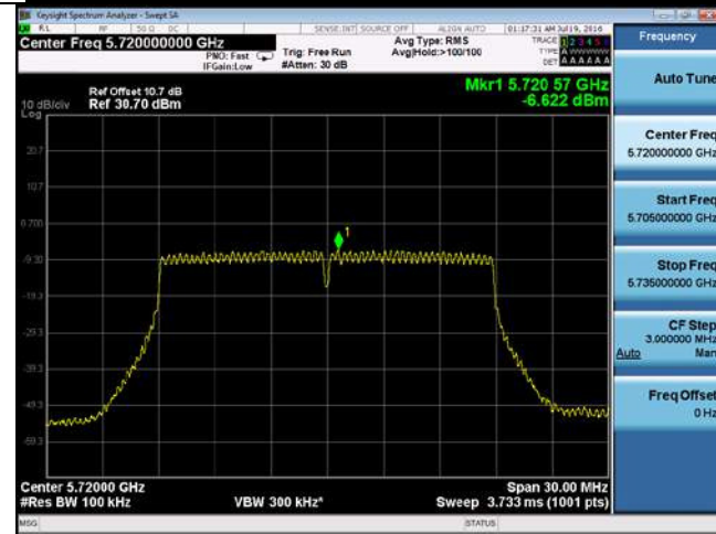
PSD-802.11n-20M-CROSS-5720M-chain1
