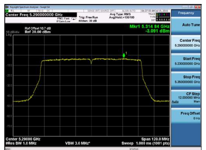
PSD-802.11ac-80M-5290M-chain4
