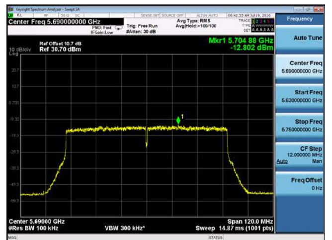
PSD-802.11ac-CROSS-5690M-chain4
