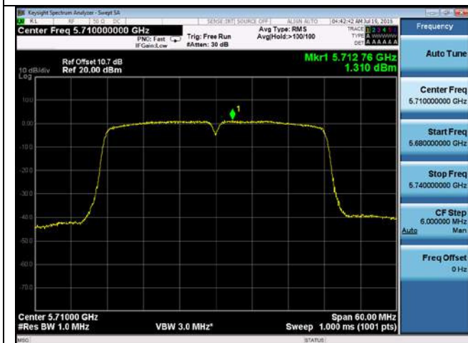
PSD-802.11n-40M-CROSS-5710M-chain3
