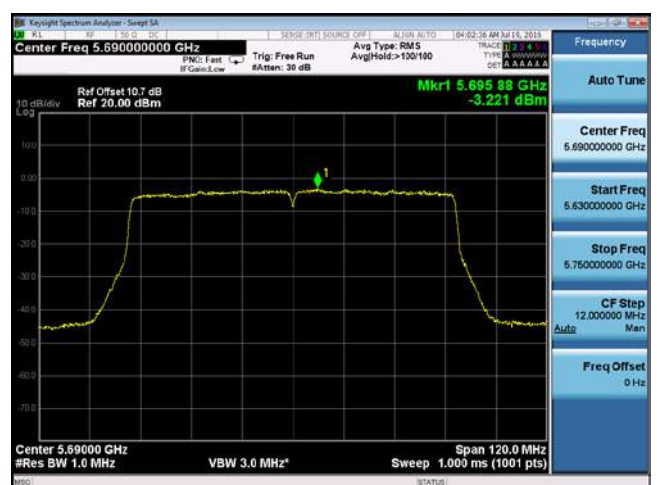
PSD-802.11ac-CROSS-5690M-chain2
