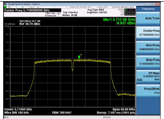
PSD-802.11n-40M-CROSS-5710M-chain2
