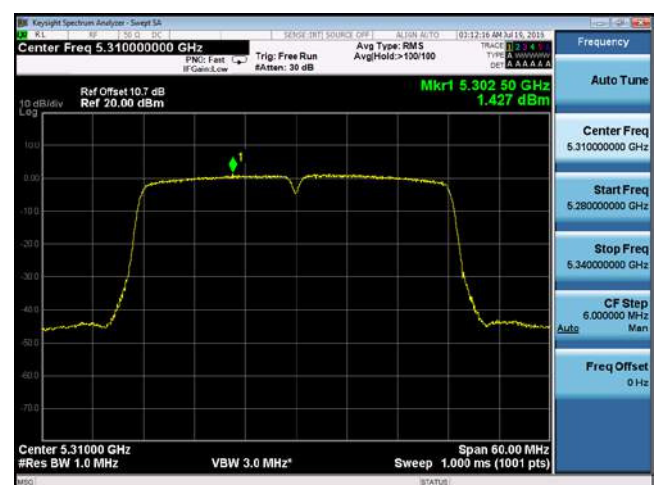
PSD-802.11n-40M-5310M-chain2
