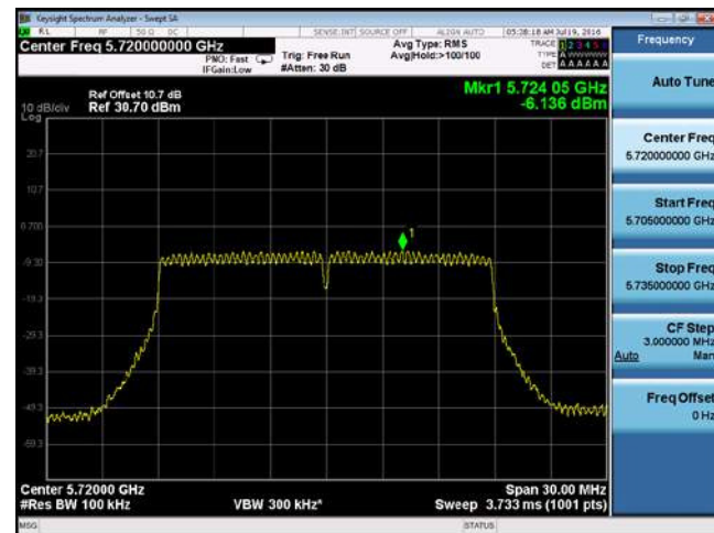
PSD-802.11n-20M-CROSS-5720M-chain3
