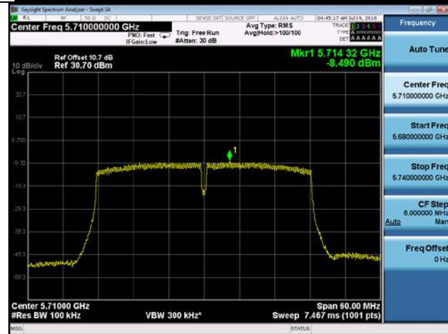
PSD-802.11n-40M-CROSS-5710M-chain3
