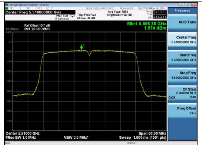
PSD-802.11n-40M-5510M-chain4
