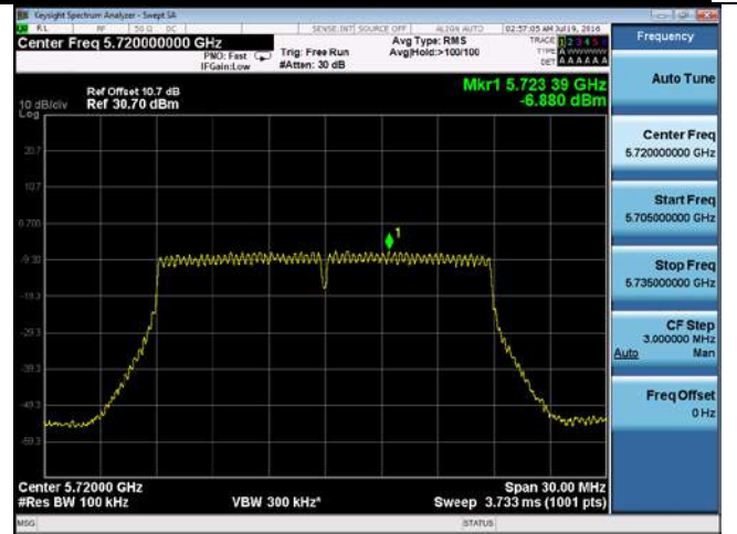
PSD-802.11n-20M-CROSS-5720M-chain2
