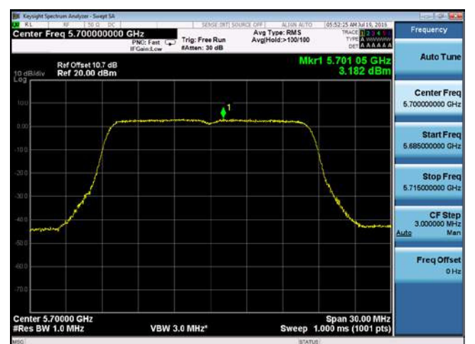
PSD-802.11a-5700M-chain4
