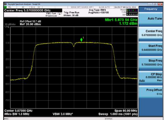
PSD-802.11n-40M-5670M-chain4
