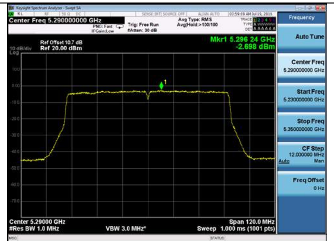
PSD-802.11ac-80M-5290M-chain2
