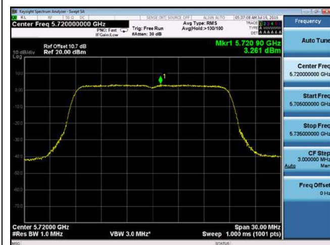
PSD-802.11n-20M-CROSS-5720M-chain3
