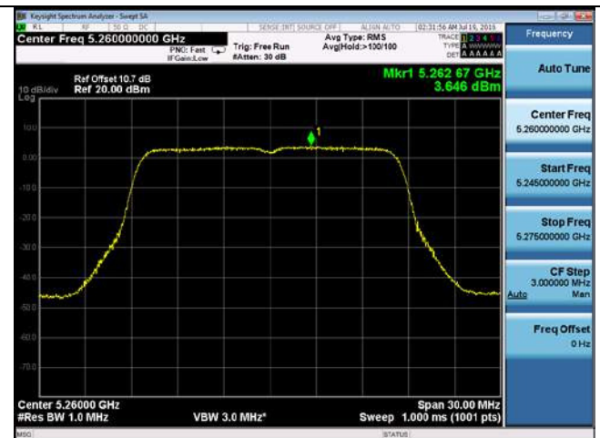
PSD-802.11a-5260M-chain2
