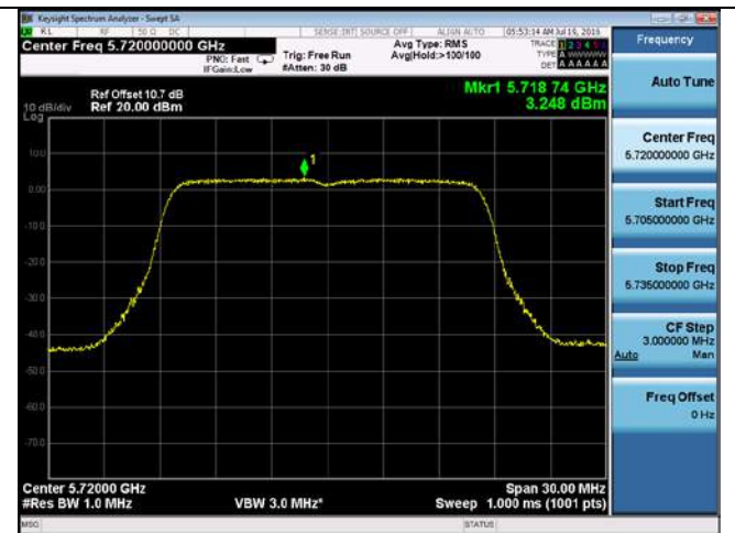
PSD-802.11a-CROSS-5720M-chain4
