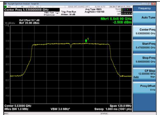
PSD-802.11ac-80M-5530M-chain4
