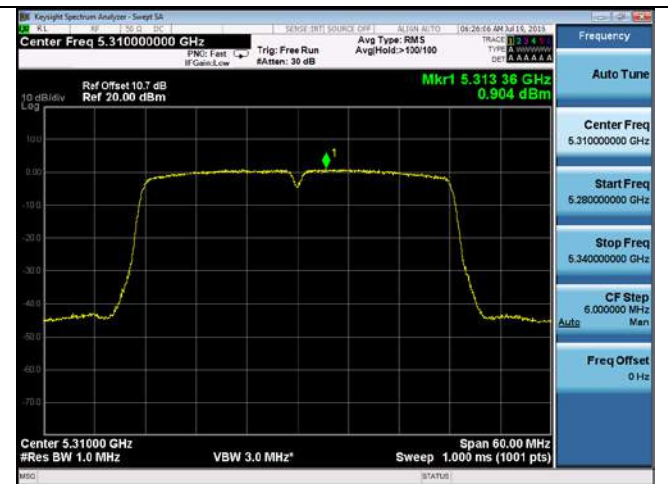
PSD-802.11n-40M-5310M-chain4
