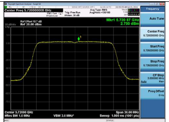
PSD-802.11n-20M-CROSS-5720M-chain2
