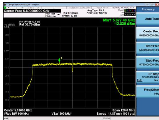
PSD-802.11ac-CROSS-5690M-chain1
