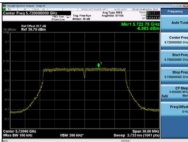
PSD-802.11a-CROSS-5720M-chain3
