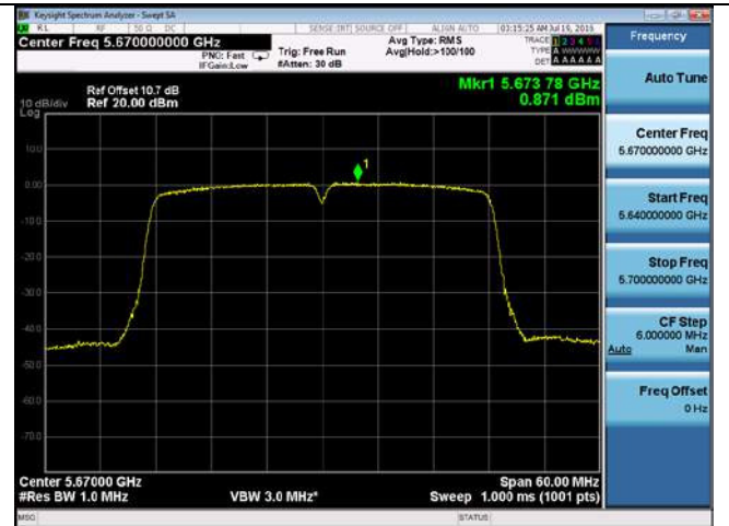
PSD-802.11n-40M-5670M-chain2
