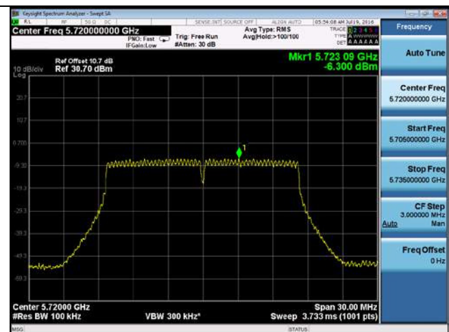
PSD-802.11a-CROSS-5720M-chain4
