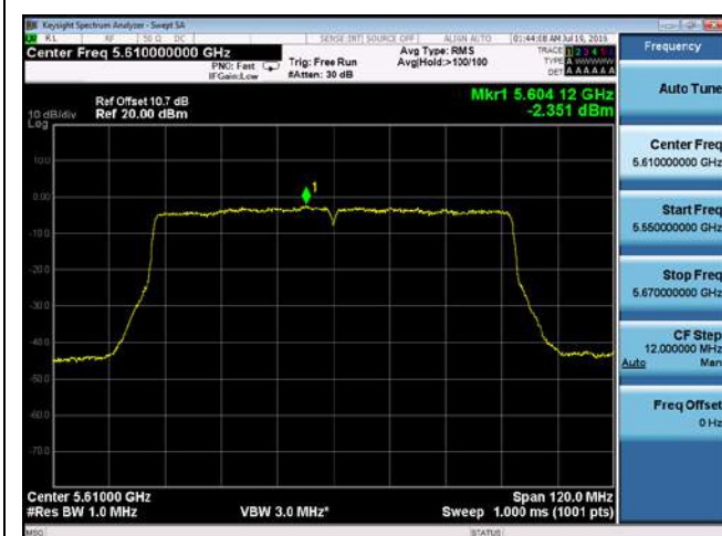
PSD-802.11ac-80M-5610M-chain1
