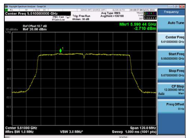
PSD-802.11ac-80M-5610M-chain2
