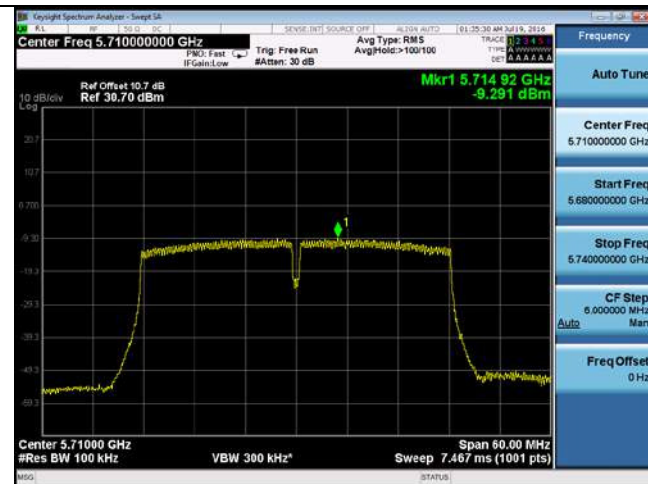
PSD-802.11n-40M-CROSS-5710M-chain1
