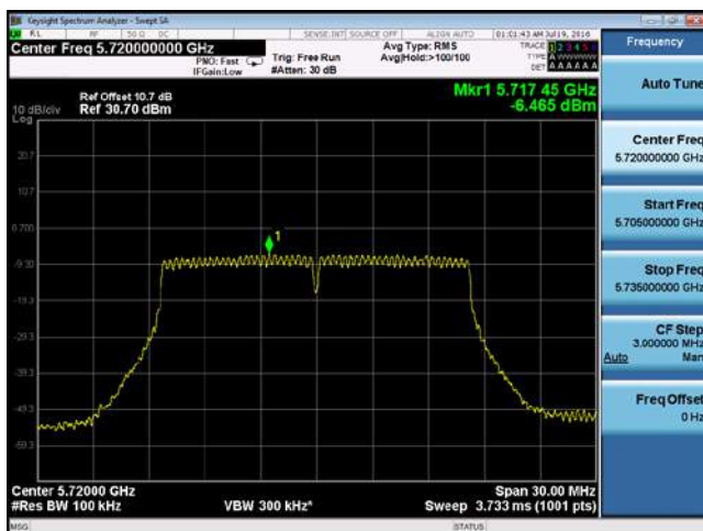
PSD-802.11a-CROSS-5720M-chain1
