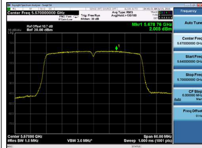
PSD-802.11n-40M-5670M-chain3
