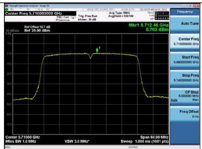
PSD-802.11n-40M-CROSS-5710M-chain2
