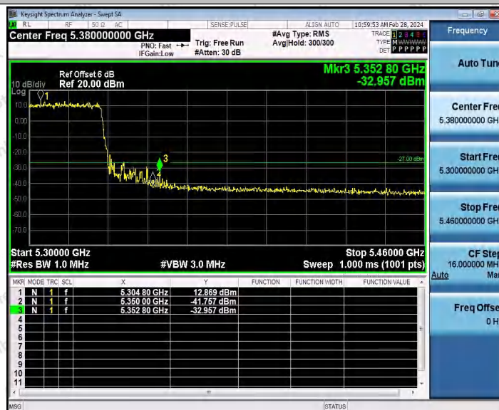
11AX40SISO_Ant1_High_5310
