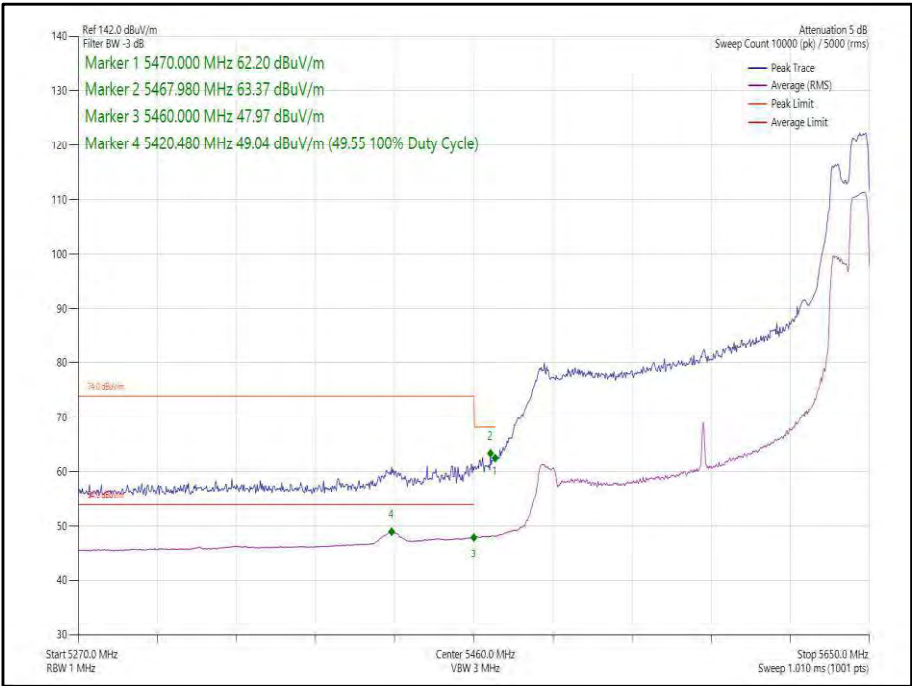
Figure 154 - 802.11ax, HE160, RU 106-60, SISO, Core 1 - 5570 MHz, Band Edge Frequency 5460 MHz
