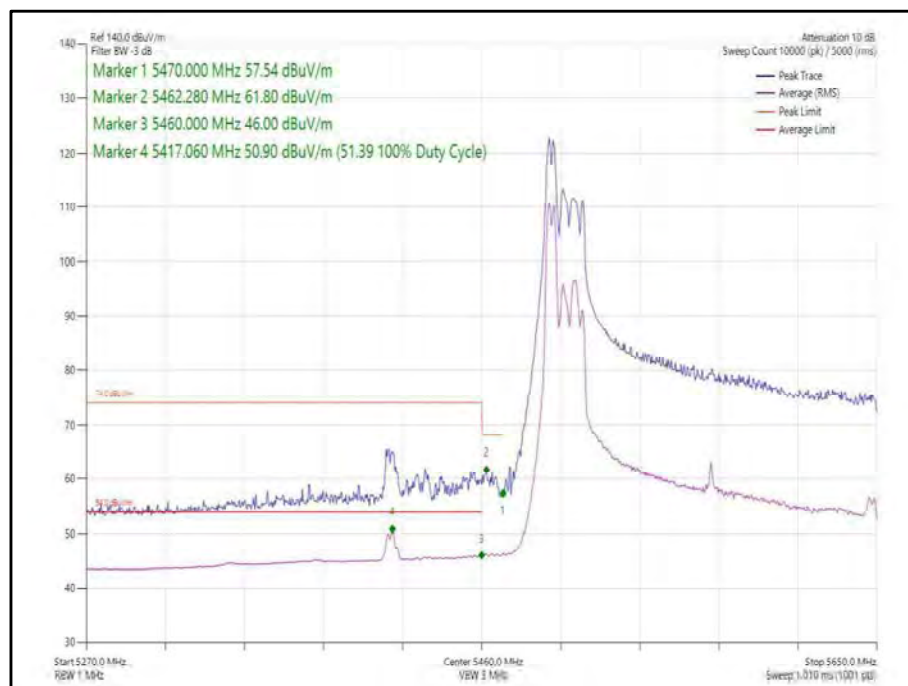
Figure 172 - 802.11ax, HE160, RU 52-37, SDM, Core 0-1 - 5570 MHz, Band Edge Frequency 5460 MHz
