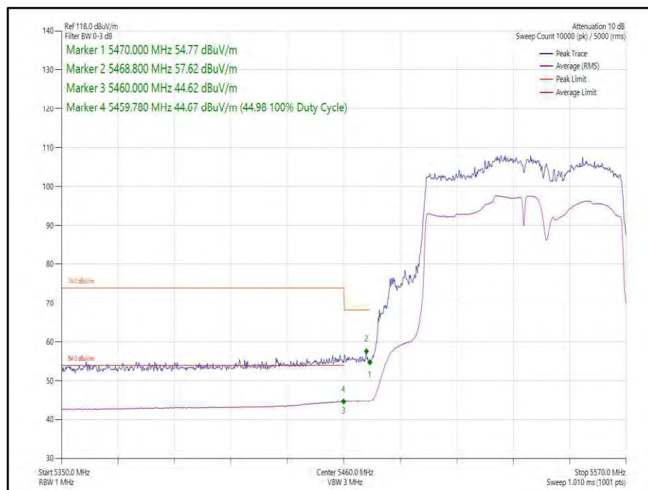
Figure 135 - 802.11ac, VHT80, TxBF, Core 0-1 - 5530 MHz, Band Edge Frequency 5460 MHz
