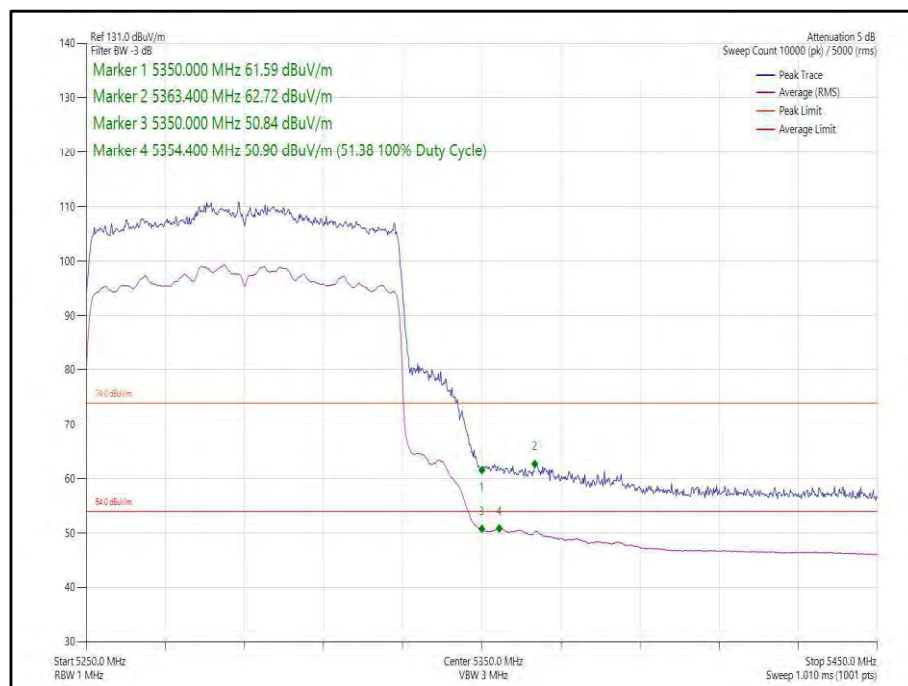
Figure 126 - 802.11ax, HE80, SU, SDM, Core 0-1 - 5290 MHz, Band Edge Frequency 5350 MHz
