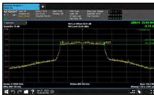
Figure 236 - 802.11n HT40 Maximum 6 dB EBW
