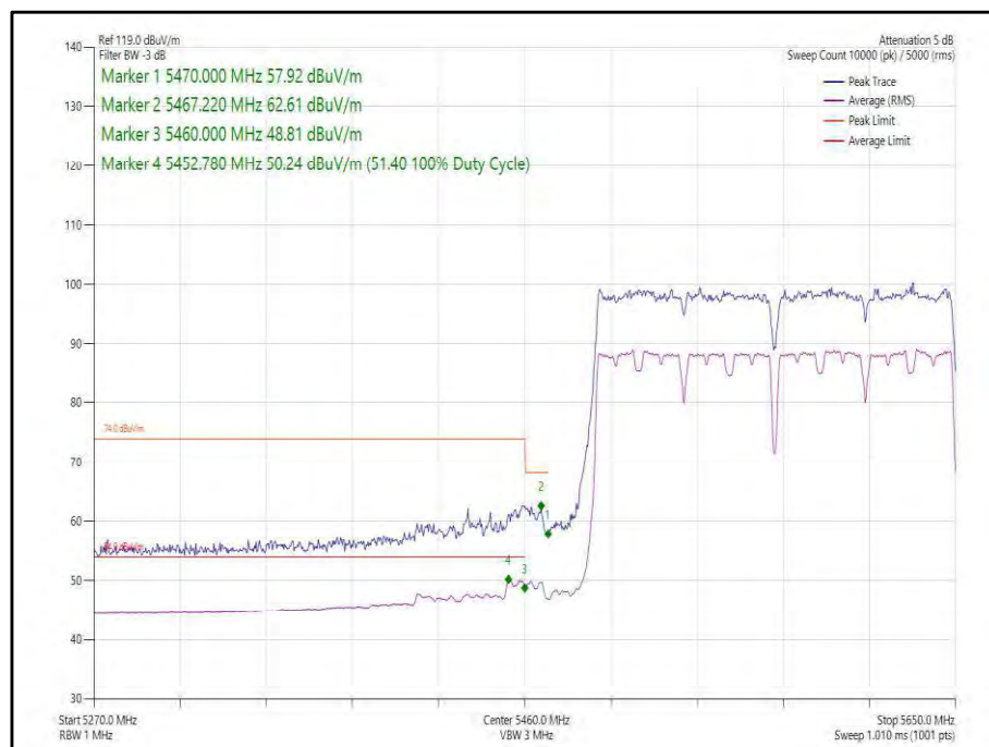
Figure 152 - 802.11ac, VHT160, SISO, Core 1 - 5570 MHz, Band Edge Frequency 5460 MHz
