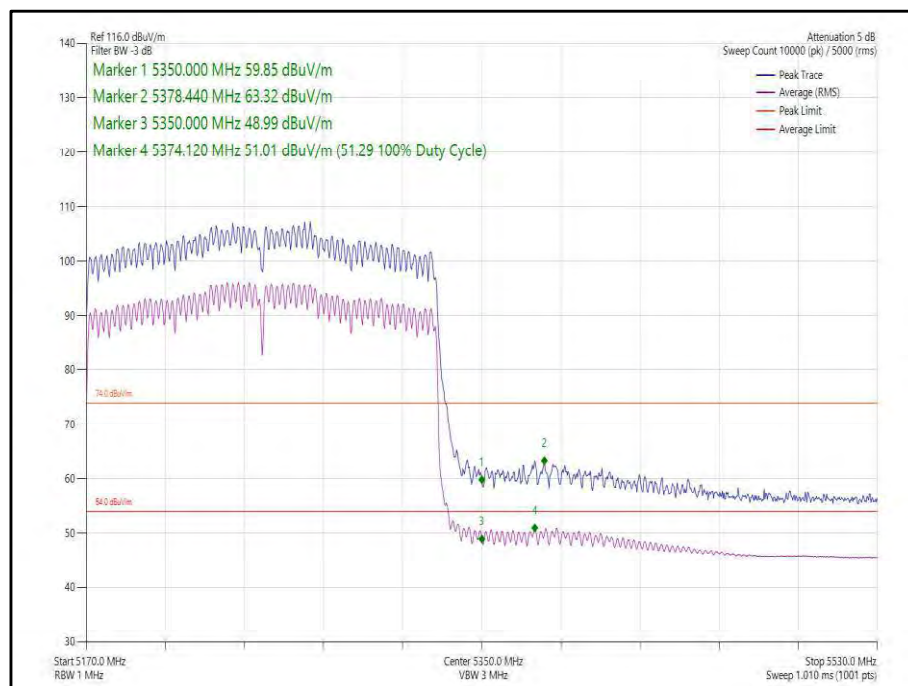
Figure 159 - 802.11ax, HE160, SU, CDD, Core 0-1 - 5250 MHz, Band Edge Frequency 5350 MHz
