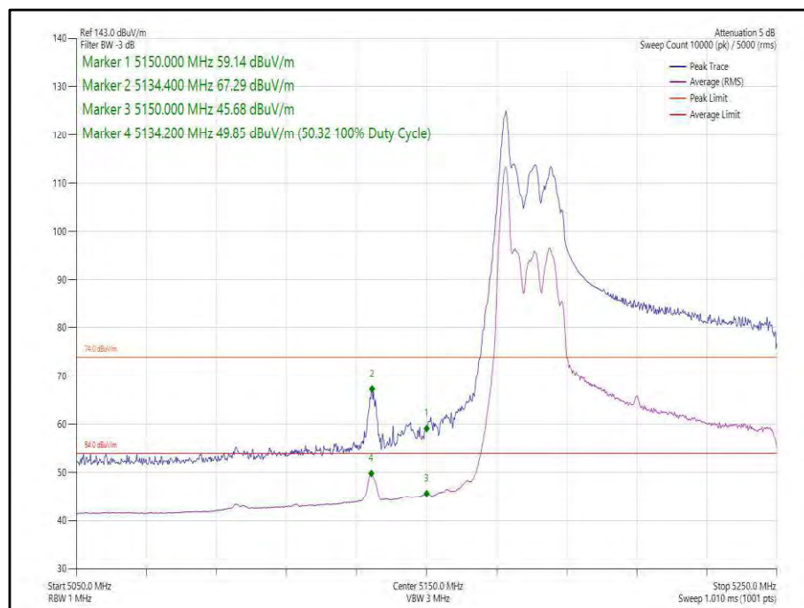
Figure 124 - 802.11ax, HE80, RU 26-0, SDM, Core 0-1 - 5210 MHz, Band Edge Frequency 5150 MHz
