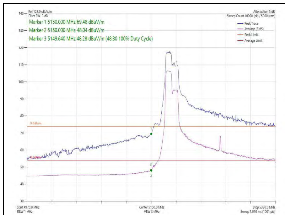
Figure 148 - 802.11ax, HE160, RU 106-53, SISO, Core 1 - 5250 MHz, Band Edge Frequency 5150 MHz
