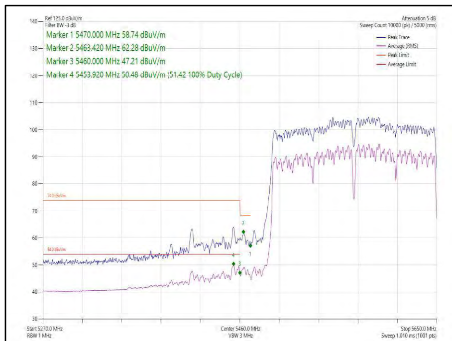
Figure 161 - 802.11ac, VHT160, CDD, Core 0-1 - 5570 MHz, Band Edge Frequency 5460 MHz
