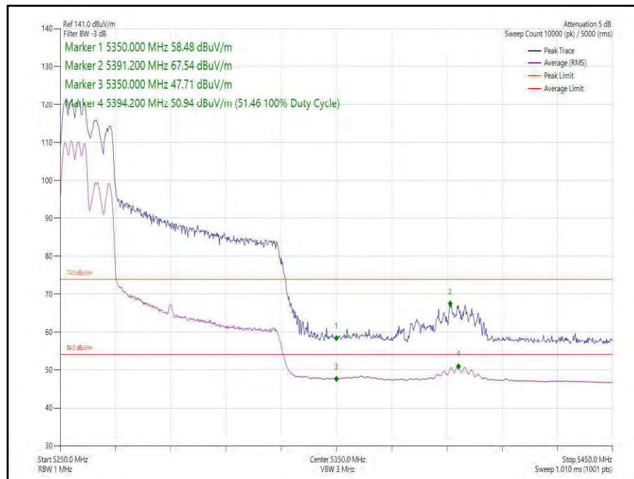
Figure 127 - 802.11ax, HE80, RU 106-53, SDM, Core 0-1 - 5290 MHz, Band Edge Frequency 5350 MHz
