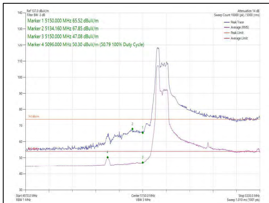
Figure 139 - 802.11ax, HE160, RU 52-37, SISO, Core 0 - 5250 MHz, Band Edge Frequency 5150 MHz
