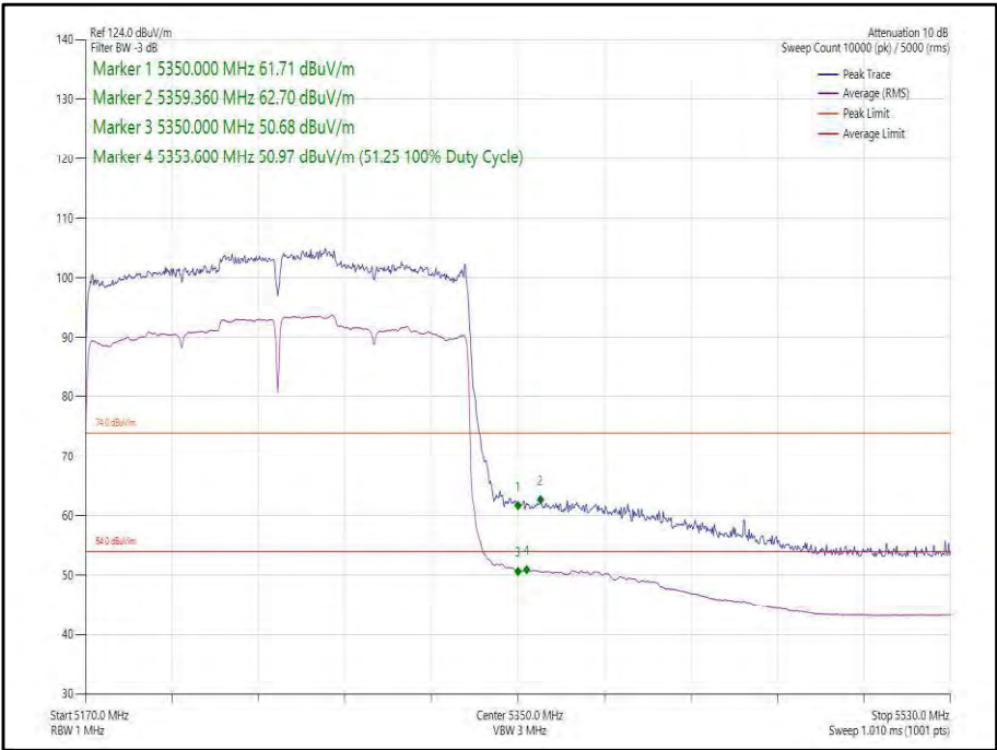
Figure 141 - 802.11ax, HE160, SU, SISO, Core 0 - 5250 MHz, Band Edge Frequency 5350 MHz
