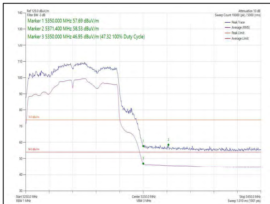
Figure 133 - 802.11ac, VHT80, TxBF, Core 0-1 - 5290 MHz, Band Edge Frequency 5350 MHz
