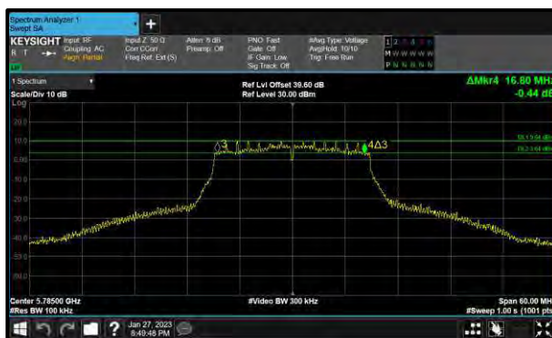
Figure 205 - 802.11n HT20 Minimum 6 dB EBW
