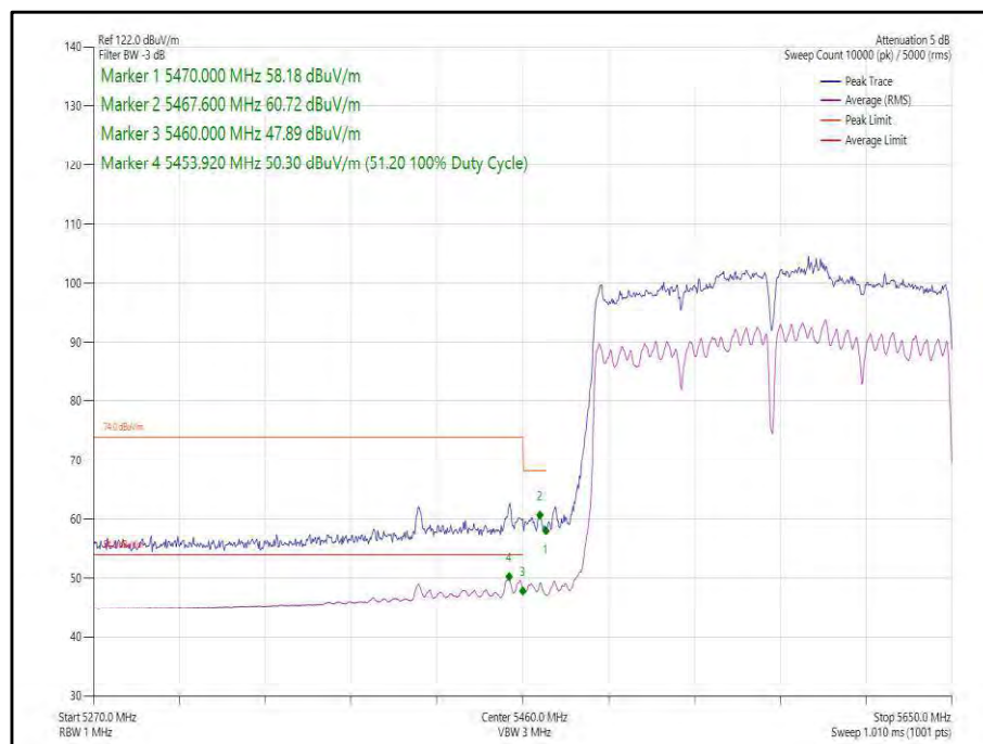
Figure 170 - 802.11ac, VHT160, SDM, Core 0-1 - 5570 MHz, Band Edge Frequency 5460 MHz
