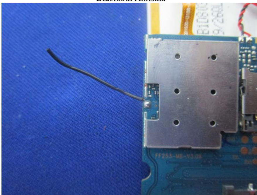
Bluetooth Antenna
