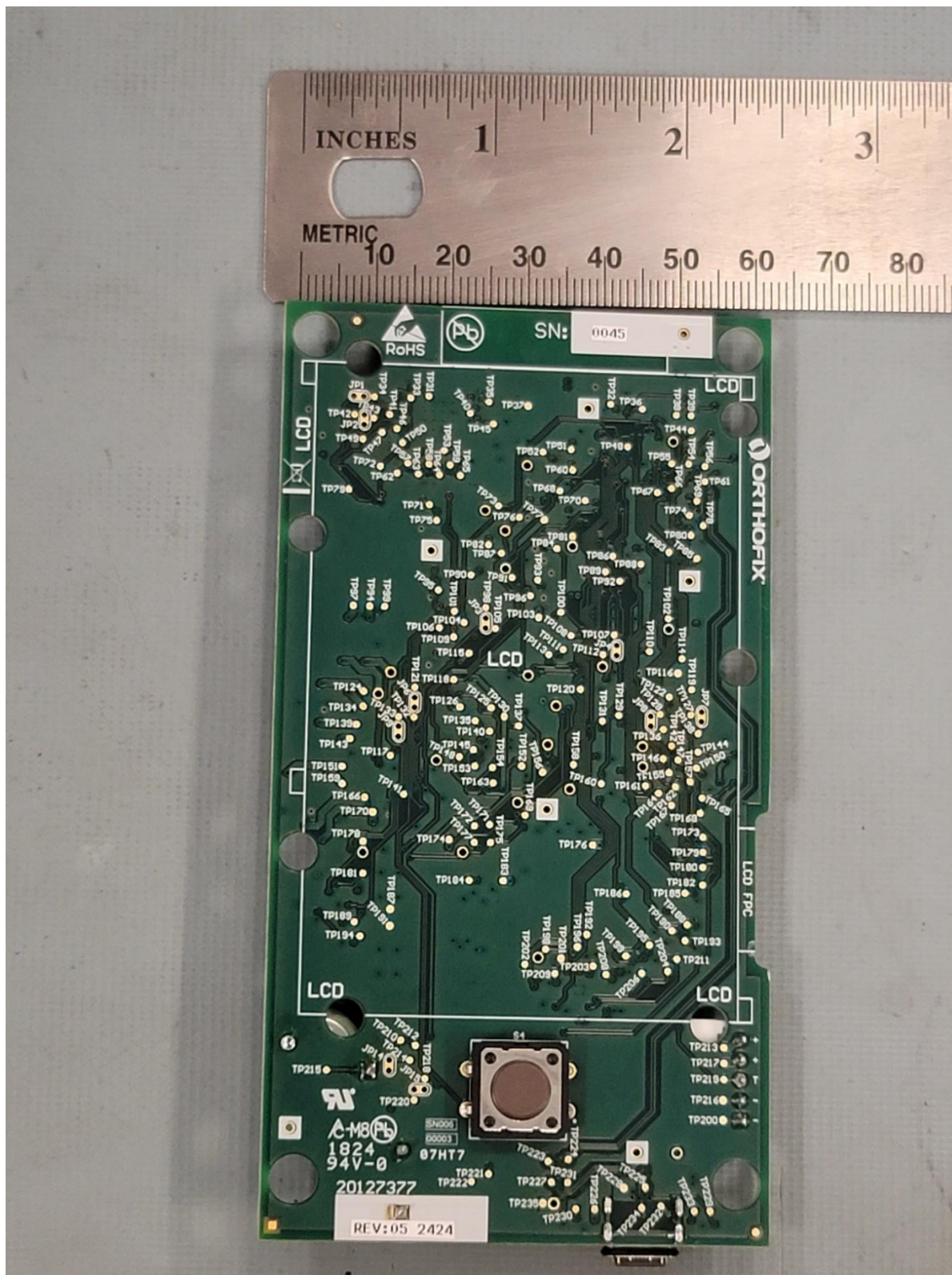
Model 4301 Internal Photo – PCA Rear
