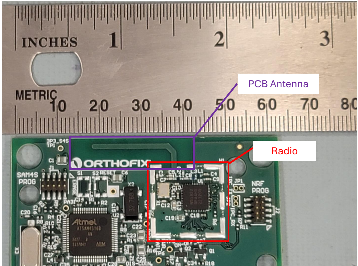
Model 4301 Internal Photo – PCA Radio Section and PCB Antenna
