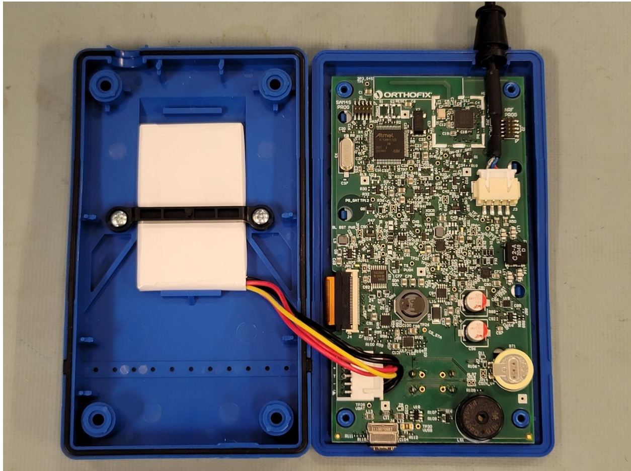
Model 4301 Internal Photo – Assembly
