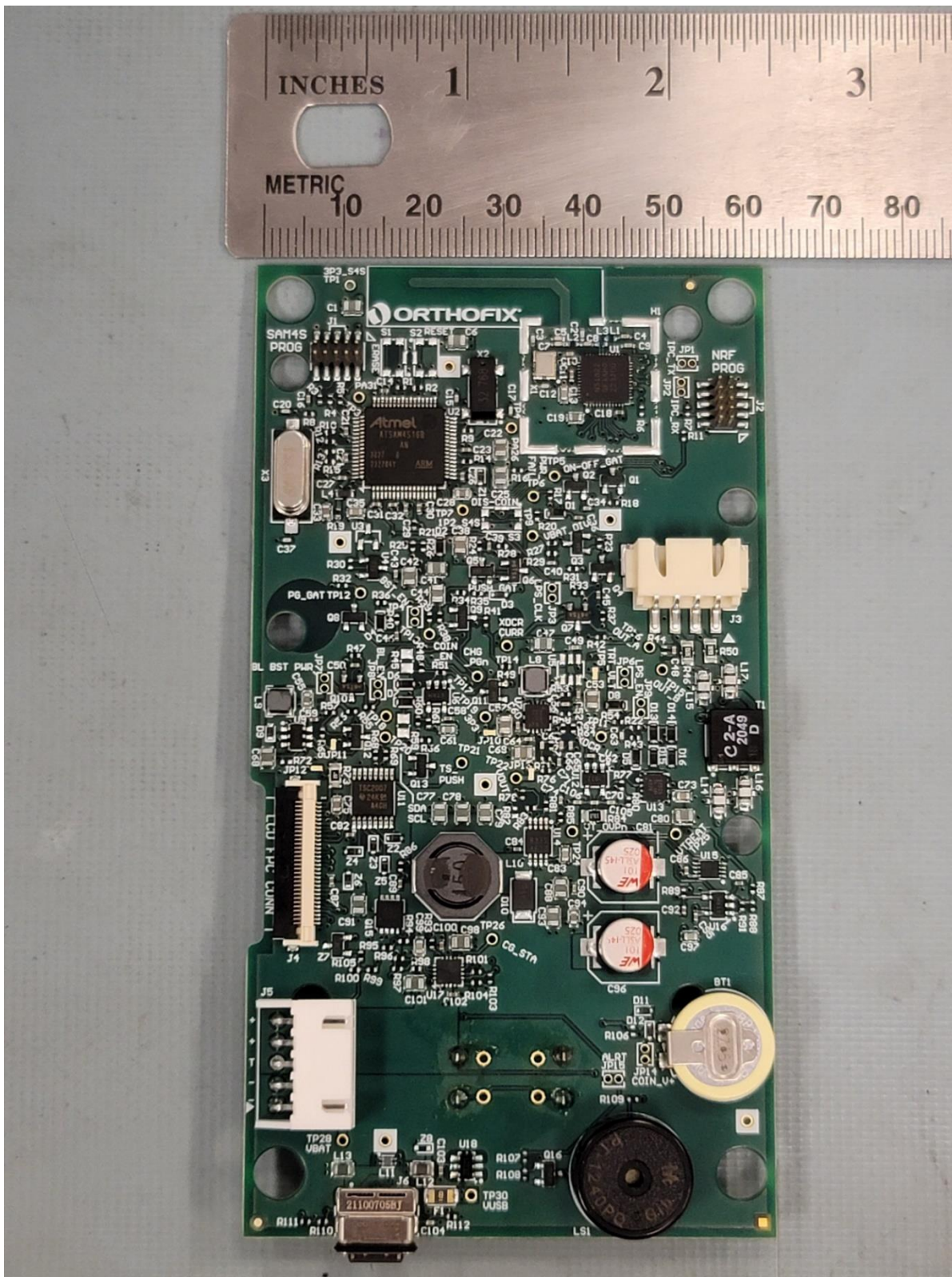
Model 4301 Internal Photo – PCA Front
