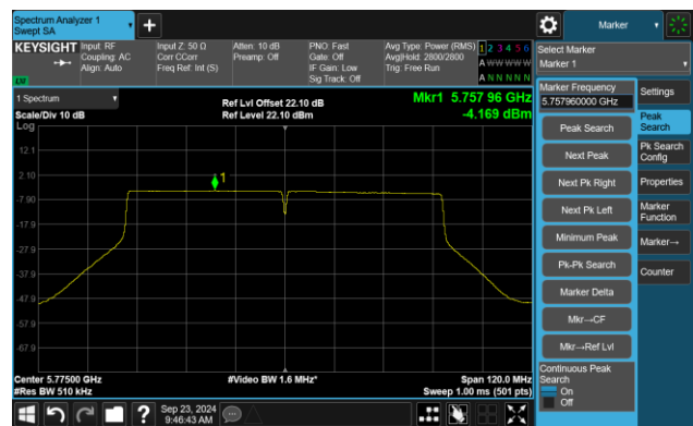
Channel 155 (5775MHz)
