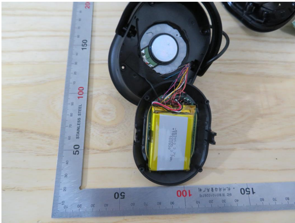
Internal View of EUT-5(right earbud)
