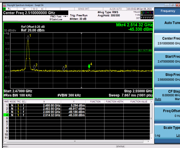
BLE_BT4.2_Ant1_High_2480
