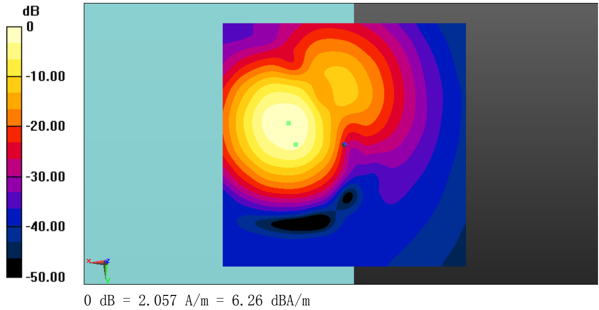
Fig B.14 T-Coil LTE B4
