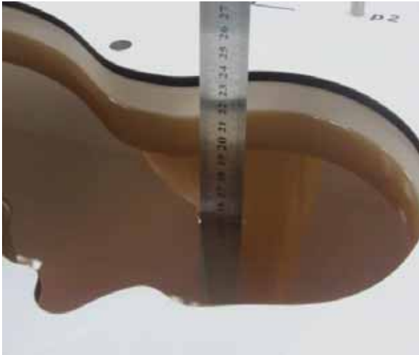
Photo 25: HBBL600-6000MHz Depth (15.1cm)
