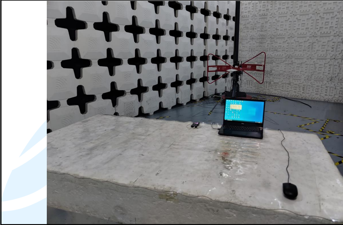
Radiated emission Test Setup-1 (30 MHz~1 GHz)
