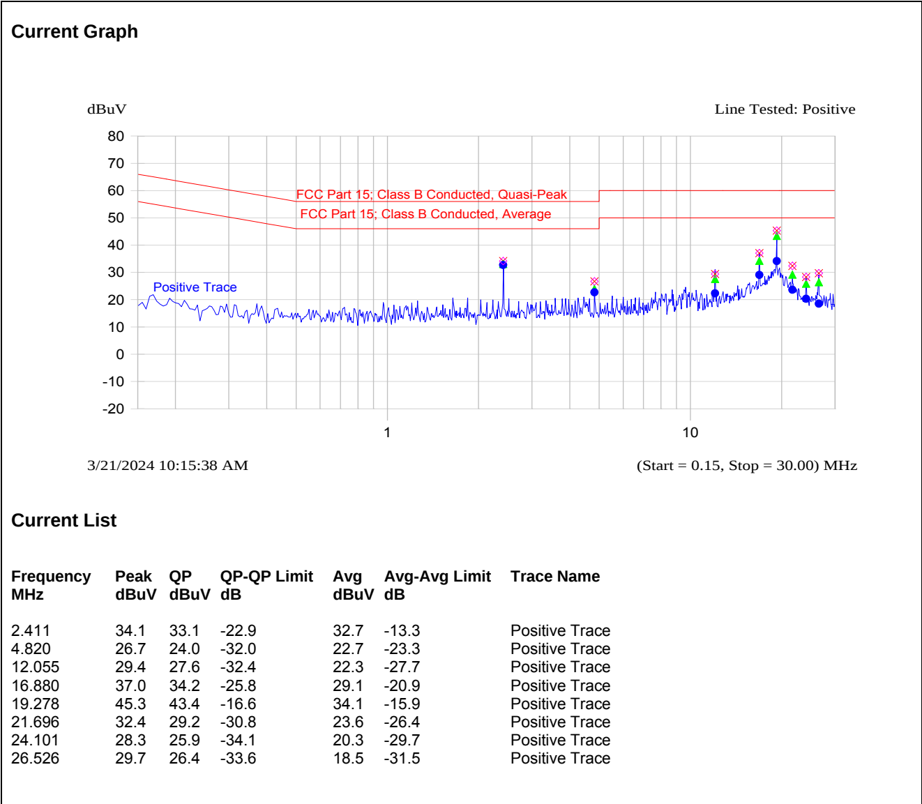
Plot 5.1.4.9. XB-9XR-DMUT-001 Power Line Conducted Emissions (Tx Mode) Line Voltage: 3.6 VDC; Line Tested: Positive
