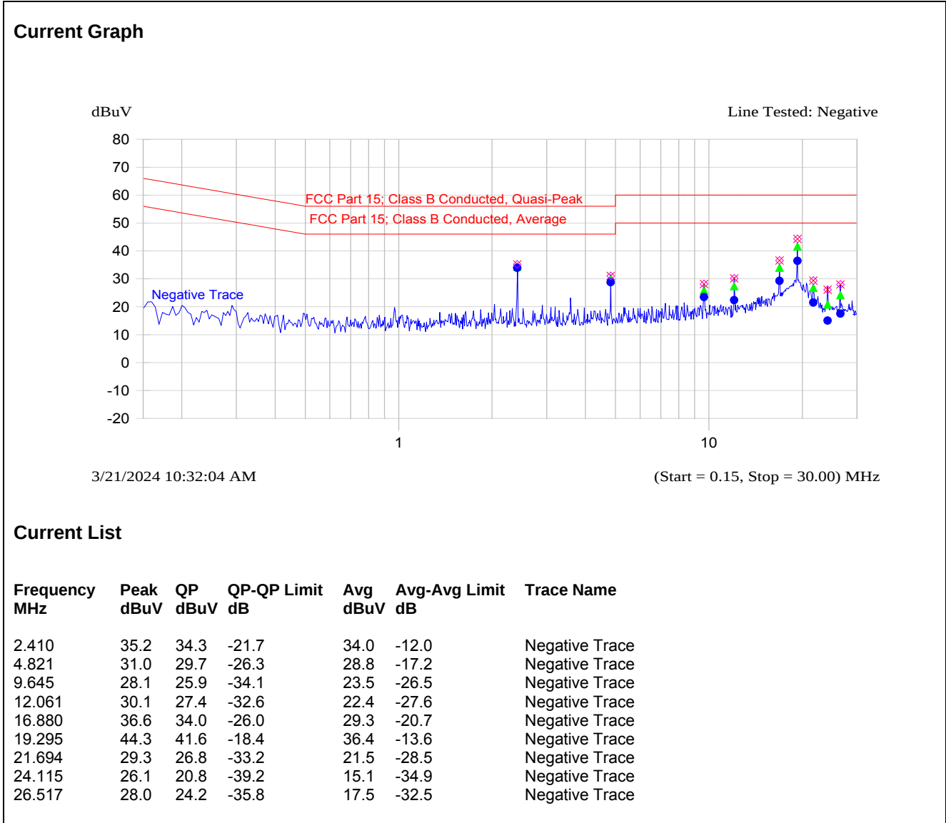
Plot 5.1.4.14. XB-9XR-DMST-001 Power Line Conducted Emissions (Tx Mode) Line Voltage: 3.6 VDC; Line Tested: Negative
