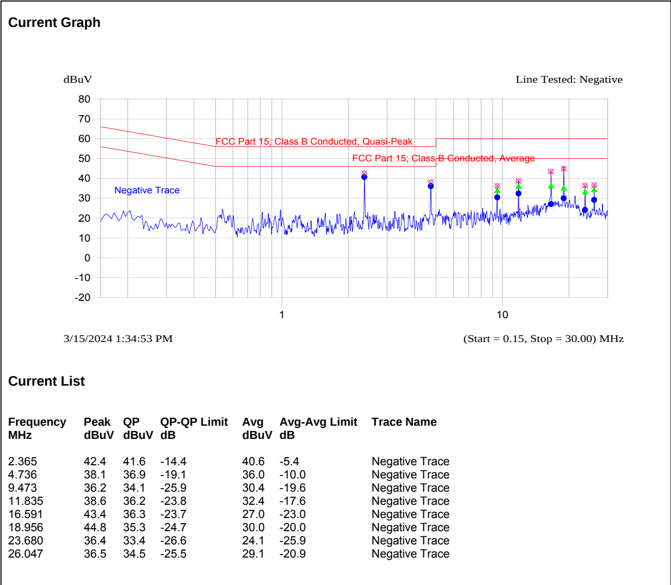
Plot 5.1.4.8. XB-9XR-DMUS-001 Power Line Conducted Emissions (Rx Mode) Line Voltage: 3.6 VDC; Line Tested: Negative
