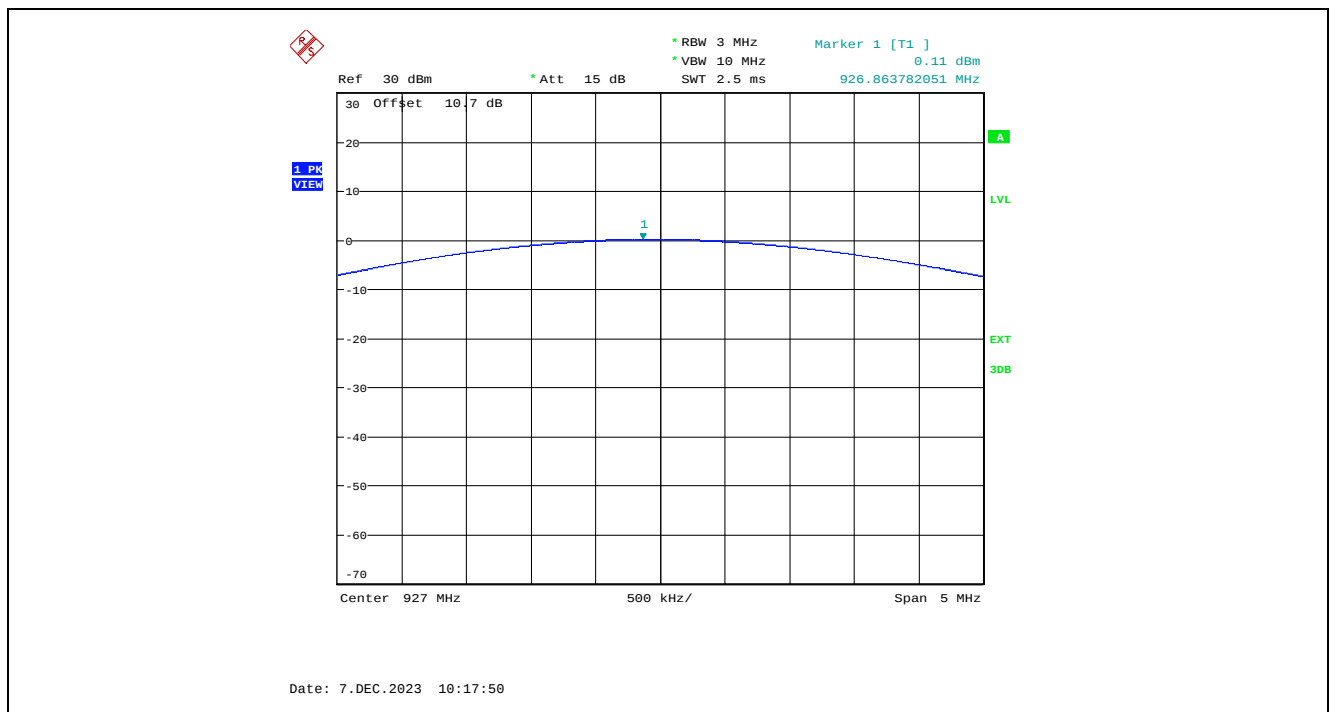
Plot 5.4.4.1.12. XB-9XR-DMUM-001 Maximum Peak Conducted Output Power, Low Power Setting, 10 kbps, 927 MHz
