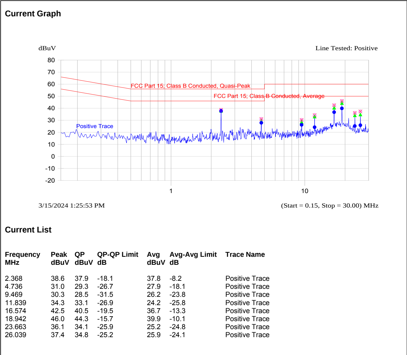
Plot 5.1.4.7. XB-9XR-DMUS-001 Power Line Conducted Emissions (Rx Mode) Line Voltage: 3.6 VDC; Line Tested: Positive
