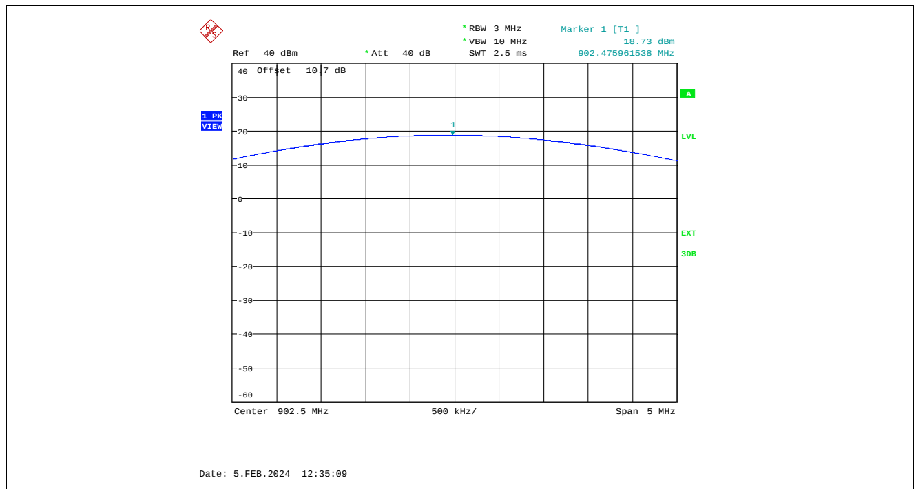
Plot 5.4.4.3.4. XB-9XR-DMUT-001 - Maximum Peak Conducted Output Power, High Power Setting, 110 kbps, 902.5 MHz
