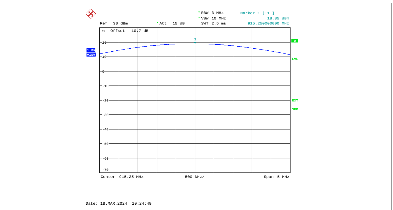
Plot 5.4.4.2.8. XB-9XR-DMUS-001 - Maximum Peak Conducted Output Power, High Power Setting, 250 kbps, 915.25 MHz
