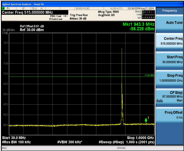
Band13_5MHz_QPSK_23255_1RB#0_30~1000_30~1000
