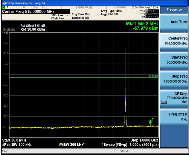
Band13_5MHz_16QAM_23255_1RB#0_30~1000_30~1000
