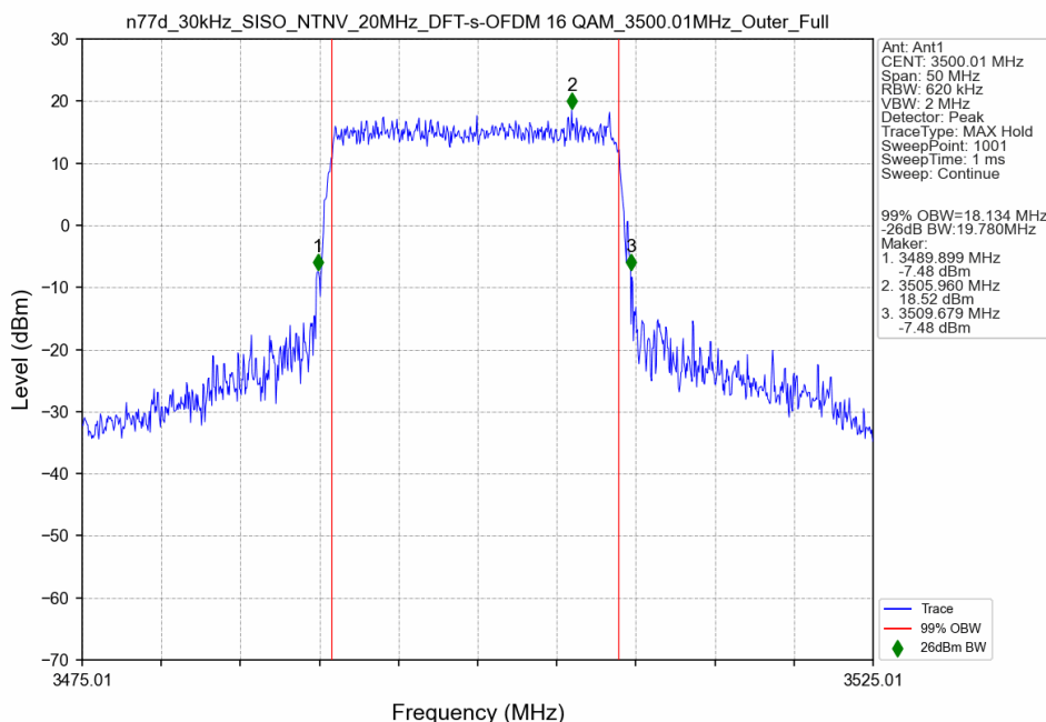
n77d_30kHz_SISO_NTNV_20MHz_DFT-s-OFDM 16 QAM_3500.01MHz_Outer_Full
