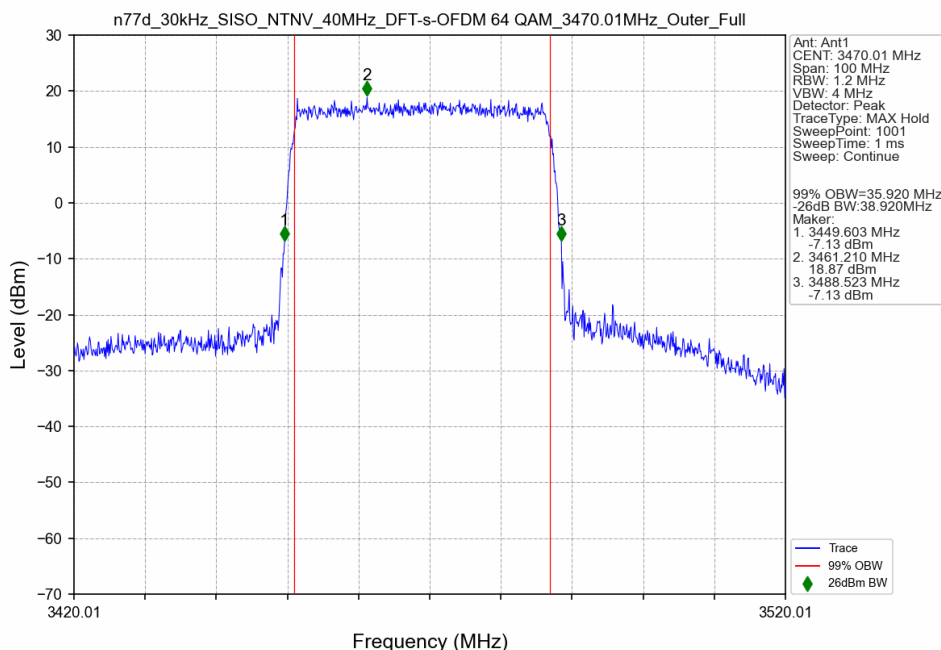
n77d_30kHz_SISO_NTNV_40MHz_DFT-s-OFDM 64 QAM_3470.01MHz_Outer_Full
