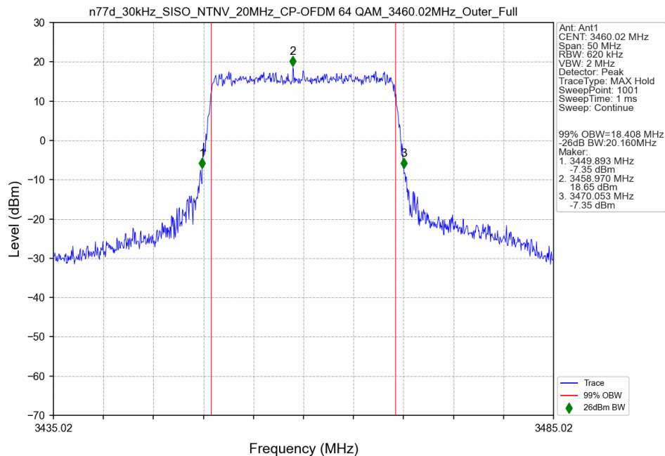
n77d_30kHz_SISO_NTNV_20MHz_CP-OFDM 64 QAM_3460.02MHz_Outer_Full
