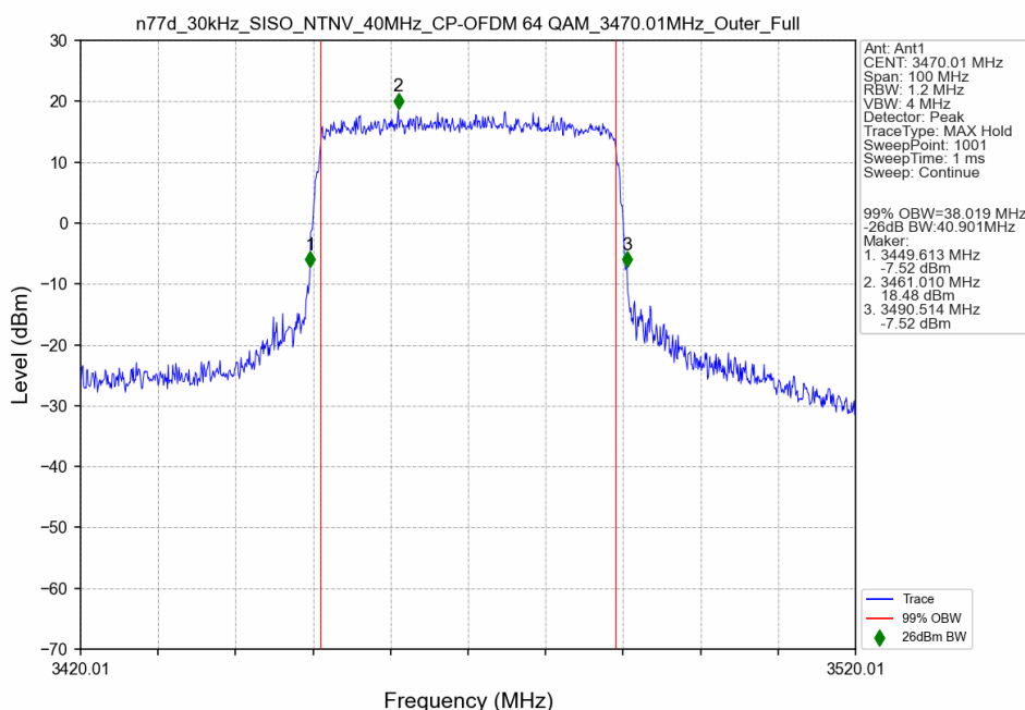
n77d_30kHz_SISO_NTNV_40MHz_CP-OFDM 64 QAM_3470.01MHz_Outer_Full
