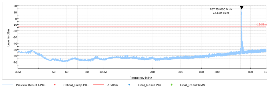
Plot #27 Radiated Emissions: 30 MHz – 1GHz
