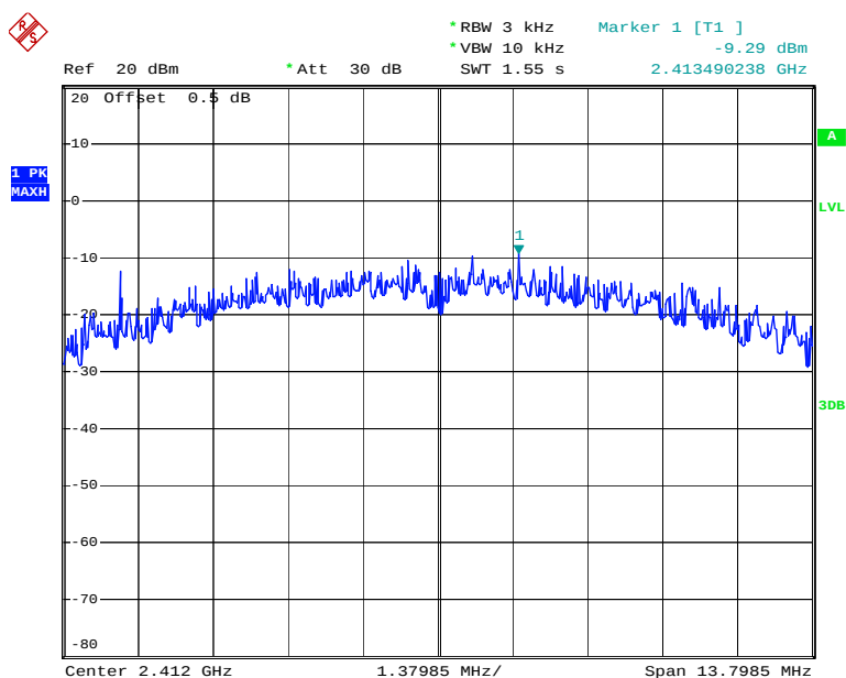
Chain 0, Power Spectral Density, 802.11b Low Channel
