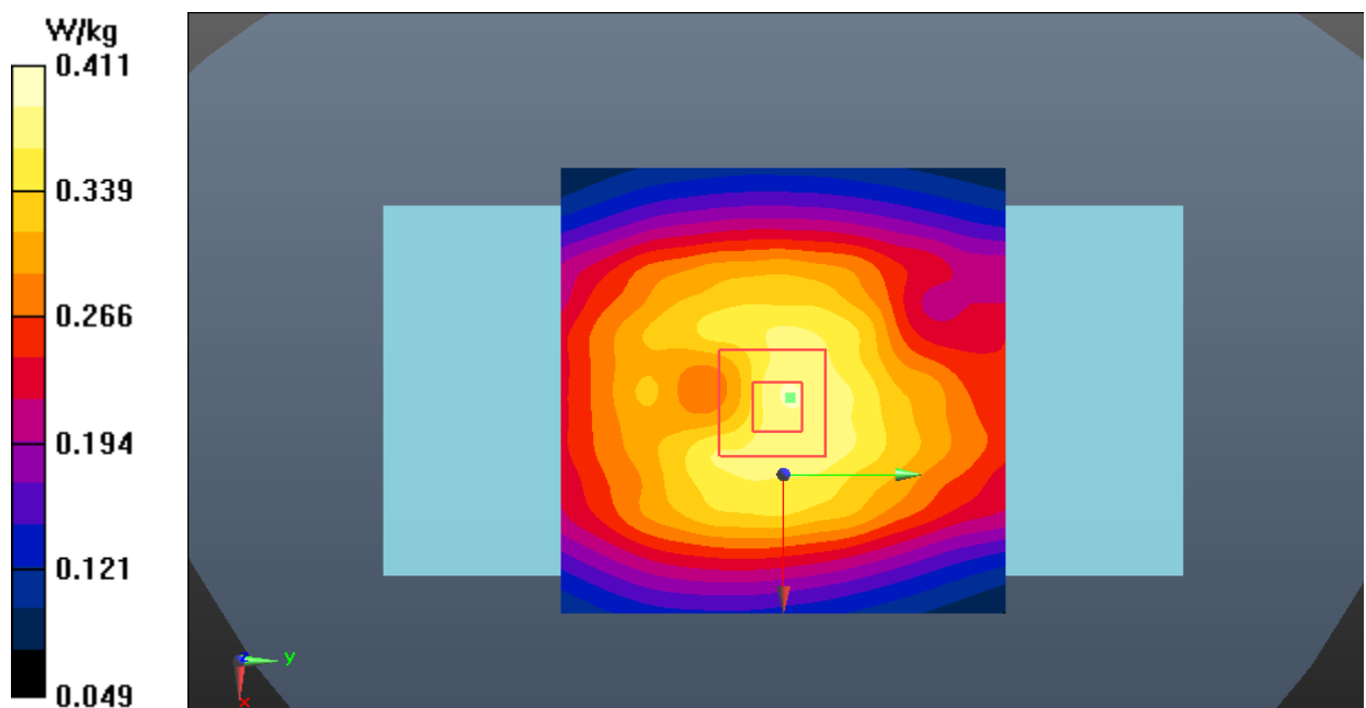
Fig.20 LTE Band 12 Body
