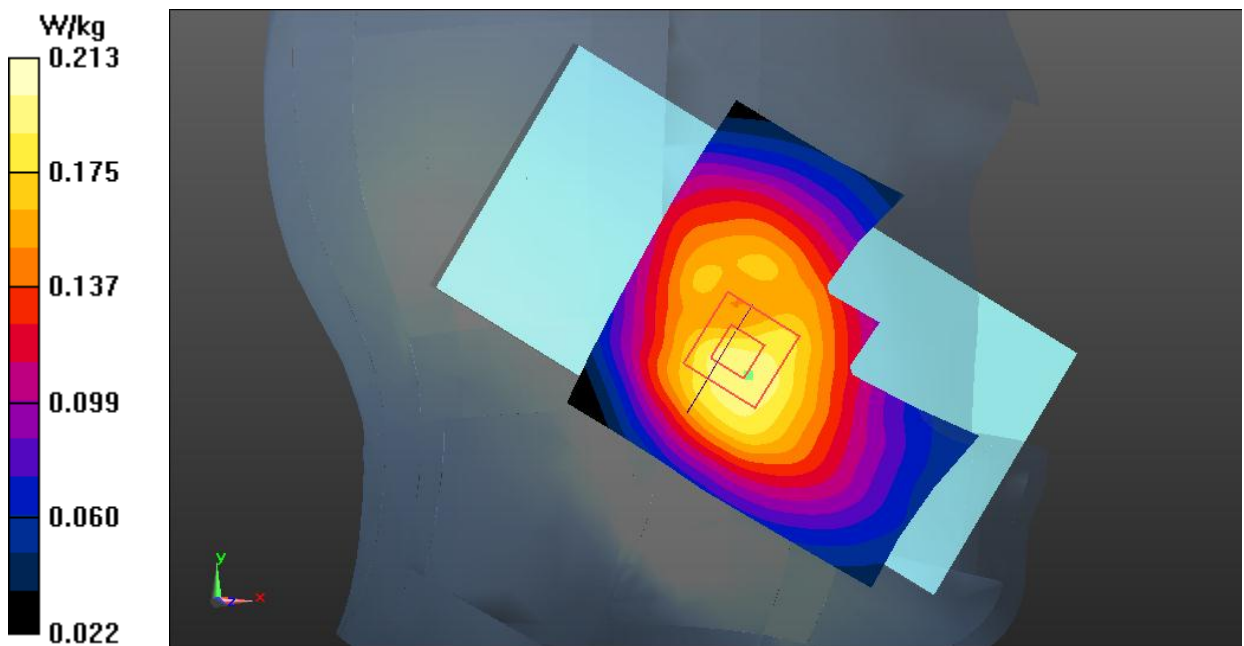
Fig.19 LTE Band 12 Head
