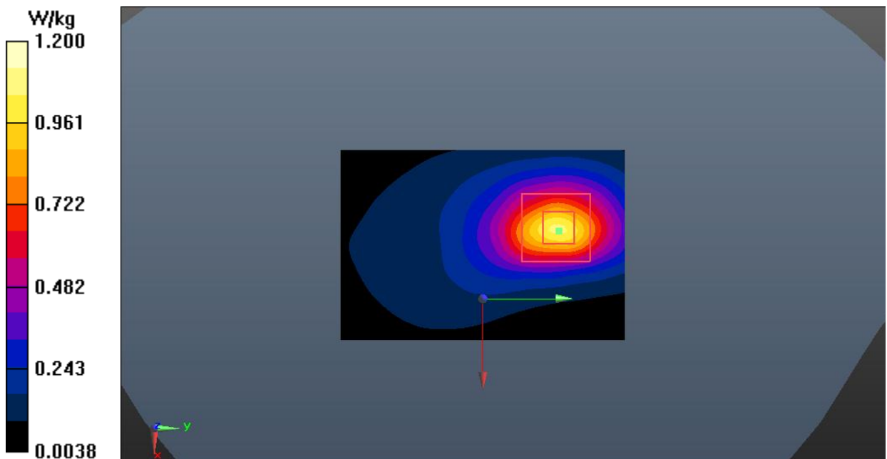
Fig.18 LTE Band 7 Body
