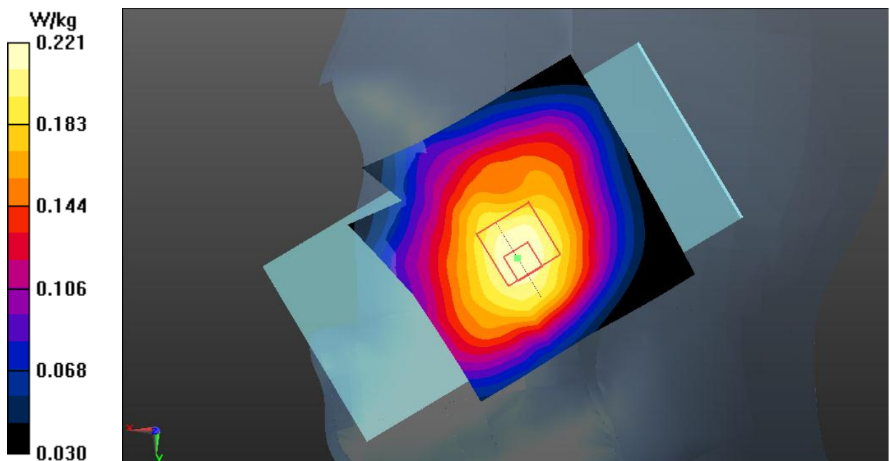
Fig.21 LTE Band 17 Head
