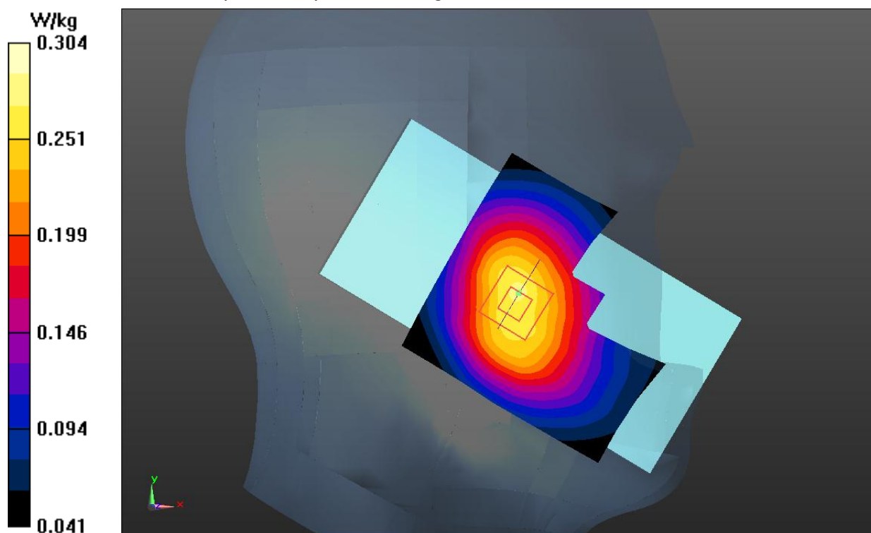
Fig.1 GSM 850 Head
