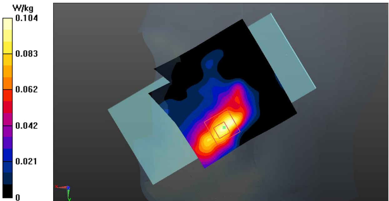
Fig.17 LTE Band 7 Head
