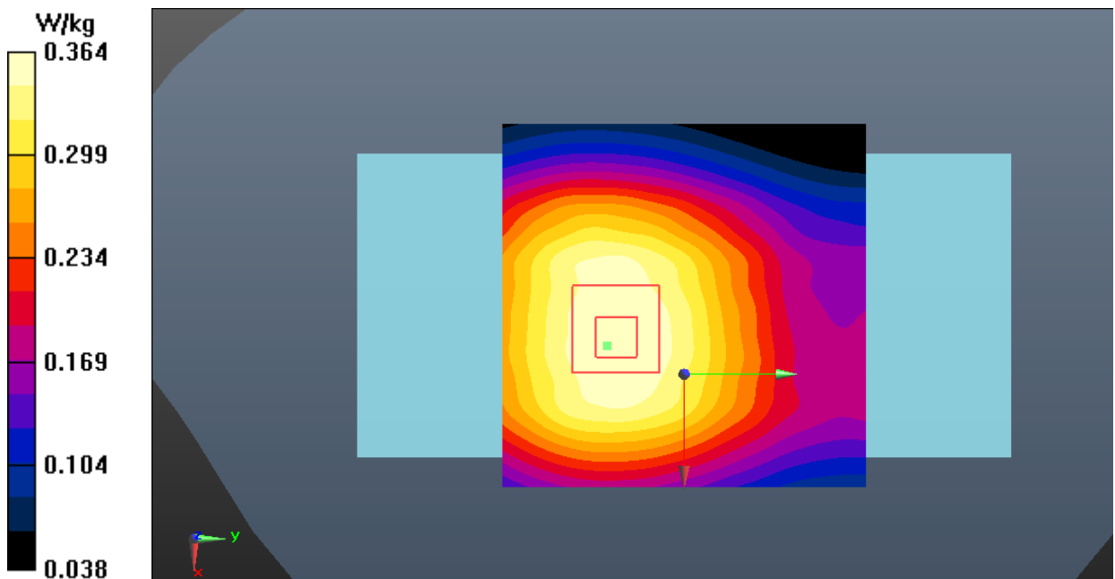
Fig.16 LTE Band 5 Body
