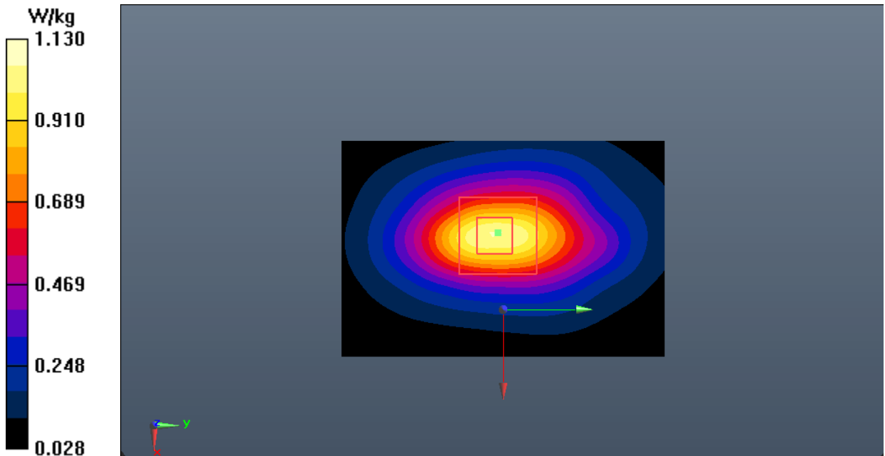
Fig.24 LTE Band 66 Body
