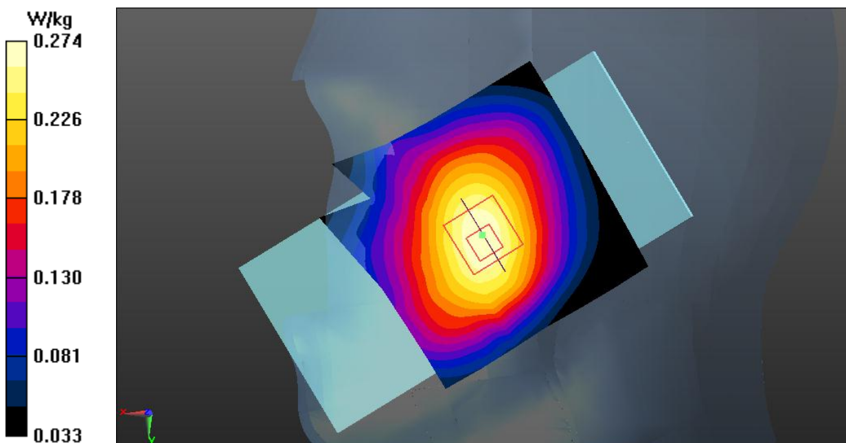
Fig.15 LTE Band 5 Head
