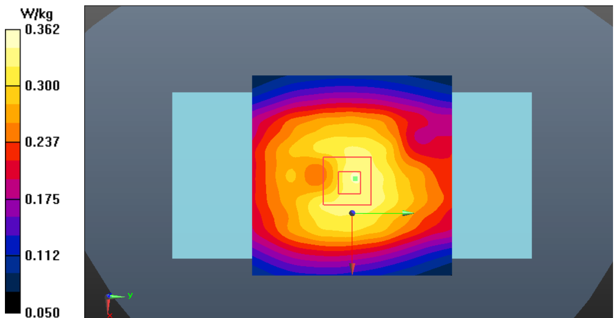
Fig.22 LTE Band 17 Body
