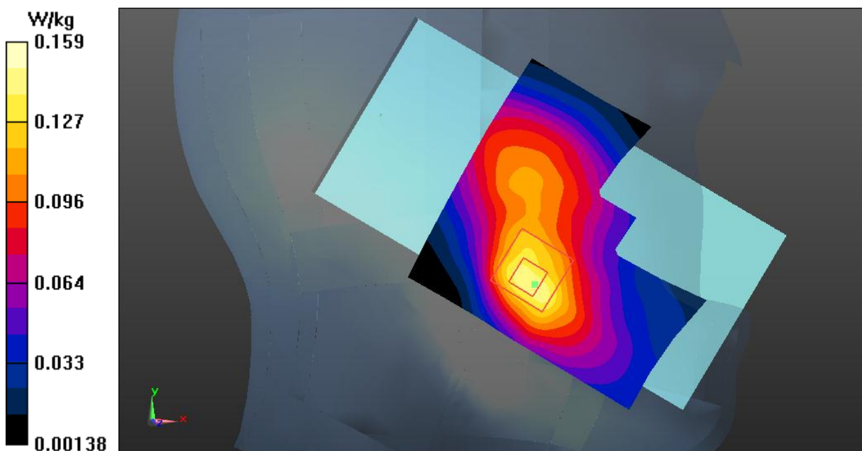
Fig.3 GSM 1900 Head
