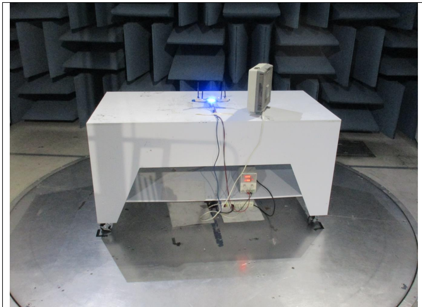
Back Radiated Emissions Below 1GHz FCC B
