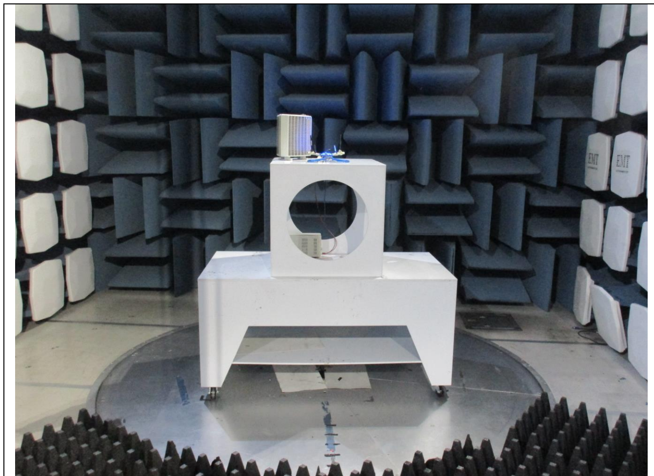
Front Radiated Emissions Above 1GHz FCC B
