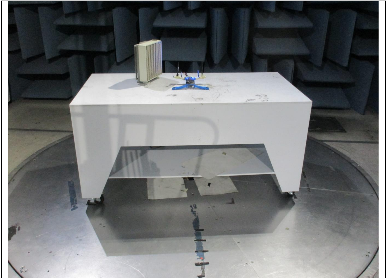
Front Radiated Emissions Below 1GHz FCC B
