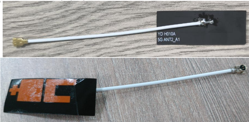
Figure 1 Antenna
