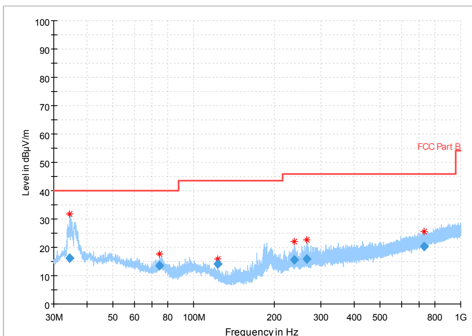
Fig.50 Radiated Spurious Emission (802.11g, Ch11, 30MHz~1GHz)
