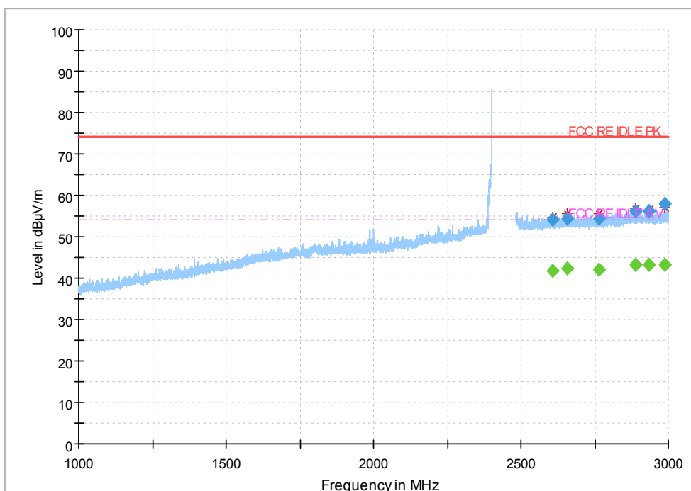
Fig.51 Radiated Spurious Emission (802.11g, Ch11, 1GHz~3GHz)
