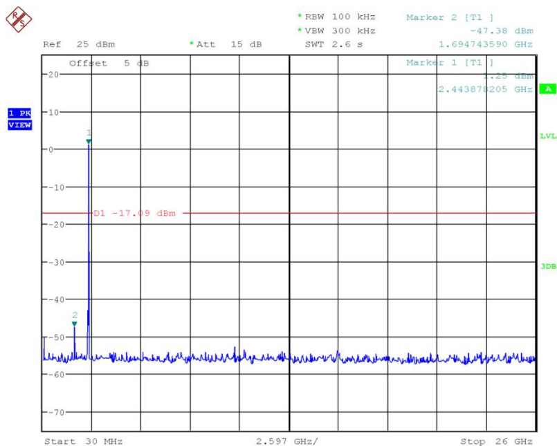
Fig.41 Conducted Spurious Emission (802.11n-20MHz, Ch11)
