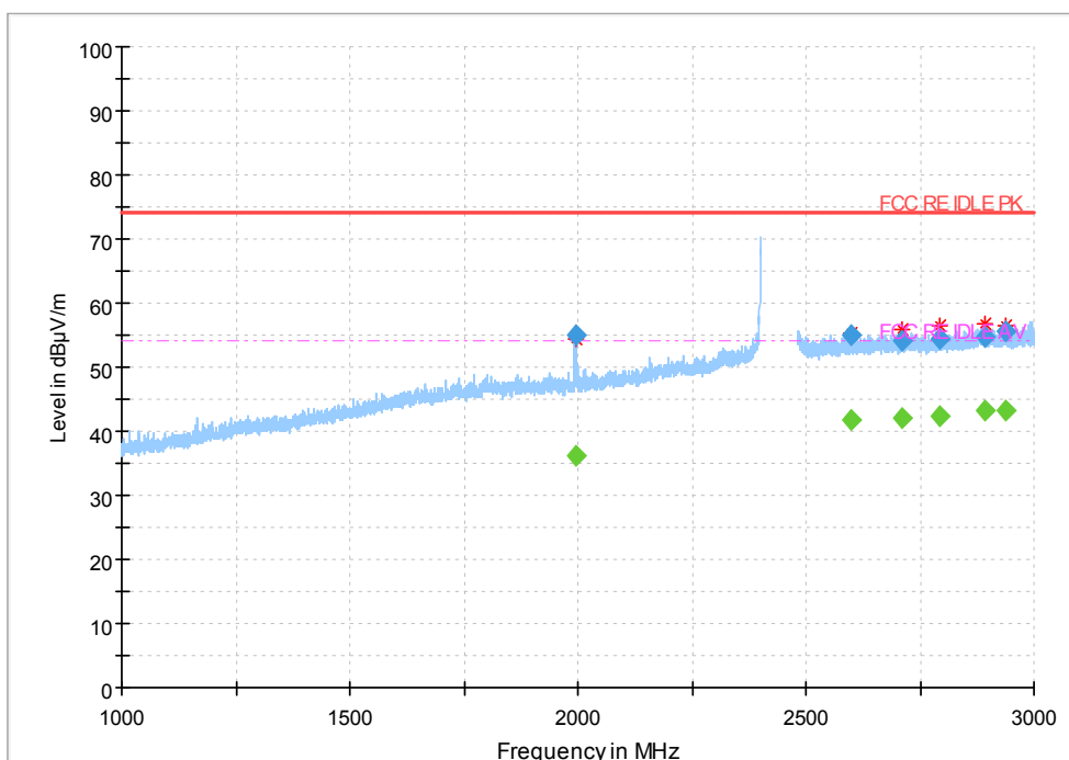
Fig.46 Radiated Spurious Emission (802.11b,Ch11,1GHz~3GHz)
