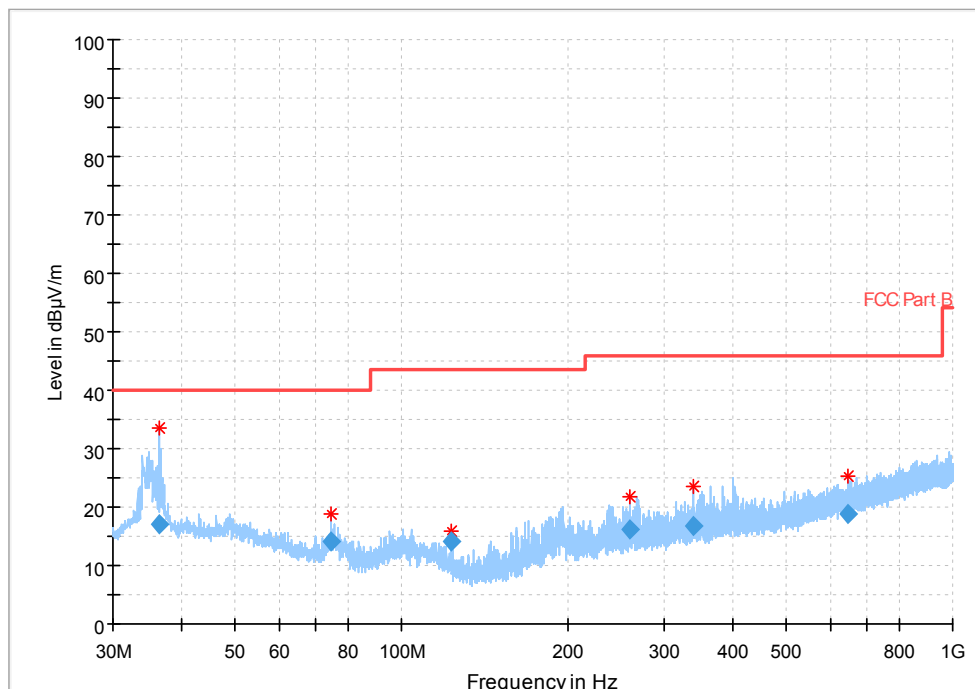
Fig.55 Radiated Spurious Emission (802.11 n-20MHz,Ch11,30MHz~1GHz)
