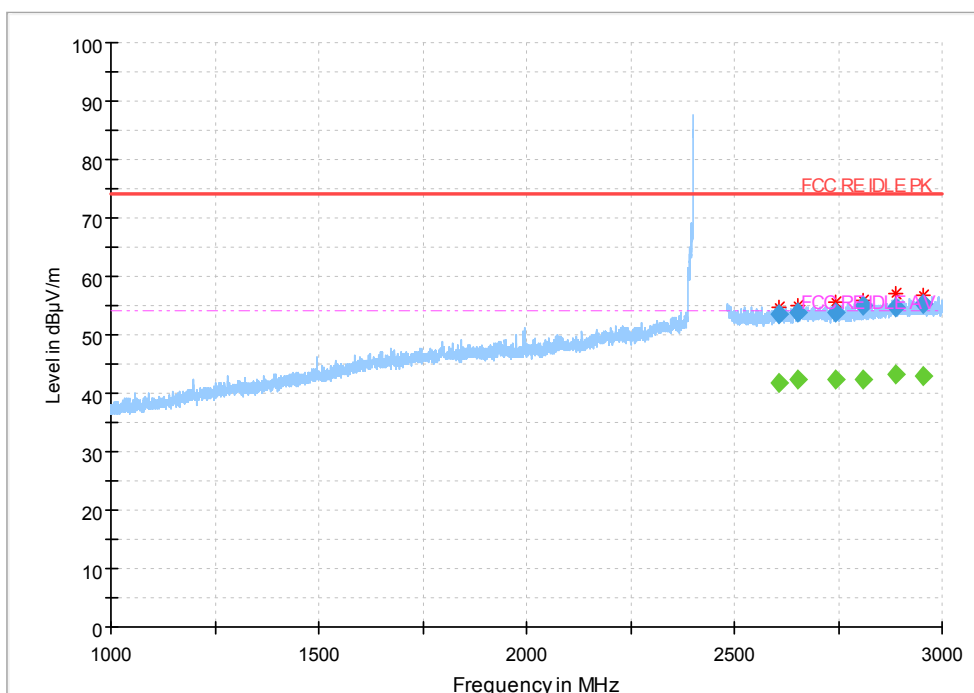
Fig.56 Radiated Spurious Emission (802.11 n-20MHz,Ch11,1GHz~3GHz)
