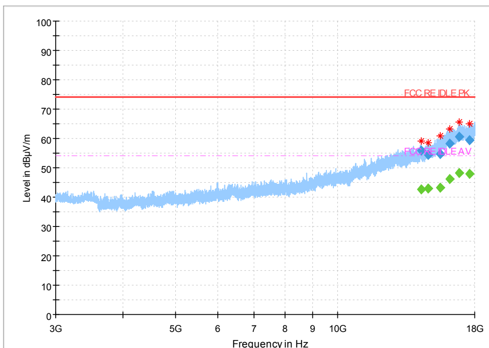
Fig.47 Radiated Spurious Emission (802.11b,Ch11,3GHz~18GHz)
