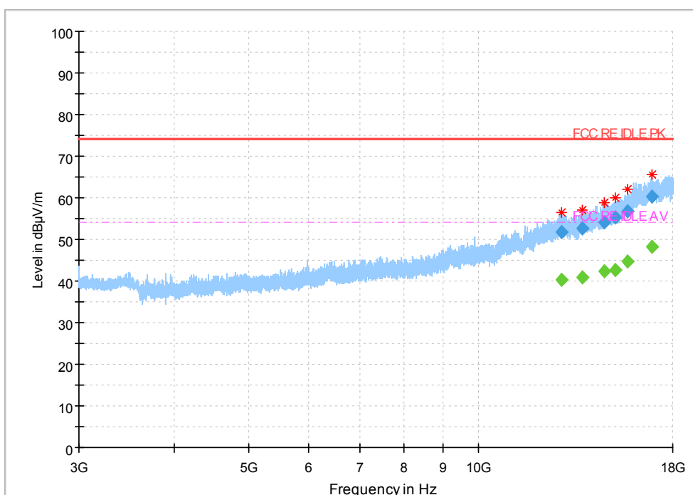
Fig.57 Radiated Spurious Emission (802.11 n-20MHz,Ch11,3GHz~18GHz)
