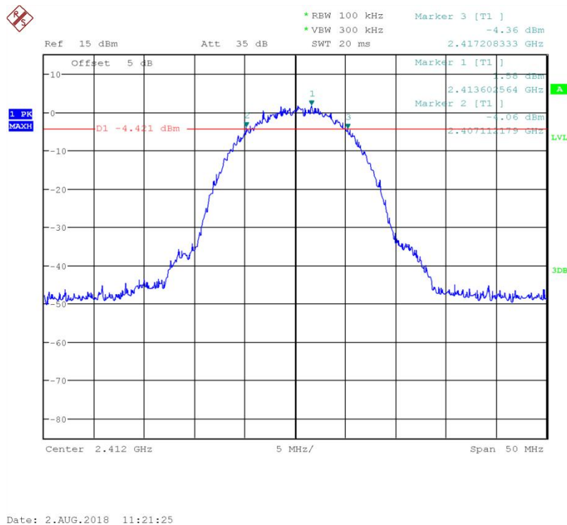
Fig.10 Occupied 6dB Bandwidth (802.11b, Ch1)
