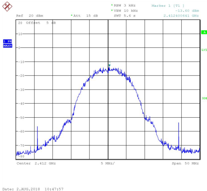
Fig 1. Power Spectral Density (802.1b,Ch1)
