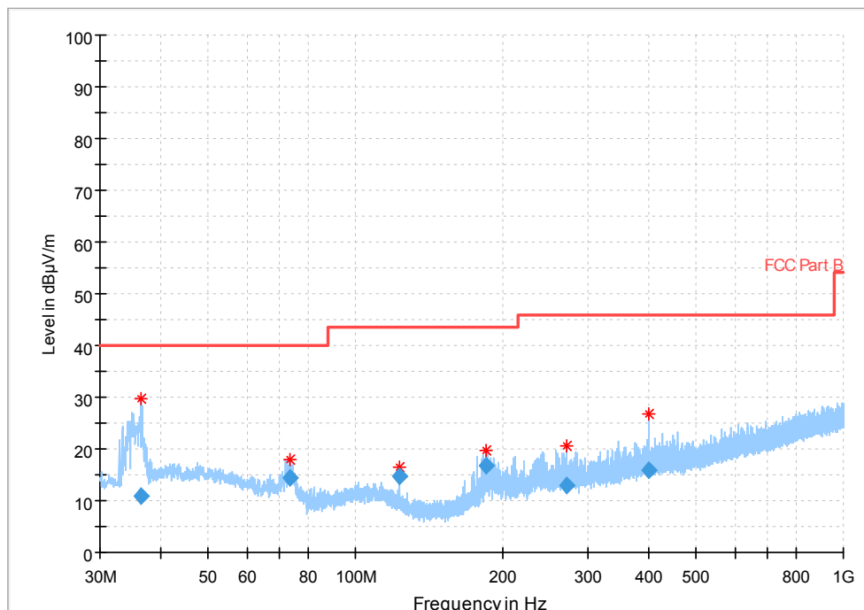
Fig.45 Radiated Spurious Emission (802.11b,Ch11,30MHz~1GHz)
