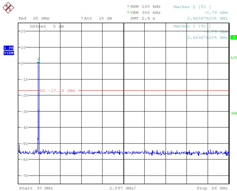
Fig.35 Conducted Spurious Emission (802.11g, Ch11)
