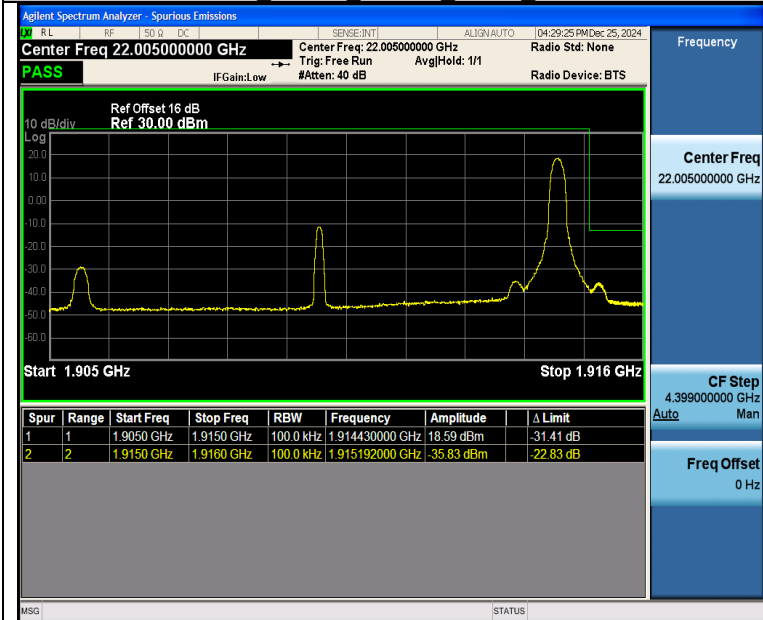
Band25_10MHz_16QAM_26640_1RB#49
