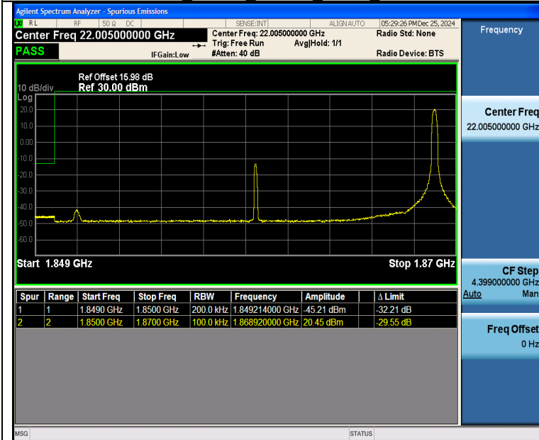
Band25_20MHz_16QAM_26140_1RB#99
