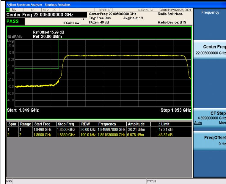
Band25 3MHz 16QAM 26055 15RB#0
