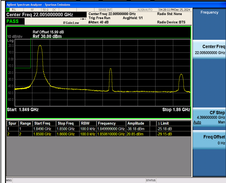
Band25 10MHz 16QAM 26090 1RB#0
