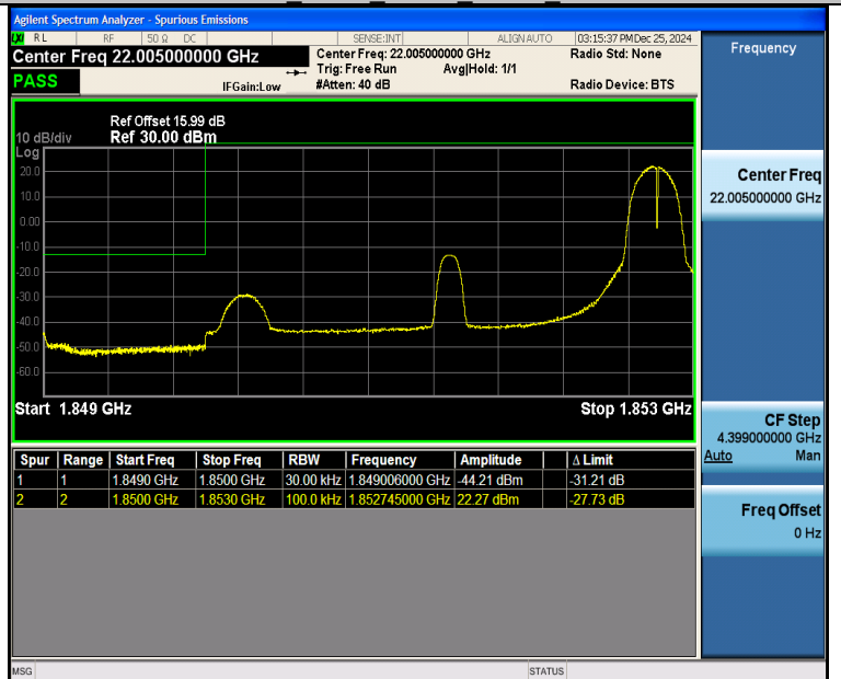
Band25_3MHz_QPSK_26055_1RB#14
