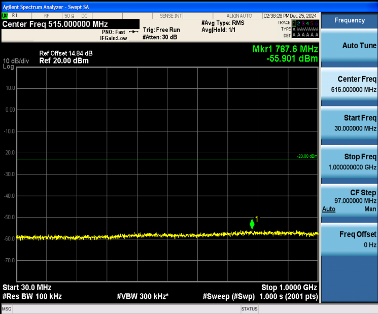
Band25_1.4MHz_QPSK_26047_1RB#0_30~1000_30~1000
