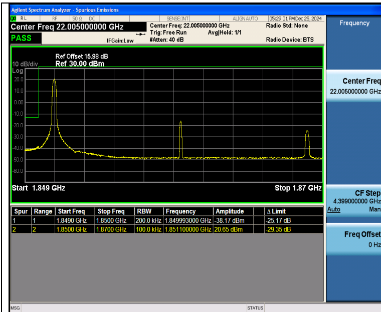
Band25_20MHz_16QAM_26140_1RB#0
