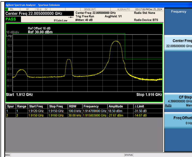
Band25 3MHz 16QAM 26675 1RB#14
