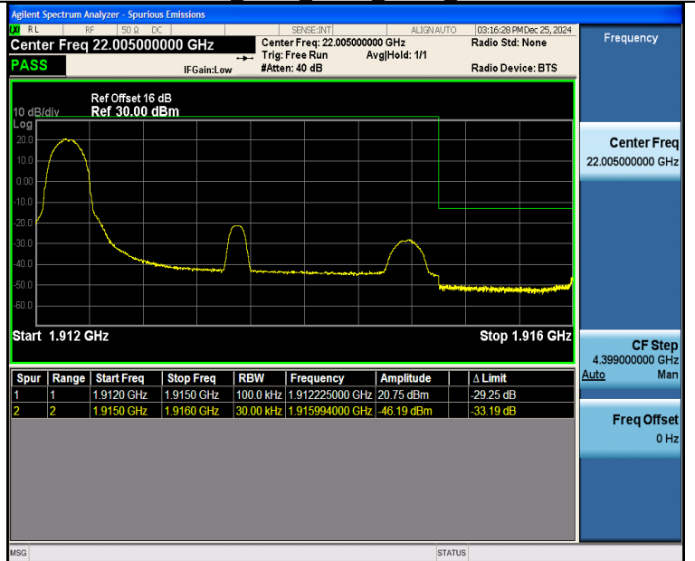
Band25 3MHz QPSK 26675 1RB#0
