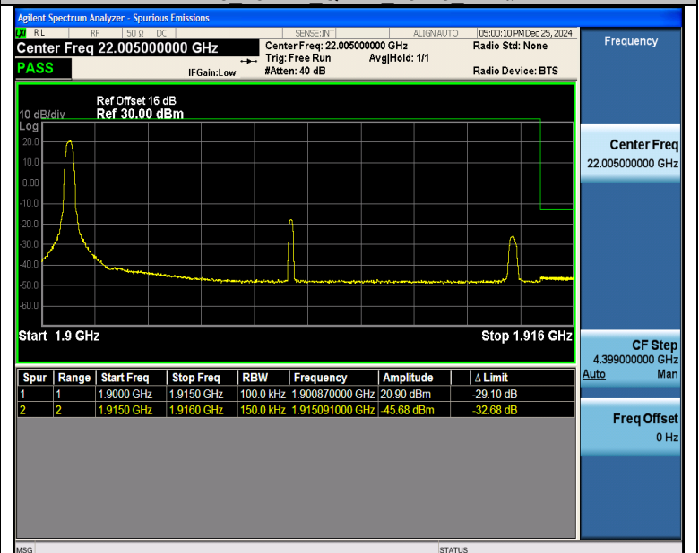
Band25_15MHz_QPSK_26615_1RB#0
