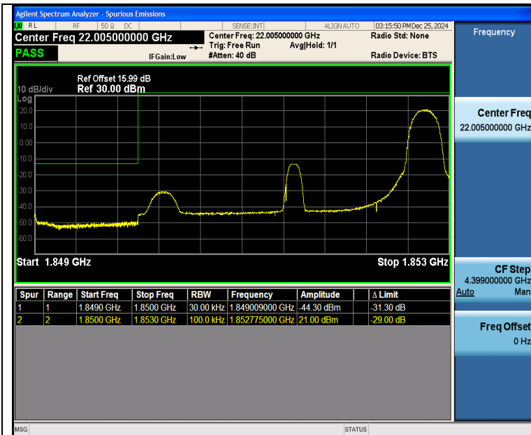
Band25 3MHz 16QAM 26055 1RB#14
