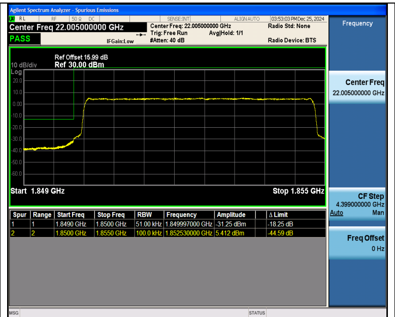
Band25 5MHz QPSK 26065 25RB#0
