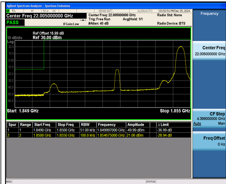
Band25 5MHz 16QAM 26065 1RB#24
