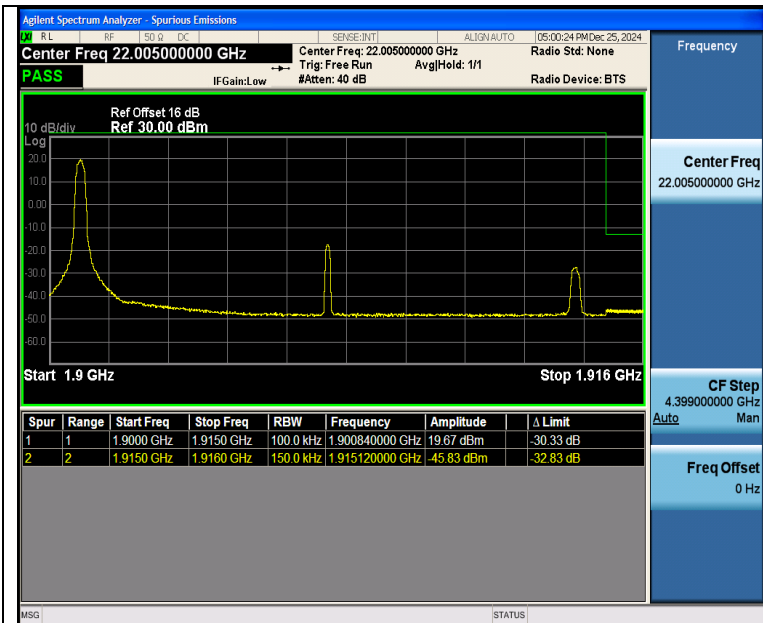
Band25 15MHz 16QAM 26615 1RB#0
