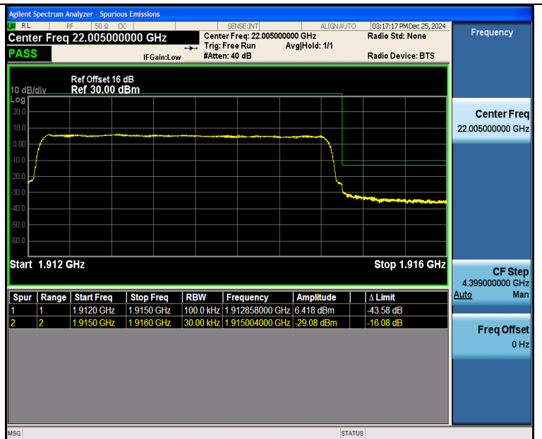
Band25 3MHz QPSK 26675 15RB#0
