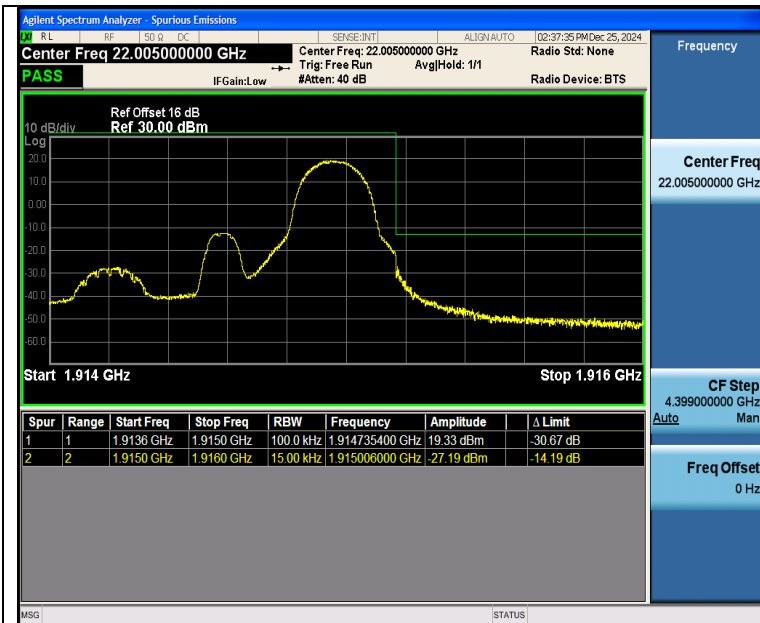
Band25 1.4MHz 16QAM 26683 1RB#5
