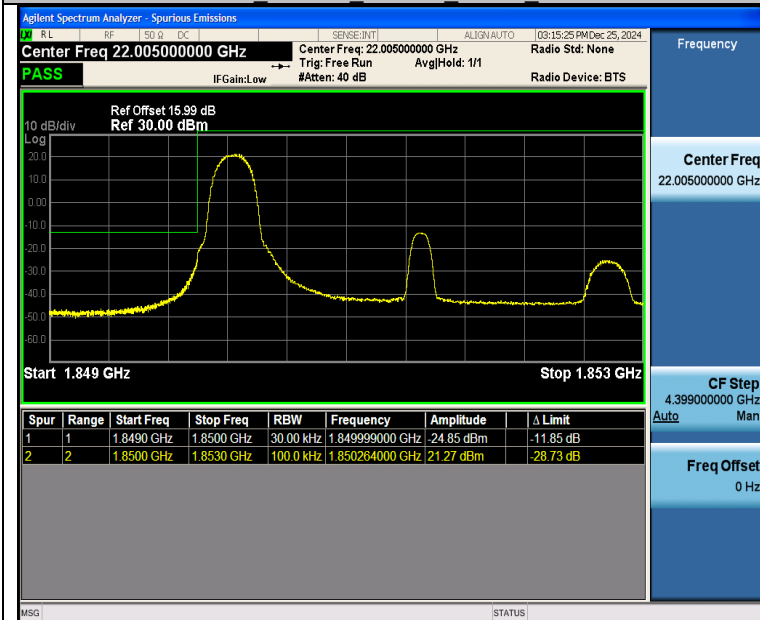
Band25_3MHz_16QAM_26055_1RB#0
