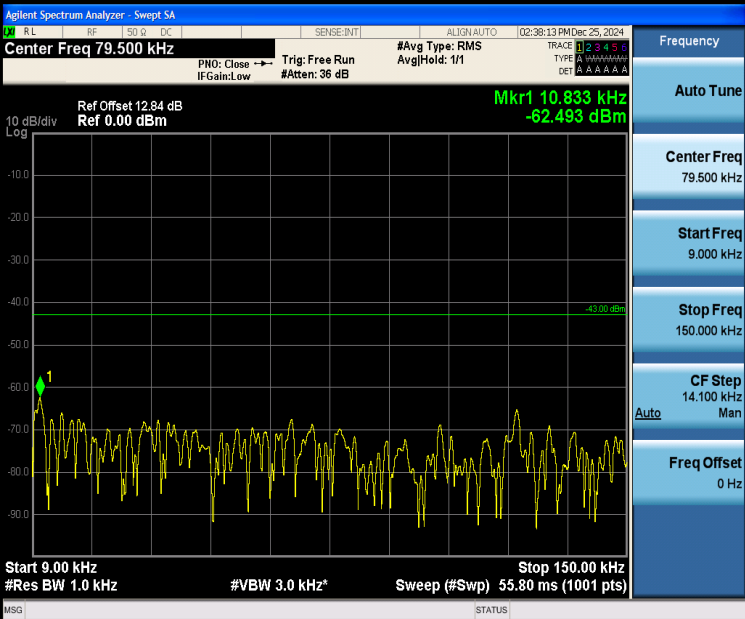
Band25_1.4MHz_QPSK_26047_1RB#0_0.009~0.15_0.009~0.15
