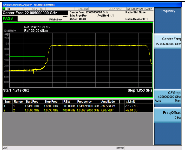
Band25 3MHz QPSK 26055 15RB#0
