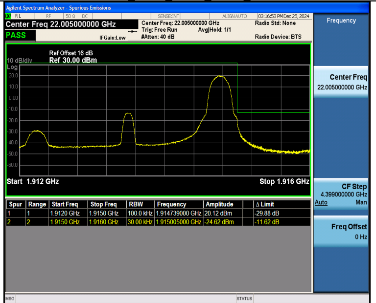
Band25_3MHz_QPSK_26675_1RB#14
