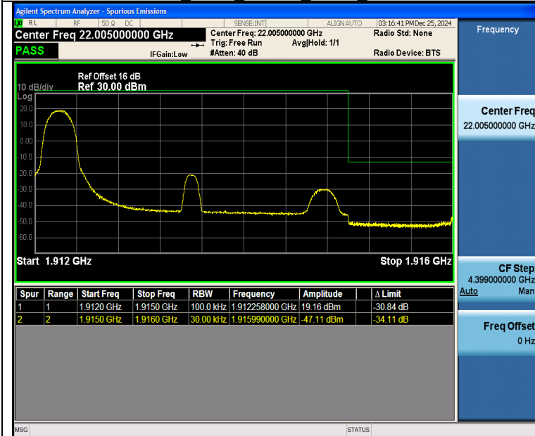
Band25_3MHz_16QAM_26675_1RB#0
