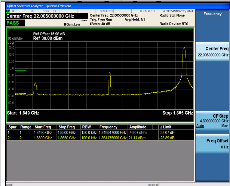
Band25_15MHz_16QAM_26115_1RB#74
