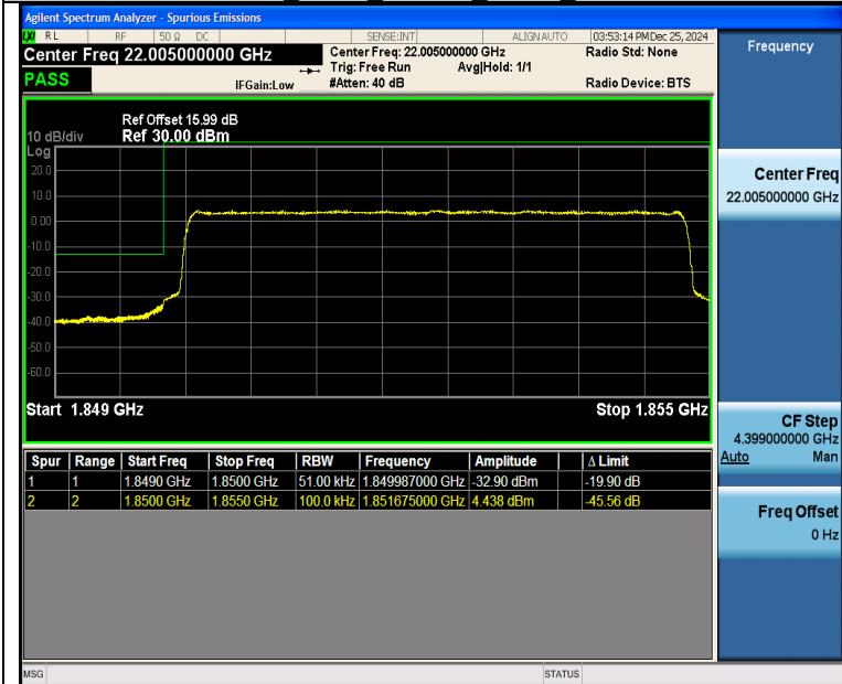
Band25 5MHz 16QAM 26065 25RB#0
