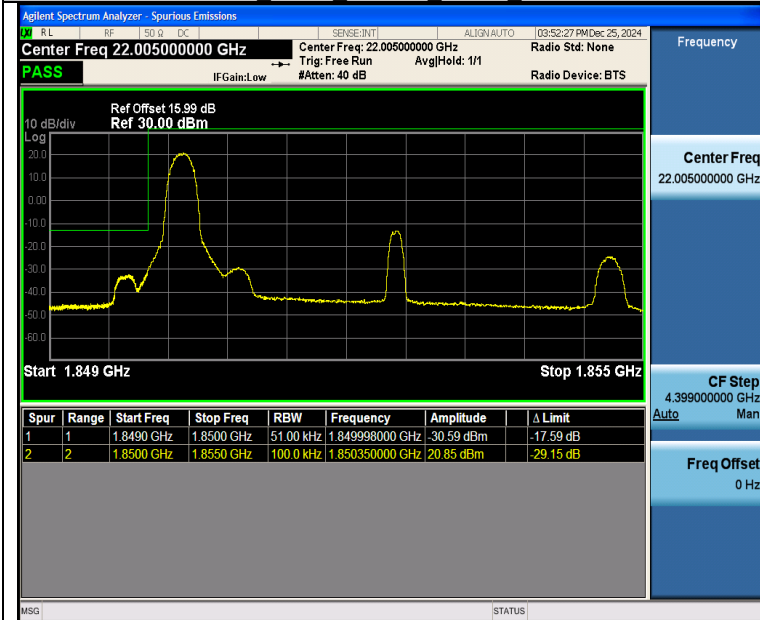
Band25 5MHz 16QAM 26065 1RB#0
