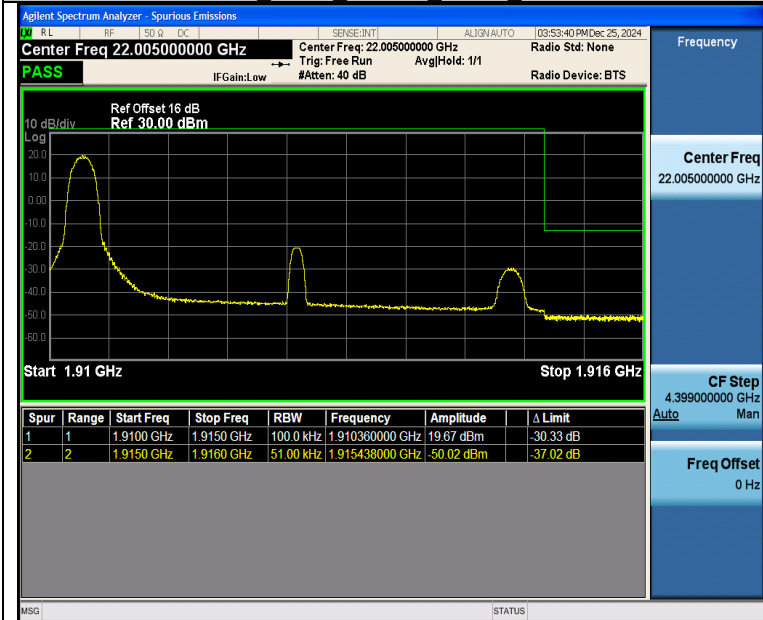
Band25_5MHz_16QAM_26665_1RB#0
