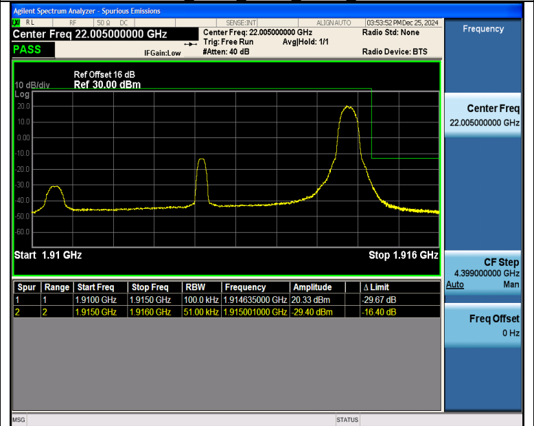
Band25_5MHz_QPSK_26665_1RB#24
