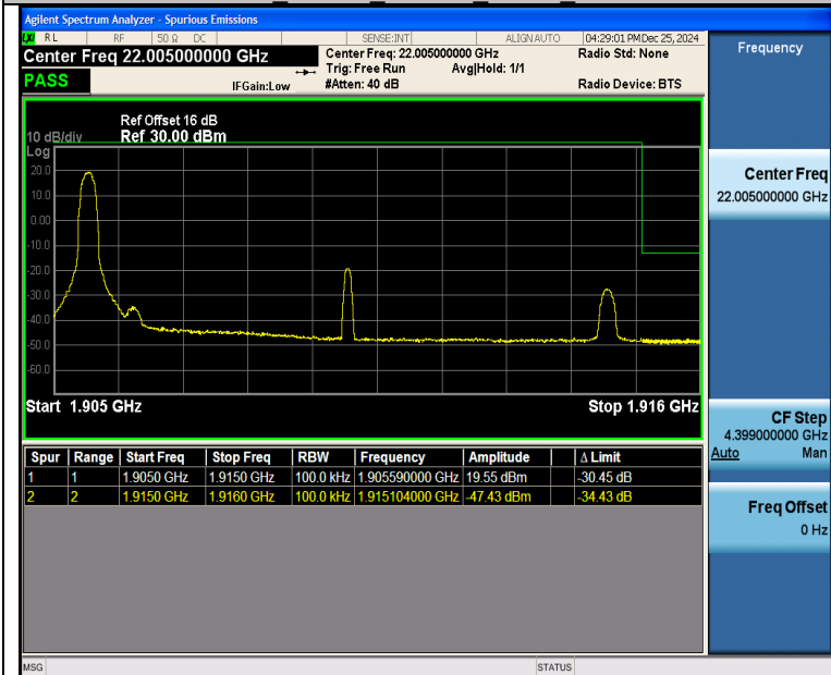
Band25 10MHz 16QAM 26640 1RB#0
