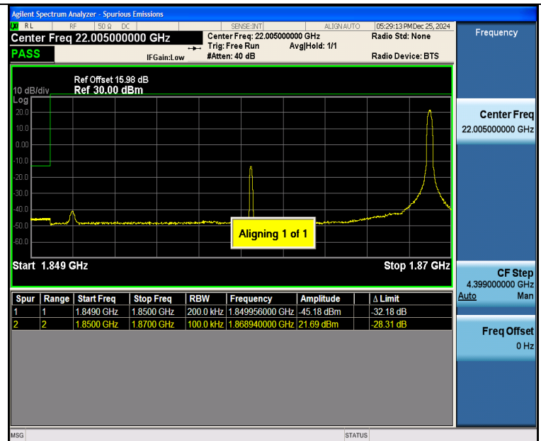
Band25_20MHz_QPSK_26140_1RB#99
