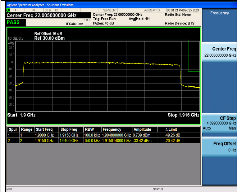
Band25 15MHz_QPSK_26615_75RB#0
