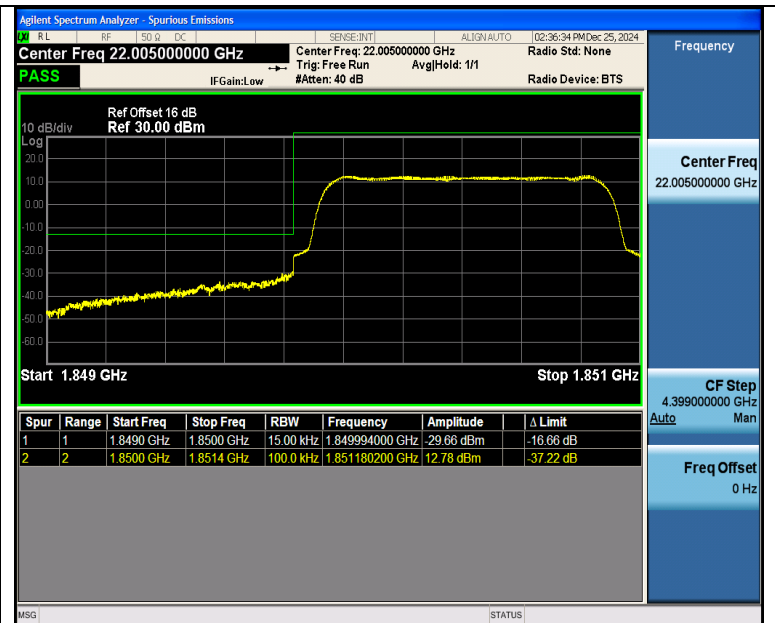
Band25 1.4MHz QPSK 26047 6RB#0
