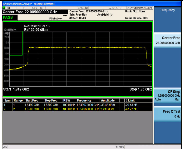
Band25_10MHz_QPSK_26090_50RB#0
