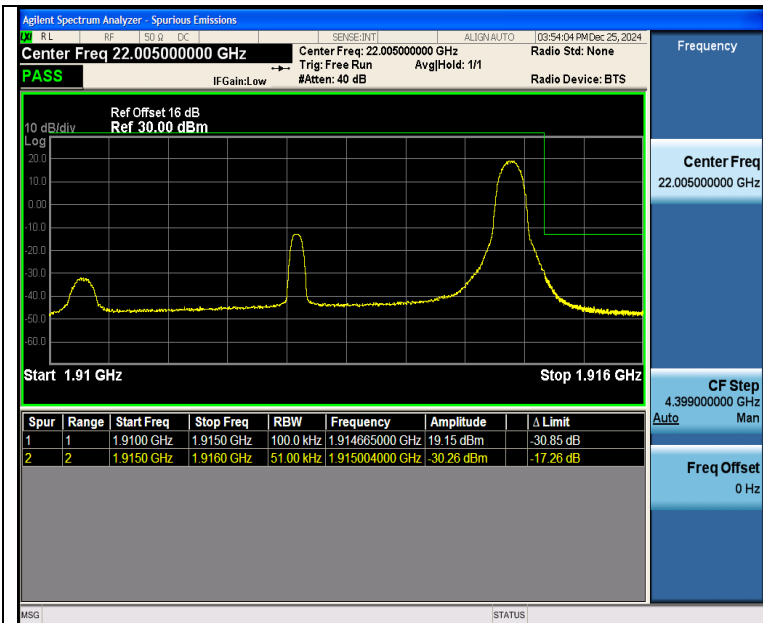
Band25 5MHz 16QAM 26665 1RB#24
