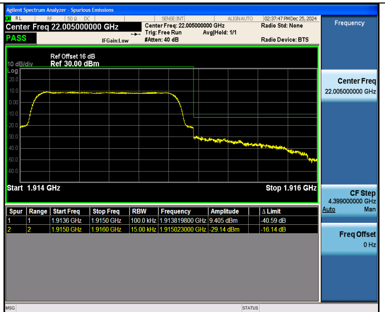
Band25 1.4MHz QPSK 26683 6RB#0
