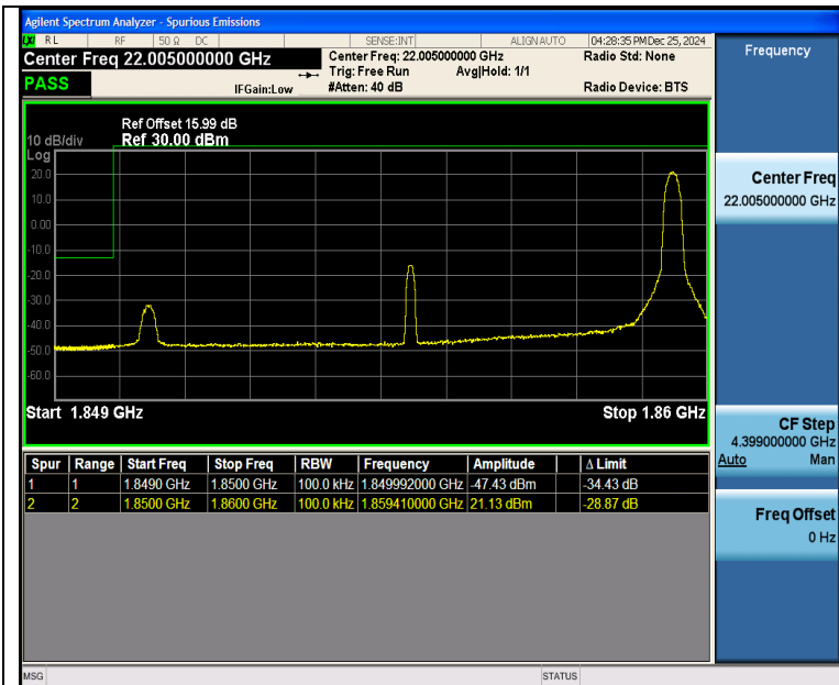
Band25 10MHz 16QAM 26090 1RB#49
