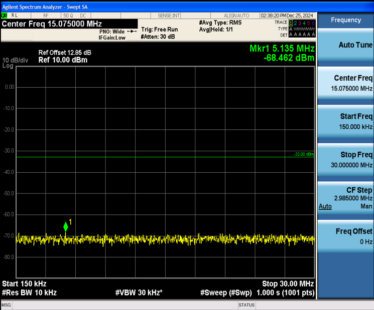
Band25_1.4MHz_QPSK_26047_1RB#0_0.15~30_0.15~30
