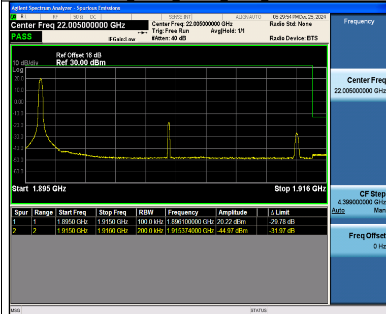
Band25_20MHz_16QAM_26590_1RB#0
