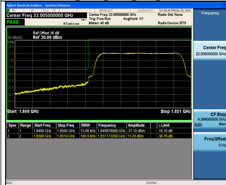
Band25 1.4MHz 16QAM 26047 6RB#0
