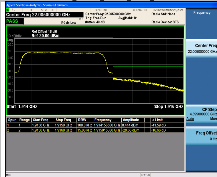
Band25 1.4MHz 16QAM 26683 6RB#0
