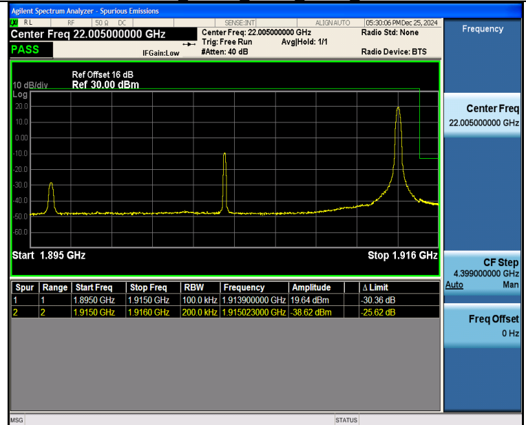
Band25_20MHz_QPSK_26590_1RB#99
