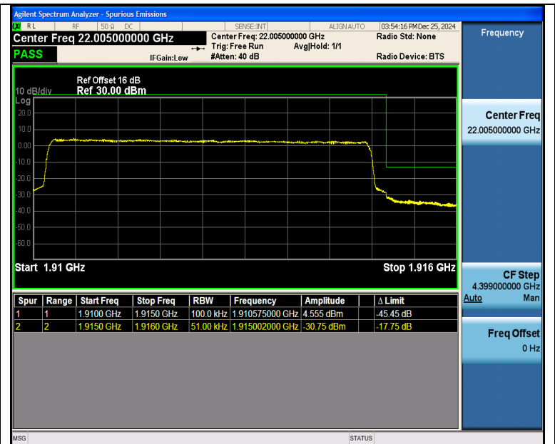
Band25 5MHz QPSK 26665 25RB#0
