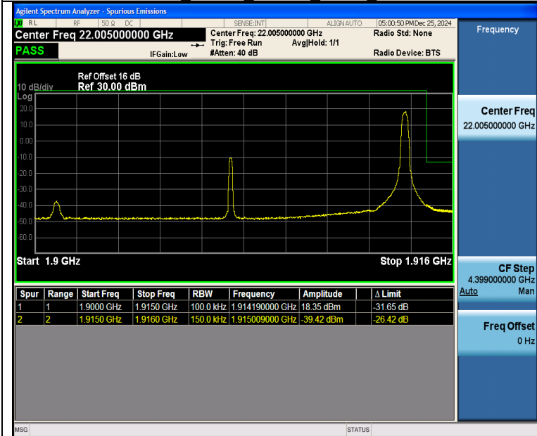
Band25 15MHz 16QAM 26615 1RB#74
