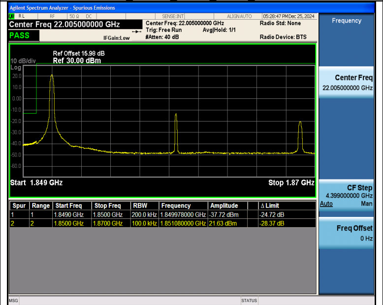
Band25 20MHz_QPSK_26140_1RB#0
