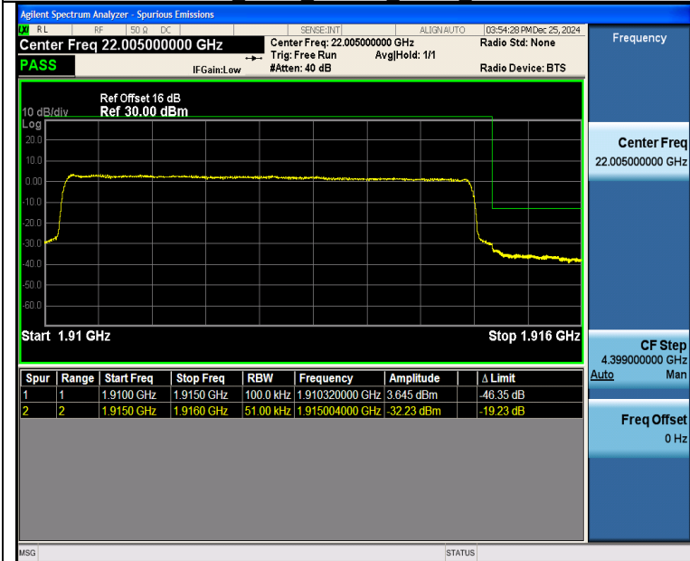
Band25 5MHz 16QAM 26665 25RB#0
