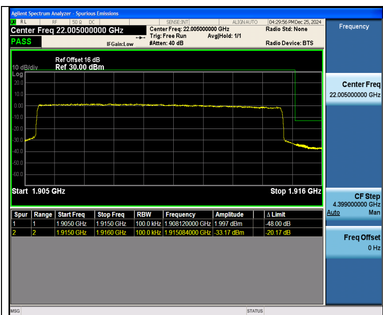
Band25 10MHz QPSK 26640 50RB#0
