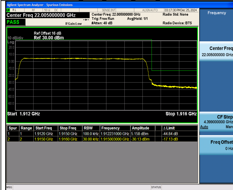
Band25 3MHz 16QAM 26675 15RB#0
