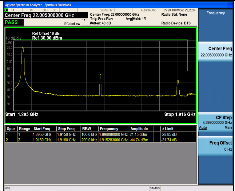
Band25_20MHz_QPSK_26590_1RB#0
