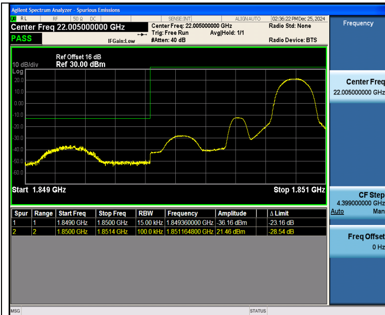
Band25 1.4MHz 16QAM 26047 1RB#5
