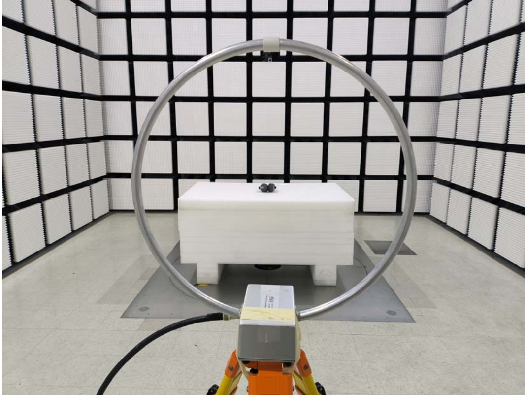
9kHz to 30MHz_Radiated Emission_Perpendicular
