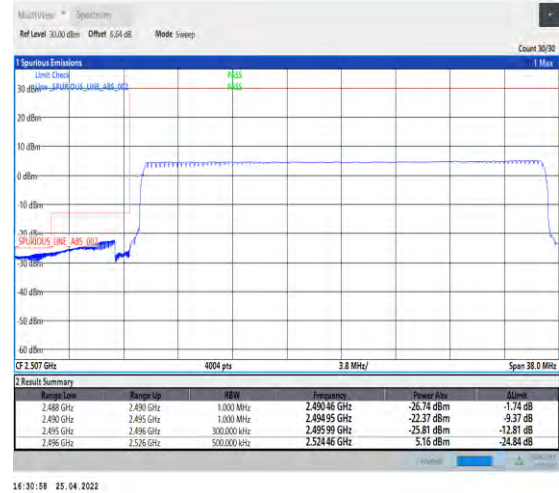
1-N41--30-30-L-6-CP-QPSK-Outer_Full-78@0-An t1-PASS-see graph
