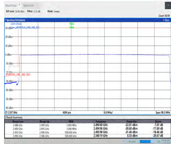
1-N41--30-90-L-6-CP-QPSK-Outer_Full-245@0-Ant 1-PASS-see graph
