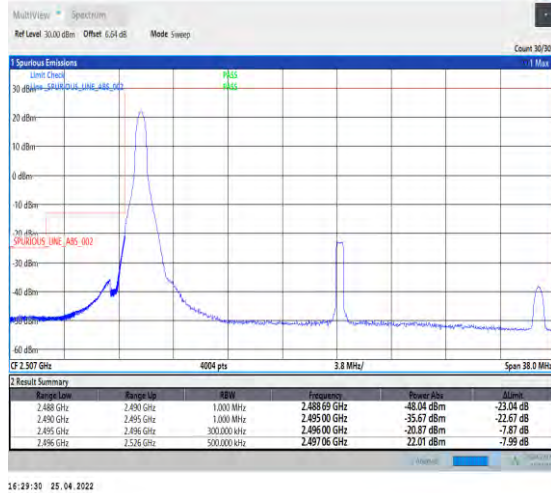
1-N41--30-30-L-4-CP-QPSK-Edge_1RB_Left-1@0-Ant 1-PASS-see graph
