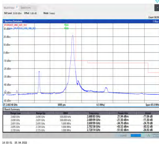
1-N41--30-30-H-5-CP-QPSK-Edge_1RB_Right-1@77- Ant1-PASS-see graph
