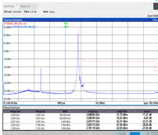
1-N41--30-90-H-5-CP-QPSK-Edge_1RB_Right-1@244-Ant 1-PASS-see graph
