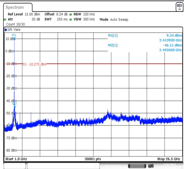
11B-Ant2-2412-1000~26500-PASS
