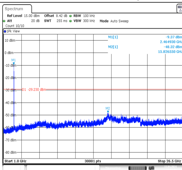
11N20MIMO-Ant2-2462-1000~26500-PASS
