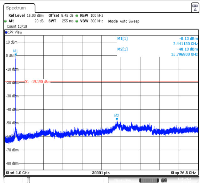
11G-Ant2-2437-1000~26500-PASS
