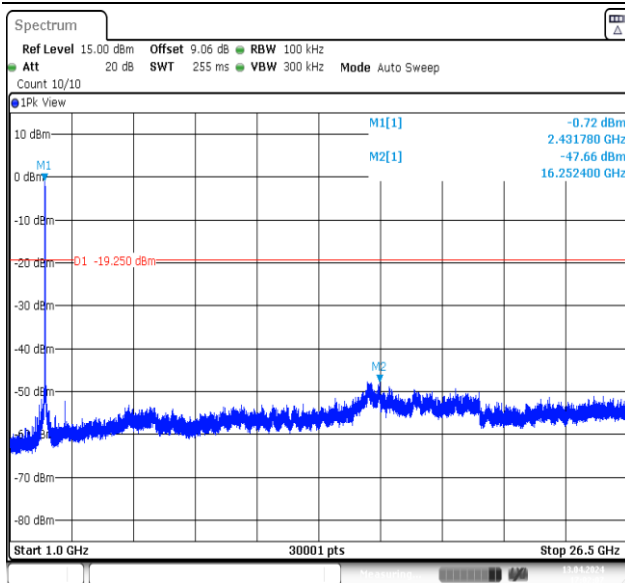
11G-Ant1-2437-1000~26500-PASS
