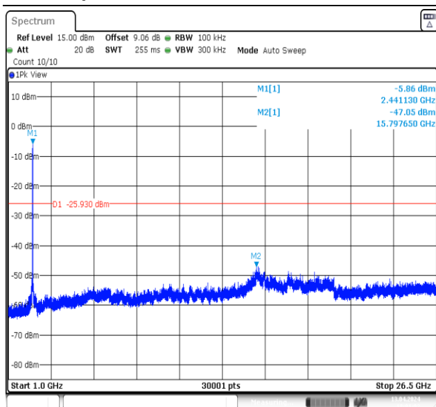
11N40MIMO-Ant1-2437-1000~26500-PASS
