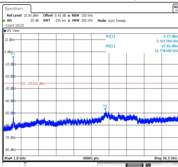
11N40MIMO-Ant2-2437-1000~26500-PASS
