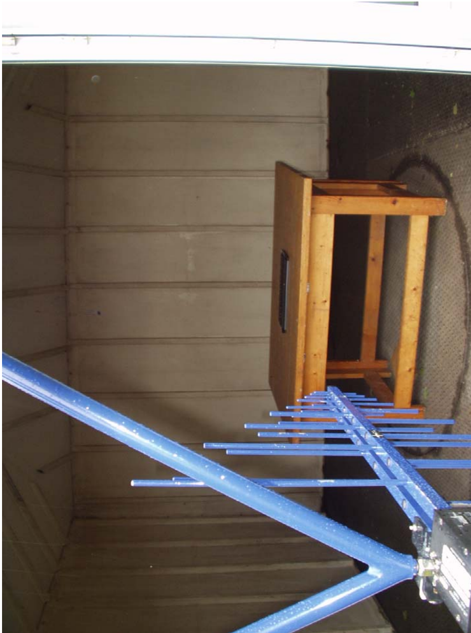
Photograph 2: Test setup OATS > 30 MHz
